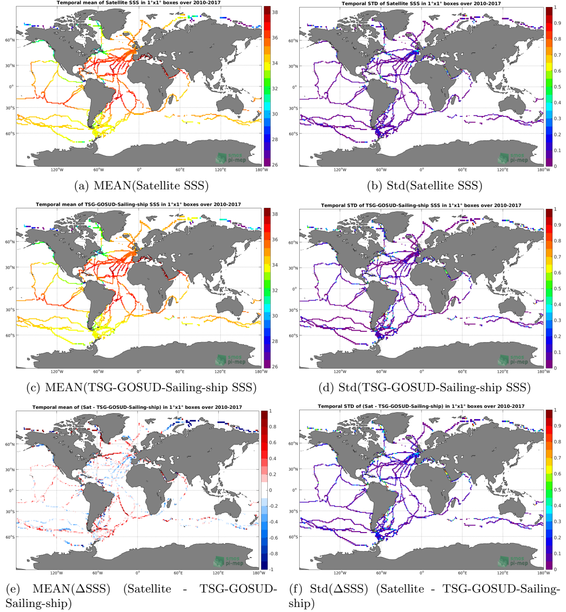
Figure 6: Temporal mean (left) and Std (right) of SSS from SMOS-L3-CATDS-CECOS-LOCEAN-V4-18DAYS-25KM (top), TSG-GOSUD-Sailing-ship (middle), and of \Delta SSS (Satellite - TSG-GOSUD-Sailing-ship). Only match-up pairs are used to generate these maps.
