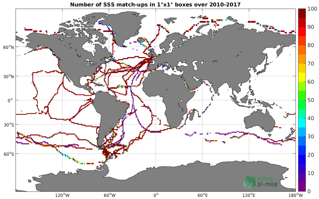
Figure 4: Number of SSS match-ups between TSG-GOSUD-Sailing-ship SSS and the SMOS-L3-CATDS-CECOS-LOCEAN-V4-18DAYS-25KM SSS product for the Global Ocean Pi-MEP region over 1^\circ \times 1^\circ boxes and for the full satellite product period.
