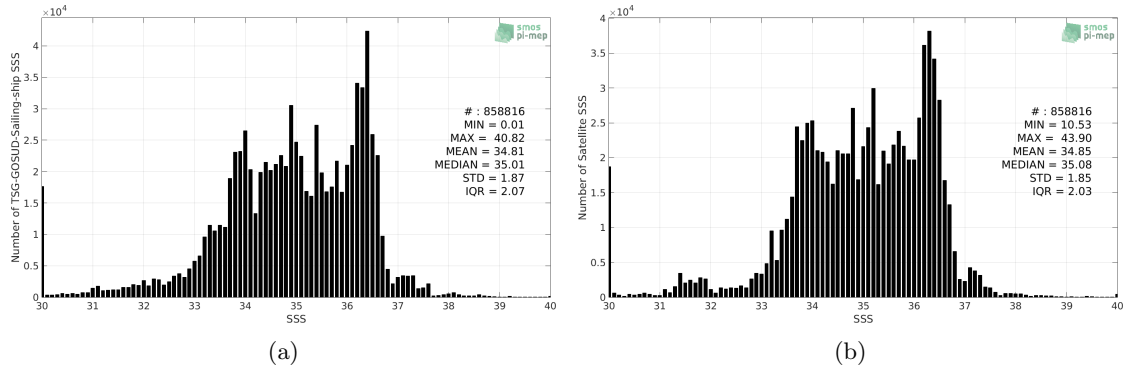
Figure 2: Histograms of SSS from TSG-GOSUD-Sailing-ship (a) and SMOS-L3-CATDS-CECOS-LOCEAN-V4-18DAYS-25KM (b) considering all match-up pairs per bins of 0.1 over the Global Ocean Pi-MEP region and for the full satellite product period.
