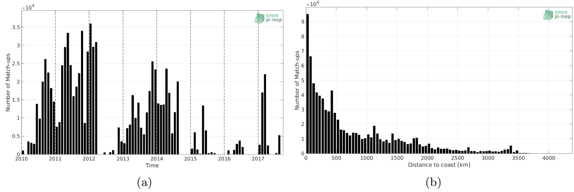
Figure 1: Number of match-ups between TSG-GOSUD-Sailing-ship and SMOS-L3-CATDS-CECOS-LOCEAN-V4-18DAYS-25KM SSS as a function of time (a) and as function of the distance to coast (b) over the Global Ocean Pi-MEP region and for the full satellite product period.
