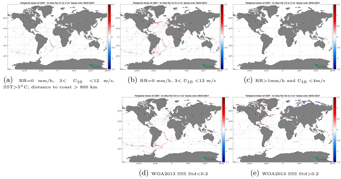
Figure 12: Temporal mean gridded over spatial boxes of size 1^\circ \times 1^\circ of \Delta SSS (SMOS-L3-CATDS-CECOS-LOCEAN-V4-18DAYS-25KM - TSG-GOSUD-Sailing-ship) for 5 different subdatasets corresponding to: RR=0 mm/h, 3 < U_{10} < 12 m/s, SST > 5^\circ C , distance to coast > 800 km (a), RR=0 mm/h, 3 < U_{10} < 12 m/s (b), RR > 1 mm/h and U_{10} < 4 m/s (c), WOA2013 SSS Std < 0.2 (d), WOA2013 SSS Std > 0.2 (e).
