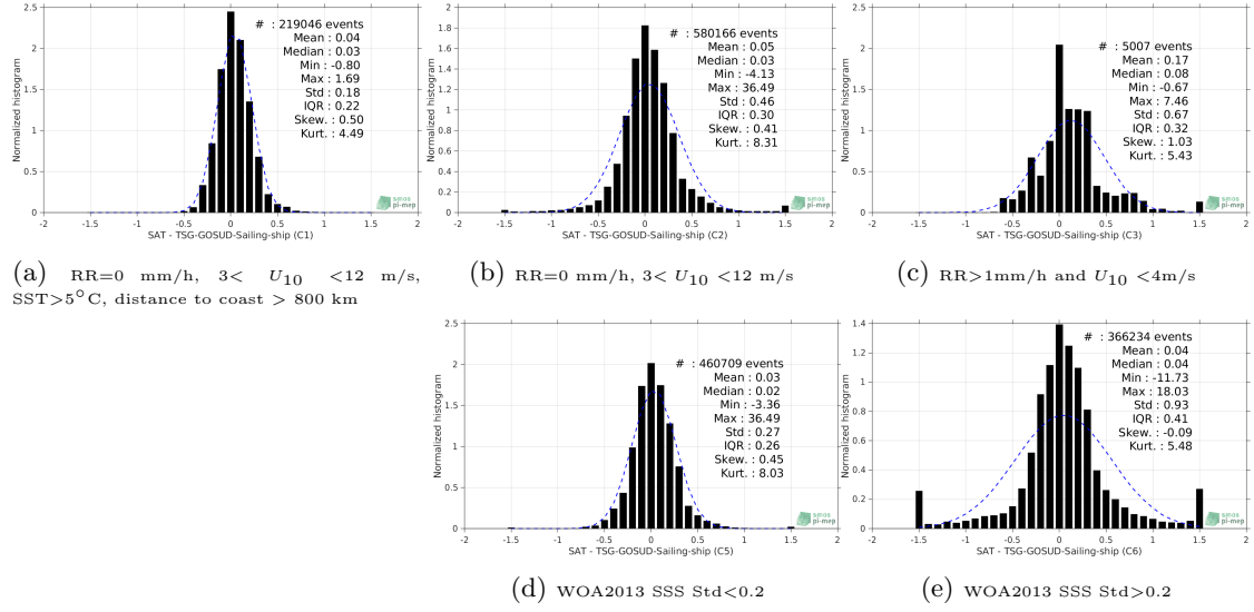
Figure 13: Normalized histogram of \Delta SSS (SMOS-L3-CATDS-CECOS-LOCEAN-V4-18DAYS-25KM - TSG-GOSUD-Sailing-ship) for 5 different subdatasets corresponding to: RR=0 mm/h, 3 < U_{10} < 12 m/s, SST > 5°C, distance to coast > 800 km (a), RR=0 mm/h, 3 < U_{10} < 12 m/s (b), RR > 1 mm/h and U_{10} < 4 m/s (c), WOA2013 SSS Std < 0.2 (d), WOA2013 SSS Std > 0.2 (e).
