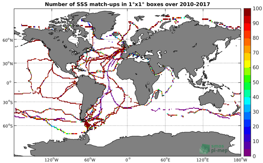
Figure 4: Number of SSS match-ups between TSG-GOSUD-Sailing-ship SSS and the SMOS-L3-CATDS-CECOS-LOCEAN-V4-18DAYS-25KM SSS product for the Global Ocean Pi-MEP region over 1°x1° boxes and for the full satellite product period.
