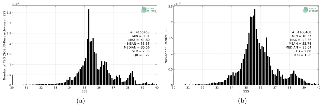
Figure 2: Histograms of SSS from TSG (GOSUD-Research-vessel) (a) and SMOS SSS L3 v4 - 18 Days (CATDS-CECOS-LOCEAN) (b) considering all match-up pairs per bins of 0.1 over the Global Ocean Pi-MEP region and for the full satellite product period.
