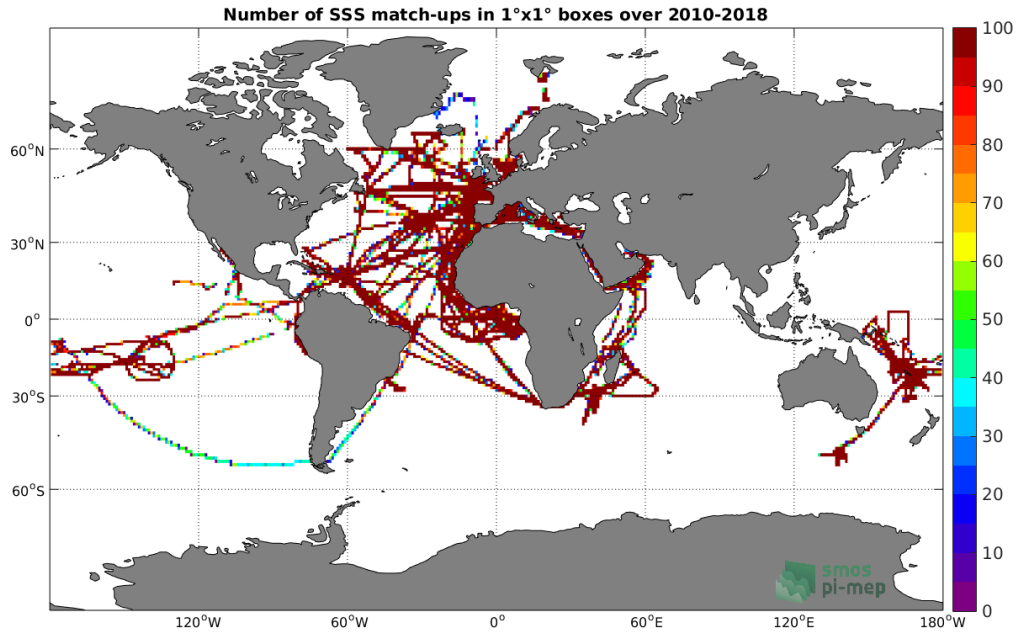
Figure 4: Number of SSS match-ups between TSG (GOSUD-Research-vessel) SSS and the SMOS SSS L3 v4 - 18 Days (CATDS-CECOS-LOCEAN) SSS product for the Global Ocean Pi-MEP region over 1^\circ \times 1^\circ boxes and for the full satellite product period.
