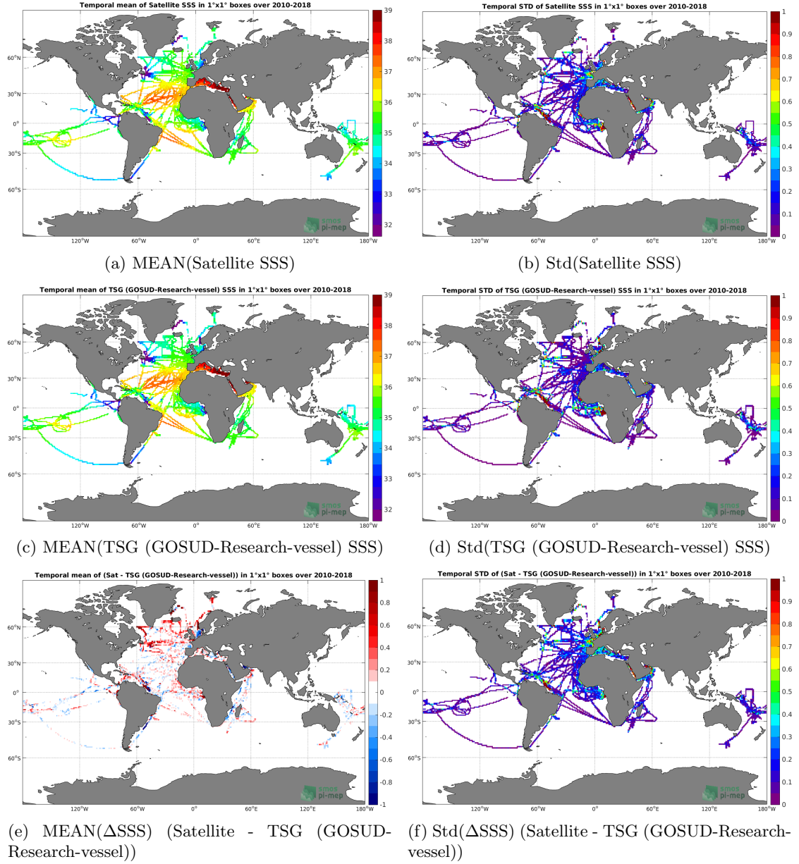
Figure 6: Temporal mean (left) and Std (right) of SSS from SMOS SSS L3 v4 - 18 Days (CATDS-CECOS-LOCEAN) (top), TSG (GOSUD-Research-vessel) (middle), and of \Delta SSS (Satellite - TSG (GOSUD-Research-vessel)). Only match-up pairs are used to generate these maps.
