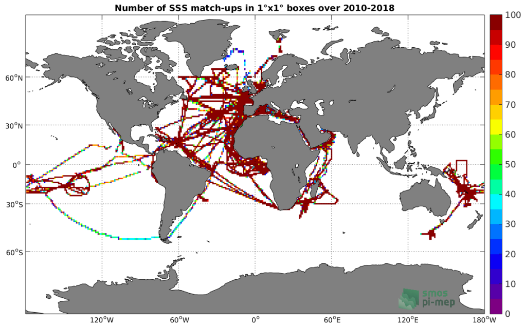
Figure 4: Number of SSS match-ups between TSG-GOSUD-Research-vessel SSS and the SMOS-L3-CATDS-CECOS-LOCEAN-V4-18DAYS-25KM SSS product for the Global Ocean Pi-MEP region over 1^\circ \times 1^\circ boxes and for the full satellite product period.
