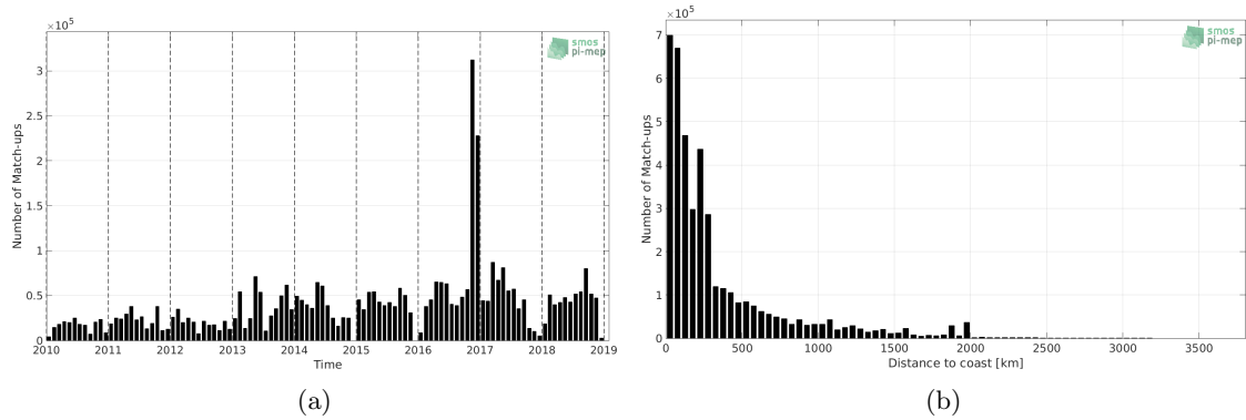
Figure 1: Number of match-ups between TSG-GOSUD-Research-vessel and SMOS-L3-CATDS-CECOS-LOCEAN-V4-18DAYS-25KM SSS as a function of time (a) and as function of the distance to coast (b) over the Global Ocean Pi-MEP region and for the full satellite product period.
