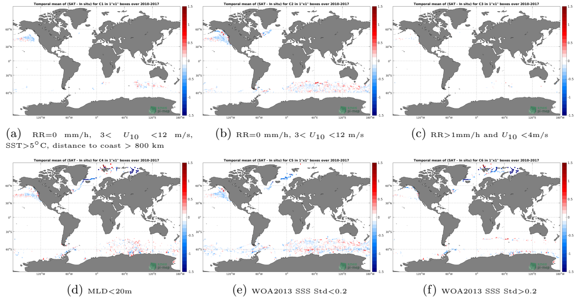
Figure 12: Temporal mean gridded over spatial boxes of size 1^{\circ}\times 1^{\circ} of \Delta\text{SSS} (SMOS-L3-CATDS-CECOS-LOCEAN-V4-18DAYS-25KM - Sea mammals) for 6 different subdatasets corresponding to: RR=0 mm/h, 3 < U_{10} < 12 m/s, SST > 5^{\circ}\text{C} , distance to coast > 800 km (a), RR=0 mm/h, 3 < U_{10} < 12 m/s (b), RR > 1 mm/h and U_{10} < 4 m/s (c), MLD < 20\text{m} (d), WOA2013 SSS Std < 0.2 (e), WOA2013 SSS Std > 0.2 (f).
