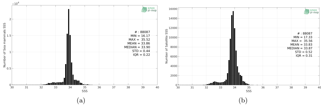
Figure 2: Histograms of SSS from Sea mammals (a) and SMOS-L3-CATDS-CECOS-LOCEAN-V4-18DAYS-25KM (b) considering all match-up pairs per bins of 0.1 over the Global Ocean Pi-MEP region and for the full satellite product period.
