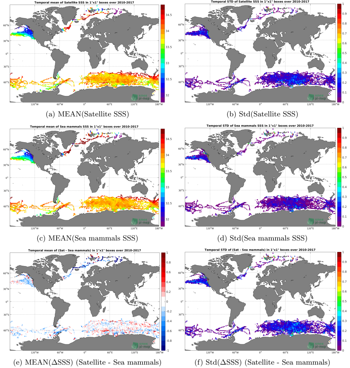
Figure 6: Temporal mean (left) and Std (right) of SSS from SMOS-L3-CATDS-CECOS-LOCEAN-V4-18DAYS-25KM (top), Sea mammals (middle), and of \Delta SSS (Satellite - Sea mammals). Only match-up pairs are used to generate these maps.
