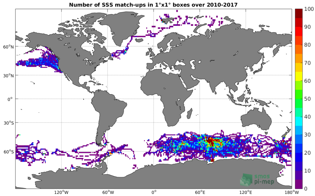
Figure 4: Number of SSS match-ups between Sea mammals SSS and the SMOS-L3-CATDS-CECOS-LOCEAN-V4-18DAYS-25KM SSS product for the Global Ocean Pi-MEP region over 1°x1° boxes and for the full satellite product period.
