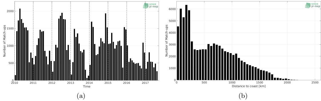
Figure 1: Number of match-ups between Sea mammals and SMOS-L3-CATDS-CECOS-LOCEAN-V4-18DAYS-25KM SSS as a function of time (a) and as function of the distance to coast (b) over the Global Ocean Pi-MEP region and for the full satellite product period.
