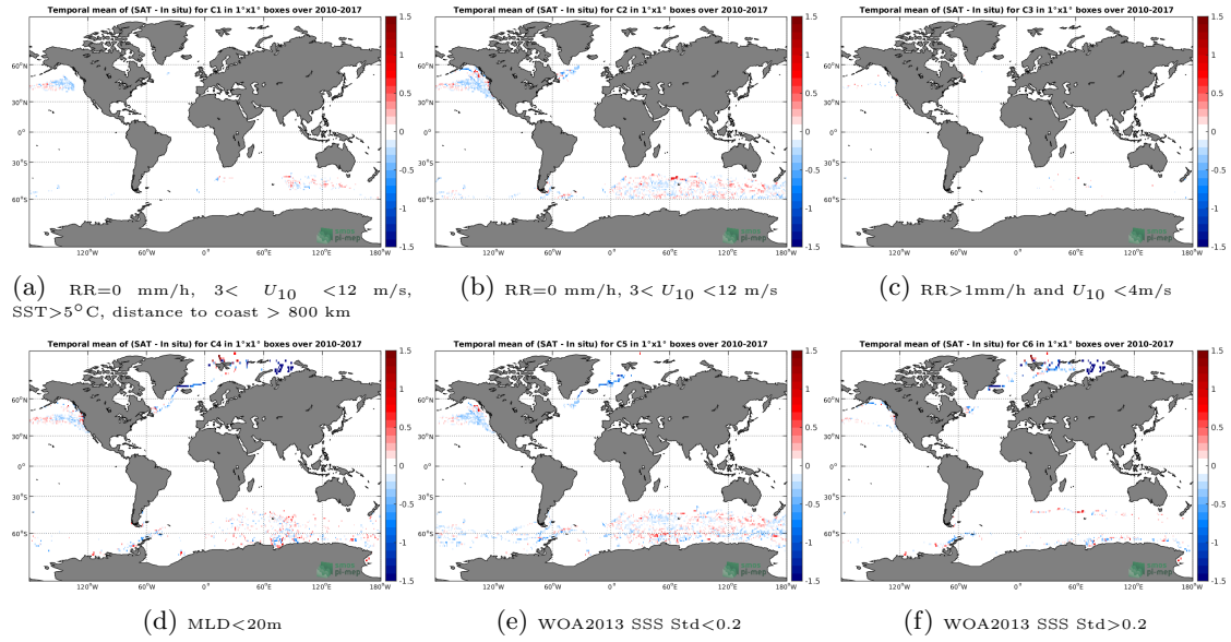
Figure 12: Temporal mean gridded over spatial boxes of size 1^\circ \times 1^\circ of \Delta SSS (SMOS-L3-CATDS-CECOS-LOCEAN-V4-18DAYS-25KM - Sea mammals) for 6 different subdatasets corresponding to: RR=0 mm/h, 3 < U_{10} < 12 m/s, SST > 5^\circ C , distance to coast > 800 km (a), RR=0 mm/h, 3 < U_{10} < 12 m/s (b), RR > 1 mm/h and U_{10} < 4 m/s (c), MLD < 20 m (d), WOA2013 SSS Std < 0.2 (e), WOA2013 SSS Std > 0.2 (f).
