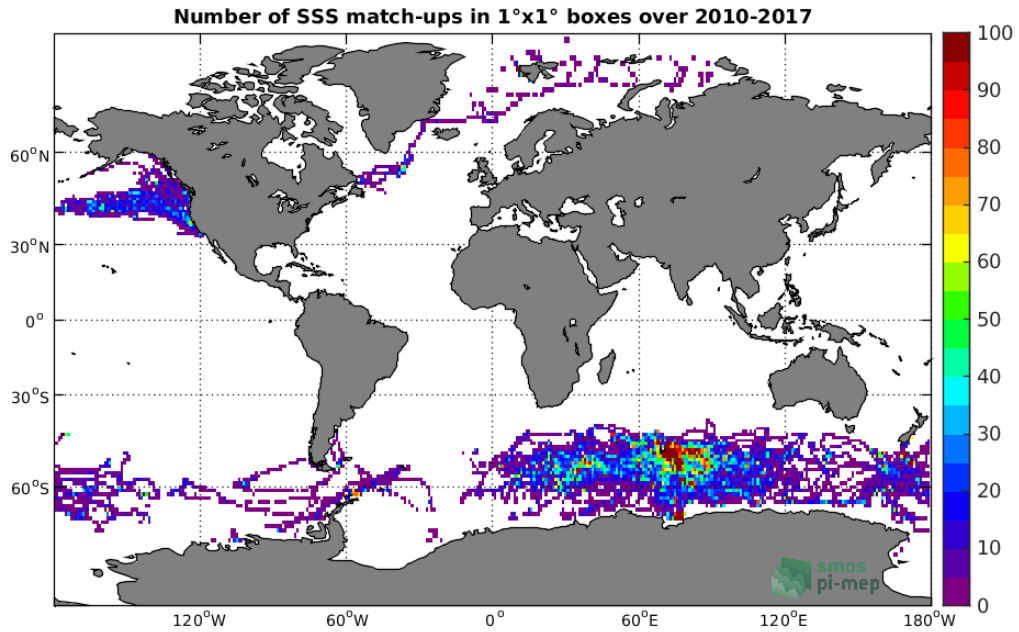
Figure 4: Number of SSS match-ups between Sea mammals SSS and the SMOS-L3-CATDS-CECOS-LOCEAN-V4-18DAYS-25KM SSS product for the Global Ocean Pi-MEP region over 1°x1° boxes and for the full satellite product period.
