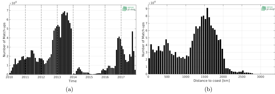
Figure 1: Number of match-ups between Surface drifters and SMOS-L3-CATDS-CECOS-LOCEAN-V4-18DAYS-25KM SSS as a function of time (a) and as function of the distance to coast (b) over the Global Ocean Pi-MEP region and for the full satellite product period.
