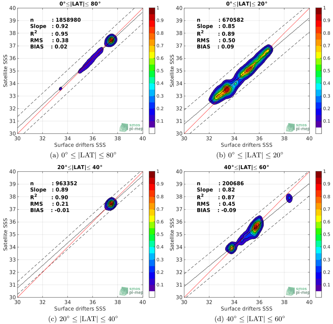
Figure 8: Contour maps of the concentration of SMOS-L3-CATDS-CECOS-LOCEAN-V4-18DAYS-25KM SSS (y-axis) versus Surface drifters SSS (x-axis) at match-up pairs for different latitude bands. For each plot, the red line shows x=y . The black thin and dashed lines indicate a linear fit through the data cloud and the \pm 95\% confidence levels, respectively. The number match-up pairs n , the slope and R^2 coefficient of the linear fit, the root mean square (RMS) and the mean bias between satellite and in situ data are indicated for each latitude band in each plots.
