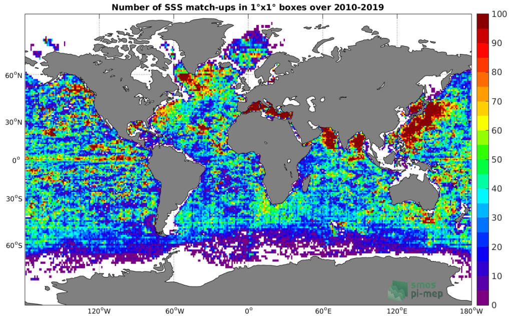
Figure 4: Number of SSS match-ups between Argo SSS and the SMOS-L3-CATDS-CECOS-LOCEAN-V4-18DAYS-25KM SSS product for the Global Ocean Pi-MEP region over 1°x1° boxes and for the full satellite product period.
