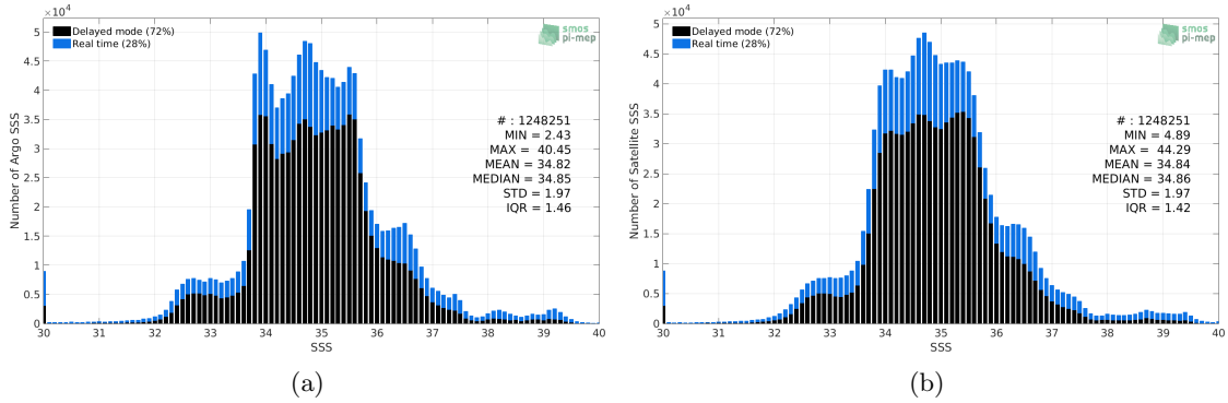
Figure 2: Histograms of SSS from Argo (a) and SMOS-L3-CATDS-CECOS-LOCEAN-V4-18DAYS-25KM (b) considering all match-up pairs per bins of 0.1 over the Global Ocean Pi-MEP region and for the full satellite product period.
