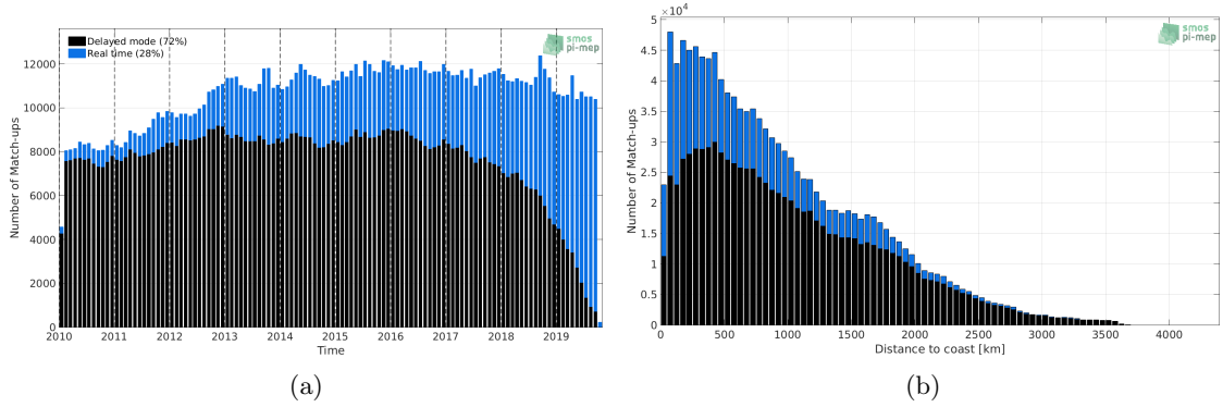
Figure 1: Number of match-ups between Argo and SMOS-L3-CATDS-CECOS-LOCEAN-V4-18DAYS-25KM SSS as a function of time (a) and as function of the distance to coast (b) over the Global Ocean Pi-MEP region and for the full satellite product period.
