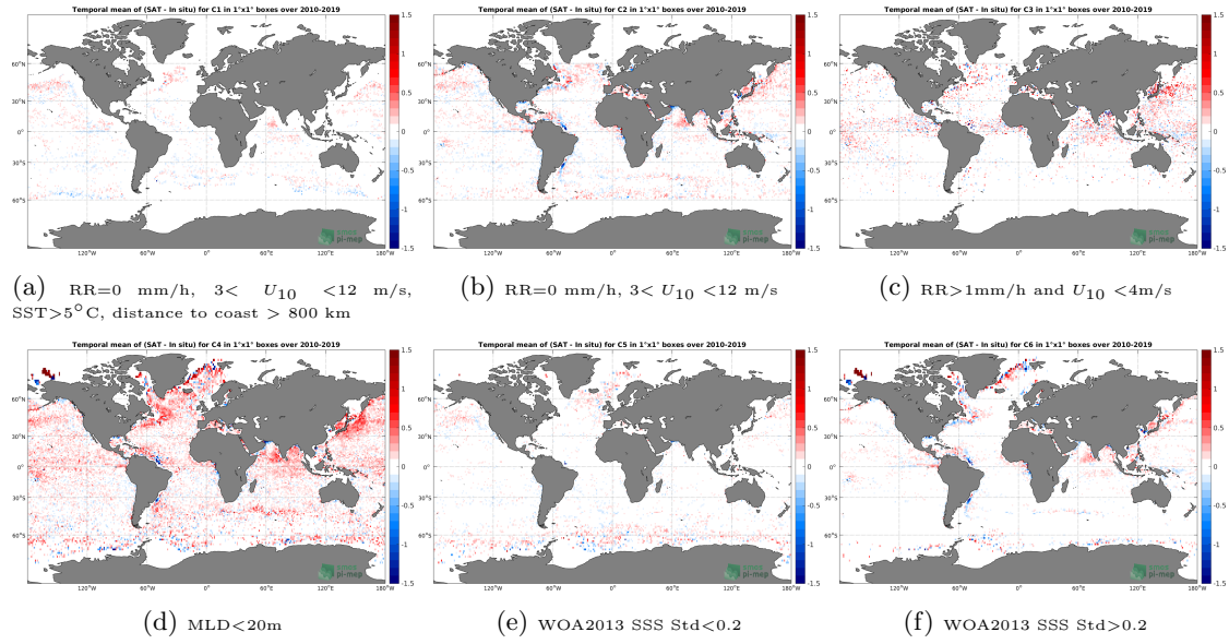
Figure 12: Temporal mean gridded over spatial boxes of size 1^\circ \times 1^\circ of \Delta SSS (SMOS-L3-CATDS-CECOS-LOCEAN-V4-18DAYS-25KM - Argo) for 6 different subdatasets corresponding to: RR=0 mm/h, 3 < U_{10} < 12 m/s, SST > 5^\circ C , distance to coast > 800 km (a), RR=0 mm/h, 3 < U_{10} < 12 m/s (b), RR > 1 mm/h and U_{10} < 4 m/s (c), MLD < 20 m (d), WOA2013 SSS Std < 0.2 (e), WOA2013 SSS Std > 0.2 (f).
