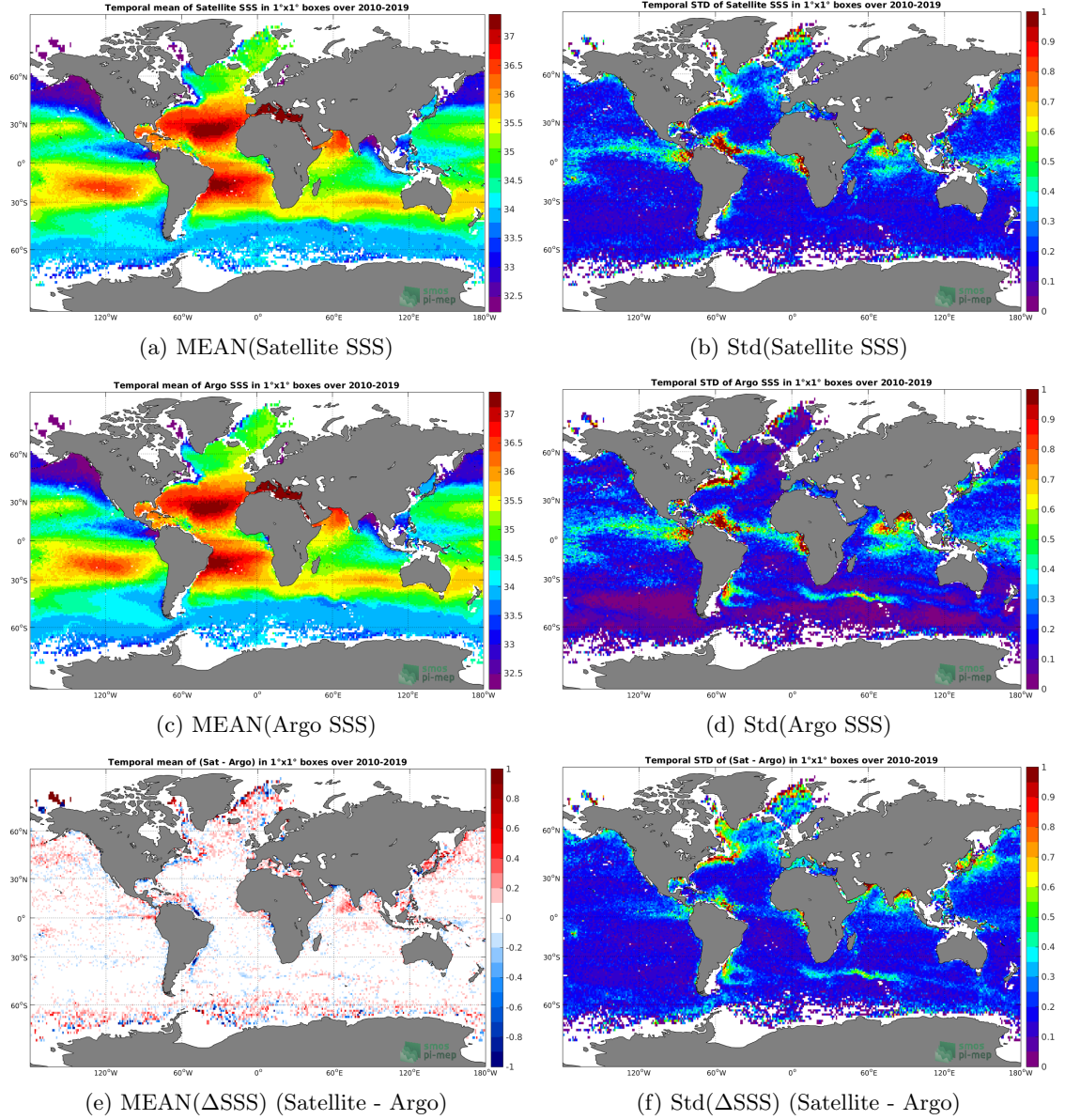
Figure 6: Temporal mean (left) and Std (right) of SSS from SMOS-L3-CATDS-CECOS-LOCEAN-V4-18DAYS-25KM (top), Argo (middle), and of \Delta SSS (Satellite - Argo). Only match-up pairs are used to generate these maps.
