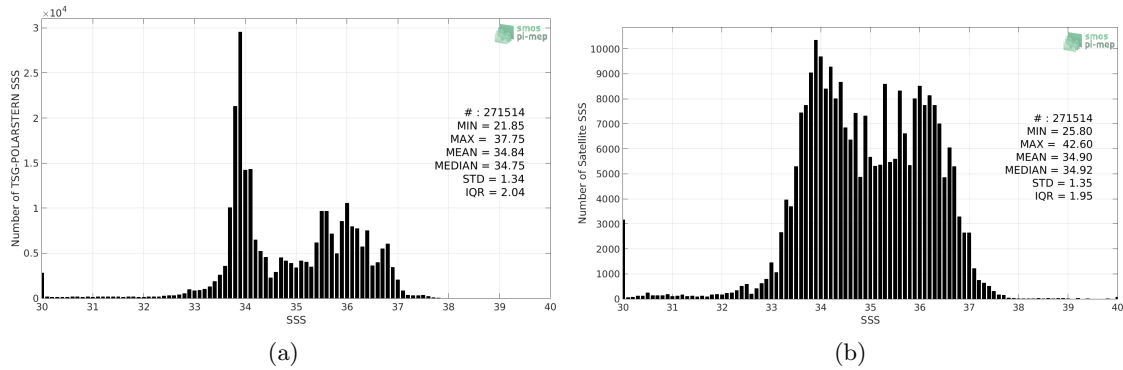
Figure 2: Histograms of SSS from TSG-POLARSTERN (a) and SMOS-L3-CATDS-CECOS-LOCEAN-V3-9DAYS-25KM (b) considering all match-up pairs per bins of 0.1 over the Global Ocean Pi-MEP region and for the full satellite product period.
