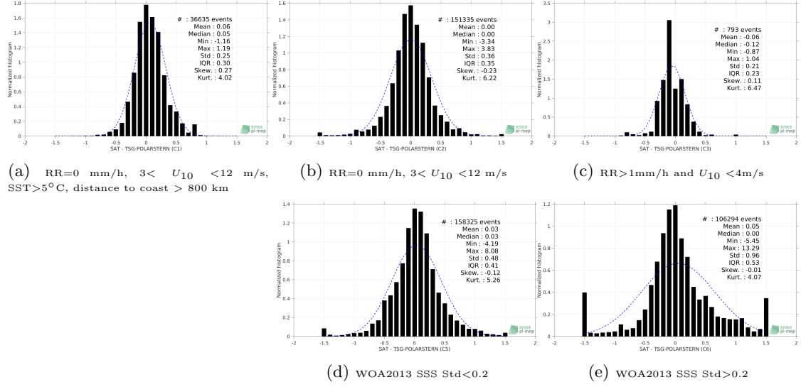
Figure 13: Normalized histogram of \Delta SSS (SMOS-L3-CATDS-CECOS-LOCEAN-V3-9DAYS-25KM - TSG-POLARSTERN) for 5 different subdatasets corresponding to: RR=0 mm/h, 3 < U_{10} < 12 m/s, SST > 5°C, distance to coast > 800 km (a), RR=0 mm/h, 3 < U_{10} < 12 m/s (b), RR > 1mm/h and U_{10} < 4 m/s (c), WOA2013 SSS Std < 0.2 (d), WOA2013 SSS Std > 0.2 (e).
