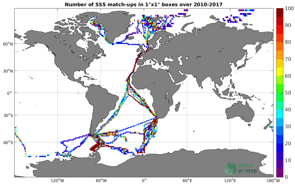
Figure 4: Number of SSS match-ups between TSG-POLARSTERN SSS and the SMOS-L3-CATDS-CECOS-LOCEAN-V3-9DAYS-25KM SSS product for the Global Ocean Pi-MEP region over 1^\circ \times 1^\circ boxes and for the full satellite product period.
