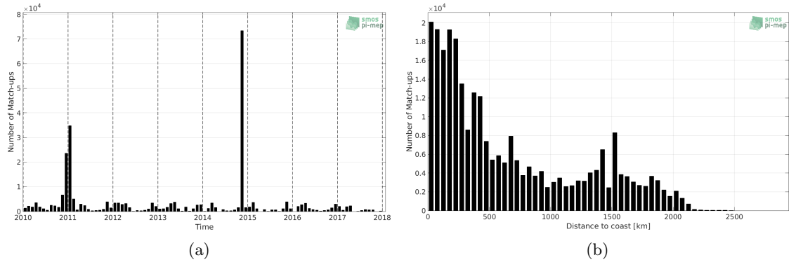
Figure 1: Number of match-ups between TSG-POLARSTERN and SMOS-L3-CATDS-CECOS-LOCEAN-V3-9DAYS-25KM SSS as a function of time (a) and as function of the distance to coast (b) over the Global Ocean Pi-MEP region and for the full satellite product period.
