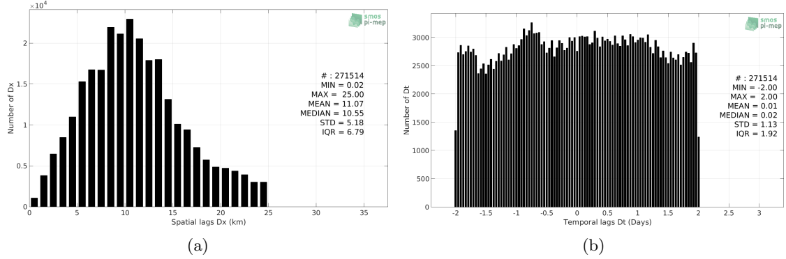
Figure 5: Histograms of the spatial (a) and temporal (b) lags between the time of the TSG-POLARSTERN measurements and the date of the corresponding SMOS-L3-CATDS-CECOS-LOCEAN-V3-9DAYS-25KM SSS product.
