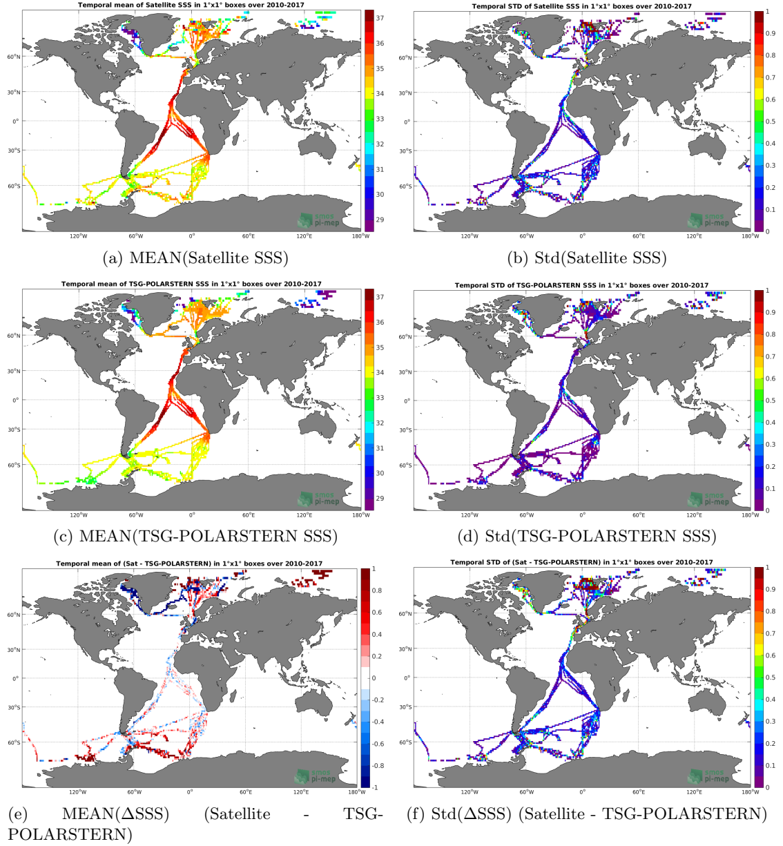
Figure 6: Temporal mean (left) and Std (right) of SSS from SMOS-L3-CATDS-CECOS-LOCEAN-V3-9DAYS-25KM (top), TSG-POLARSTERN (middle), and of \Delta SSS (Satellite - TSG-POLARSTERN). Only match-up pairs are used to generate these maps.
