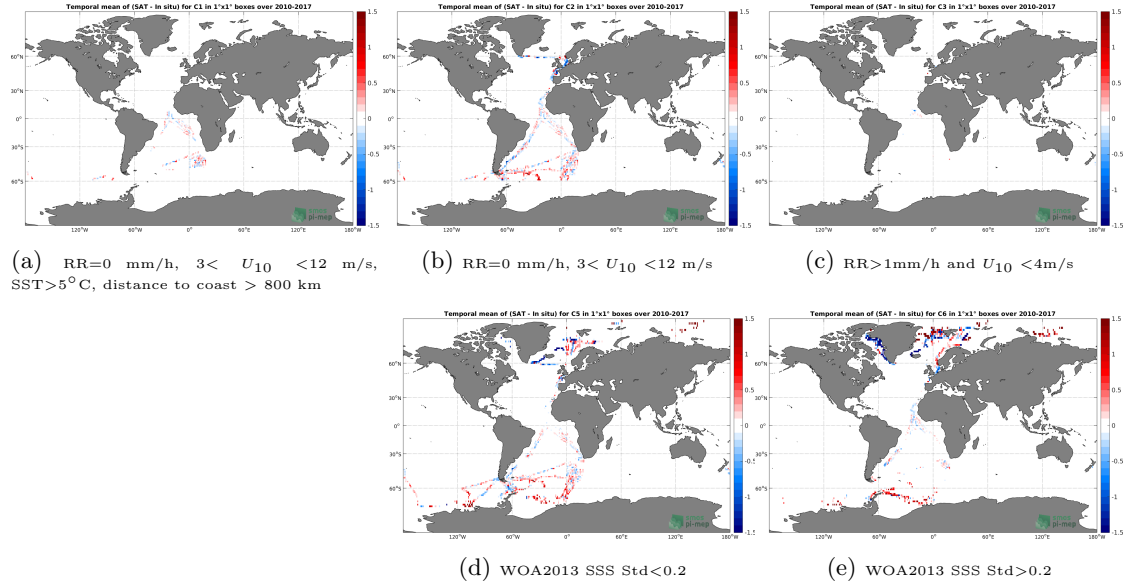
Figure 12: Temporal mean gridded over spatial boxes of size 1^\circ \times 1^\circ of \Delta SSS (SMOS-L3-CATDS-CECOS-LOCEAN-V3-9DAYS-25KM - TSG-POLARSTERN) for 5 different subdatasets corresponding to: RR=0 mm/h, 3 < U_{10} < 12 m/s, SST >5^\circ C, distance to coast > 800 km (a), RR=0 mm/h, 3 < U_{10} < 12 m/s (b), RR >1 mm/h and U_{10} < 4 m/s (c), WOA2013 SSS Std <0.2 (d), WOA2013 SSS Std >0.2 (e).
