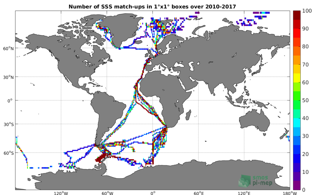
Figure 4: Number of SSS match-ups between TSG-POLARSTERN SSS and the SMOS-L3-CATDS-CECOS-LOCEAN-V3-9DAYS-25KM SSS product for the Global Ocean Pi-MEP region over 1°x1° boxes and for the full satellite product period.
