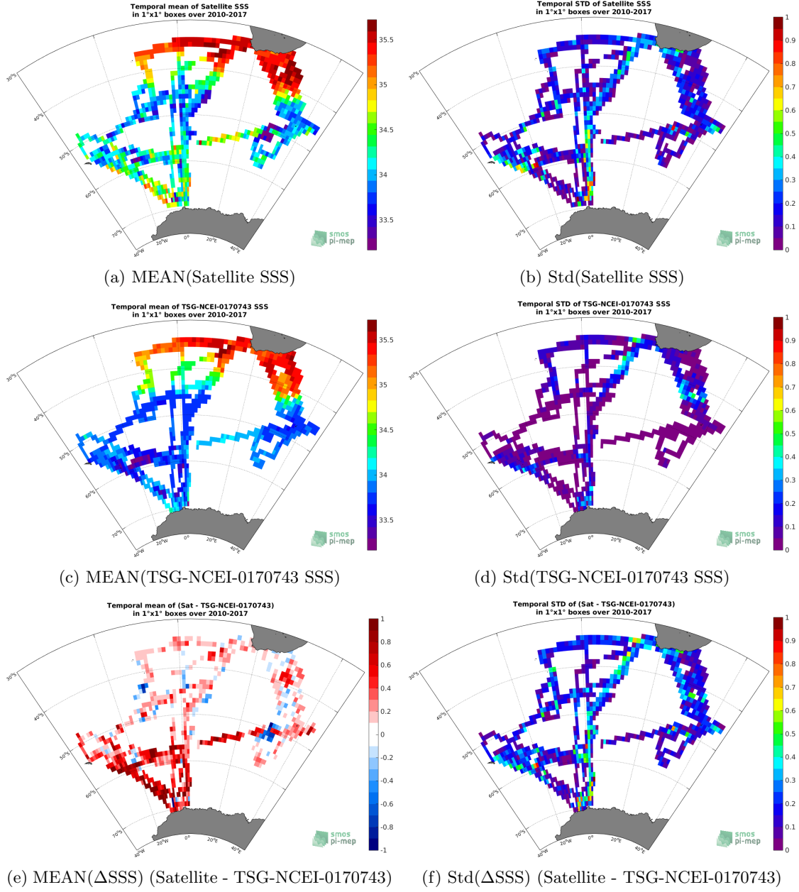
Figure 6: Temporal mean (left) and Std (right) of SSS from SMOS-L3-CATDS-CECOS-LOCEAN-V3-9DAYS-25KM (top), TSG-NCEI-0170743 (middle), and of \Delta SSS (Satellite - TSG-NCEI-0170743). Only match-up pairs are used to generate these maps.
