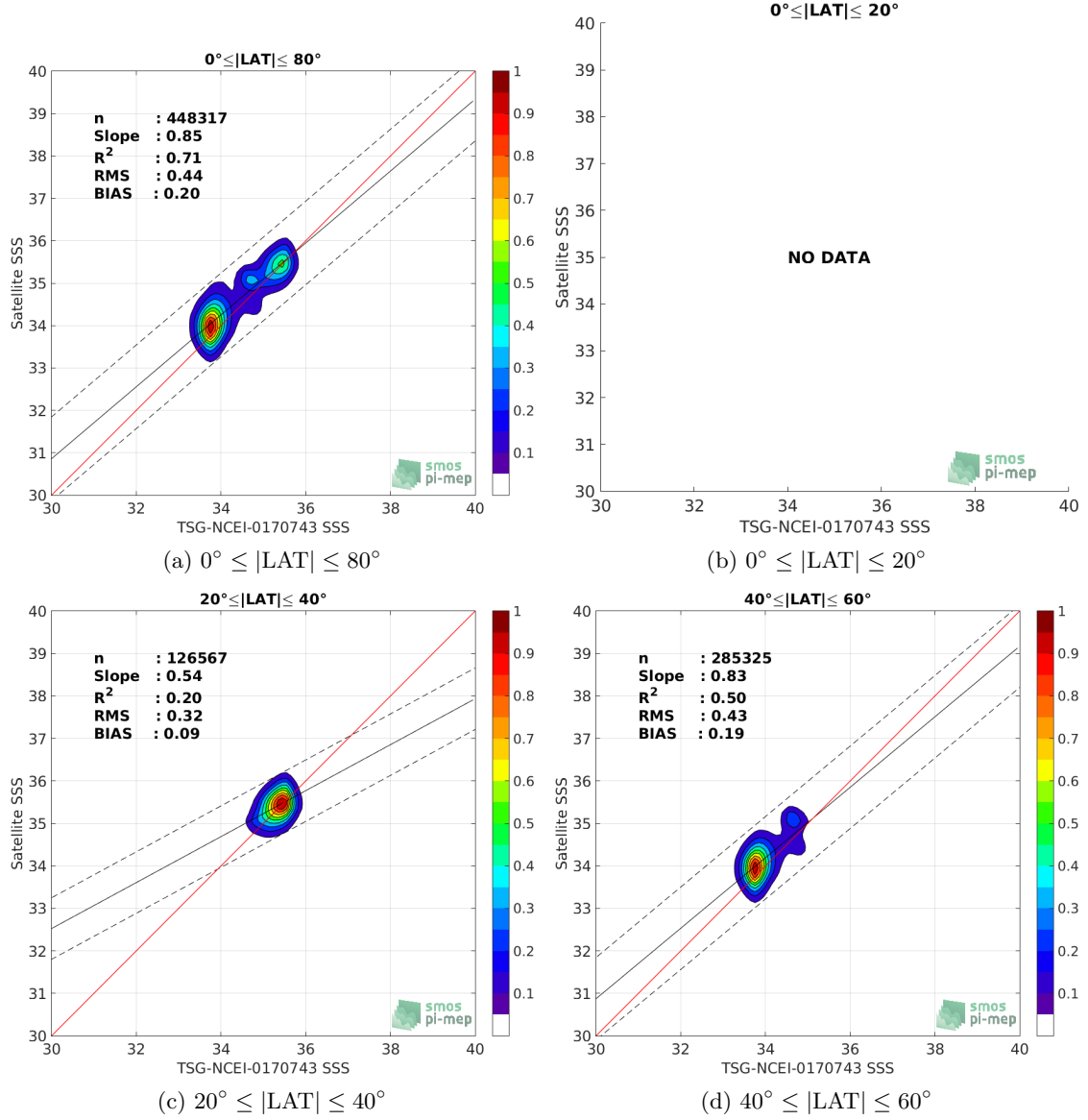
Figure 9: Contour maps of the concentration of SMOS-L3-CATDS-CECOS-LOCEAN-V3-9DAYS-25KM SSS (y-axis) versus TSG-NCEI-0170743 SSS (x-axis) at match-up pairs for different latitude bands. For each plot, the red line shows x=y . The black thin and dashed lines indicate a linear fit through the data cloud and the \pm 95\% confidence levels, respectively. The number match-up pairs n , the slope and R^2 coefficient of the linear fit, the root mean square (RMS) and the mean bias between satellite and in situ data are indicated for each latitude band in each plots.
