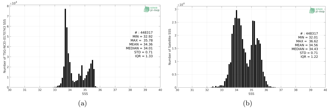
Figure 2: Histograms of SSS from TSG-NCEI-0170743 (a) and SMOS-L3-CATDS-CECOS-LOCEAN-V3-9DAYS-25KM (b) considering all match-up pairs per bins of 0.1 over the Global Ocean Pi-MEP region and for the full satellite product period.
