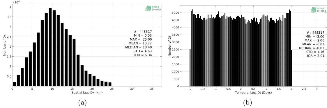
Figure 5: Histograms of the spatial (a) and temporal (b) lags between the time of the TSG-NCEI-0170743 measurements and the date of the corresponding SMOS-L3-CATDS-CECOS-LOCEAN-V3-9DAYS-25KM SSS product.
