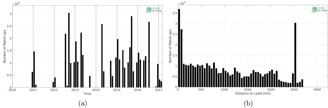
Figure 1: Number of match-ups between TSG-NCEI-0170743 and SMOS-L3-CATDS-CECOS-LOCEAN-V3-9DAYS-25KM SSS as a function of time (a) and as function of the distance to coast (b) over the Global Ocean Pi-MEP region and for the full satellite product period.
