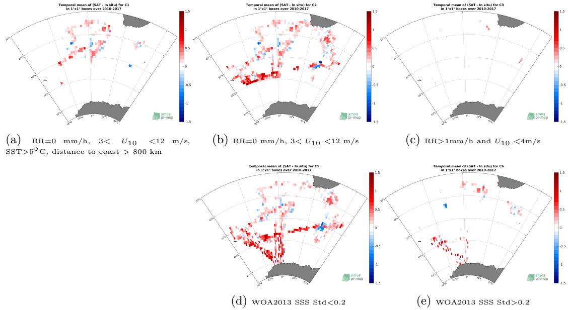
Figure 12: Temporal mean gridded over spatial boxes of size 1^\circ \times 1^\circ of \Delta SSS (SMOS-L3-CATDS-CECOS-LOCEAN-V3-9DAYS-25KM - TSG-NCEI-0170743) for 5 different subdatasets corresponding to: RR=0 mm/h, 3 < U_{10} < 12 m/s, SST >5^\circ C, distance to coast > 800 km (a), RR=0 mm/h, 3 < U_{10} < 12 m/s (b), RR >1 mm/h and U_{10} < 4 m/s (c), WOA2013 SSS Std <0.2 (d), WOA2013 SSS Std >0.2 (e).
