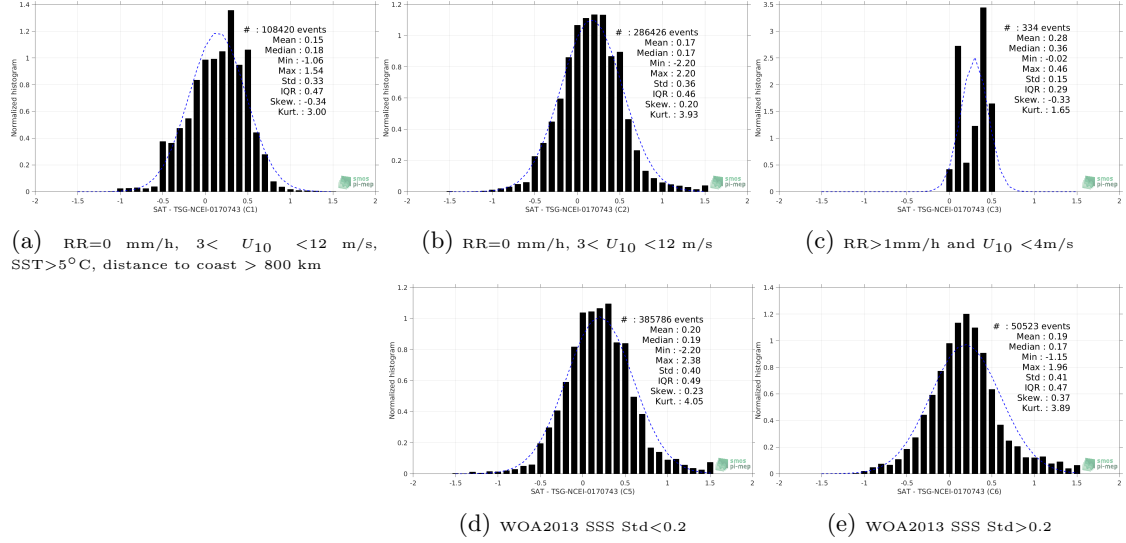
Figure 13: Normalized histogram of \Delta\text{SSS} (SMOS-L3-CATDS-CECOS-LOCEAN-V3-9DAYS-25KM - TSG-NCEI-0170743) for 5 different subdatasets corresponding to: RR=0 mm/h, 3 < U_{10} < 12 m/s, SST > 5^\circ\text{C} , distance to coast > 800 km (a), RR=0 mm/h, 3 < U_{10} < 12 m/s (b), RR > 1\text{mm/h} and U_{10} < 4\text{m/s} (c), WOA2013 SSS Std < 0.2 (d), WOA2013 SSS Std > 0.2 (e).
