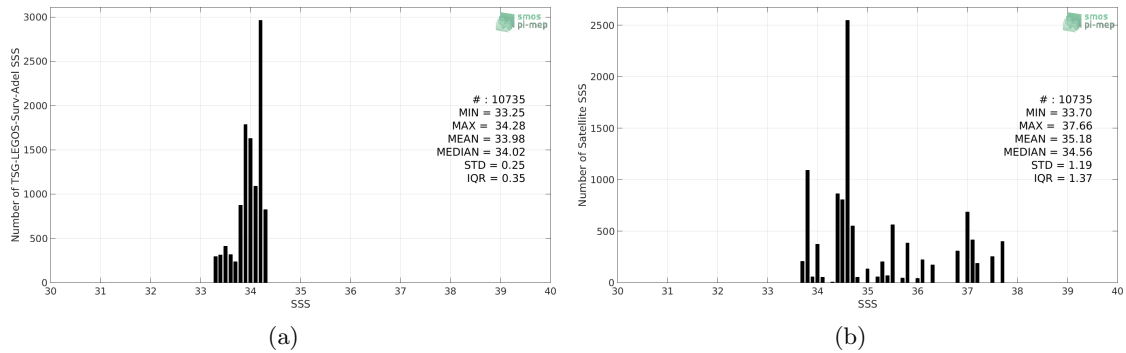
Figure 2: Histograms of SSS from TSG-LEGOS-Surv-Adel (a) and SMOS-L3-CATDS-CECOS-LOCEAN-V3-9DAYS-25KM (b) considering all match-up pairs per bins of 0.1 over the Global Ocean Pi-MEP region and for the full satellite product period.
