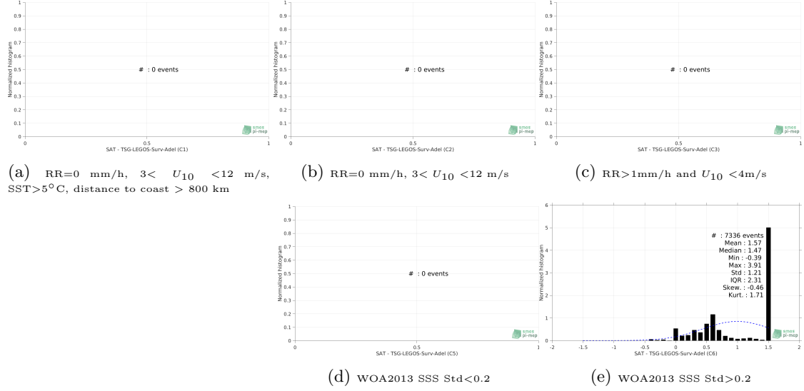
Figure 13: Normalized histogram of \Delta\text{SSS} (SMOS-L3-CATDS-CECOS-LOCEAN-V3-9DAYS-25KM - TSG-LEGOS-Surv-Adel) for 5 different subdatasets corresponding to: RR=0 mm/h, 3 < U_{10} < 12 m/s, SST > 5^\circ\text{C} , distance to coast > 800 km (a), RR=0 mm/h, 3 < U_{10} < 12 m/s (b), RR > 1\text{mm/h} and U_{10} < 4\text{m/s} (c), WOA2013 SSS Std <0.2 (d), WOA2013 SSS Std >0.2 (e).
