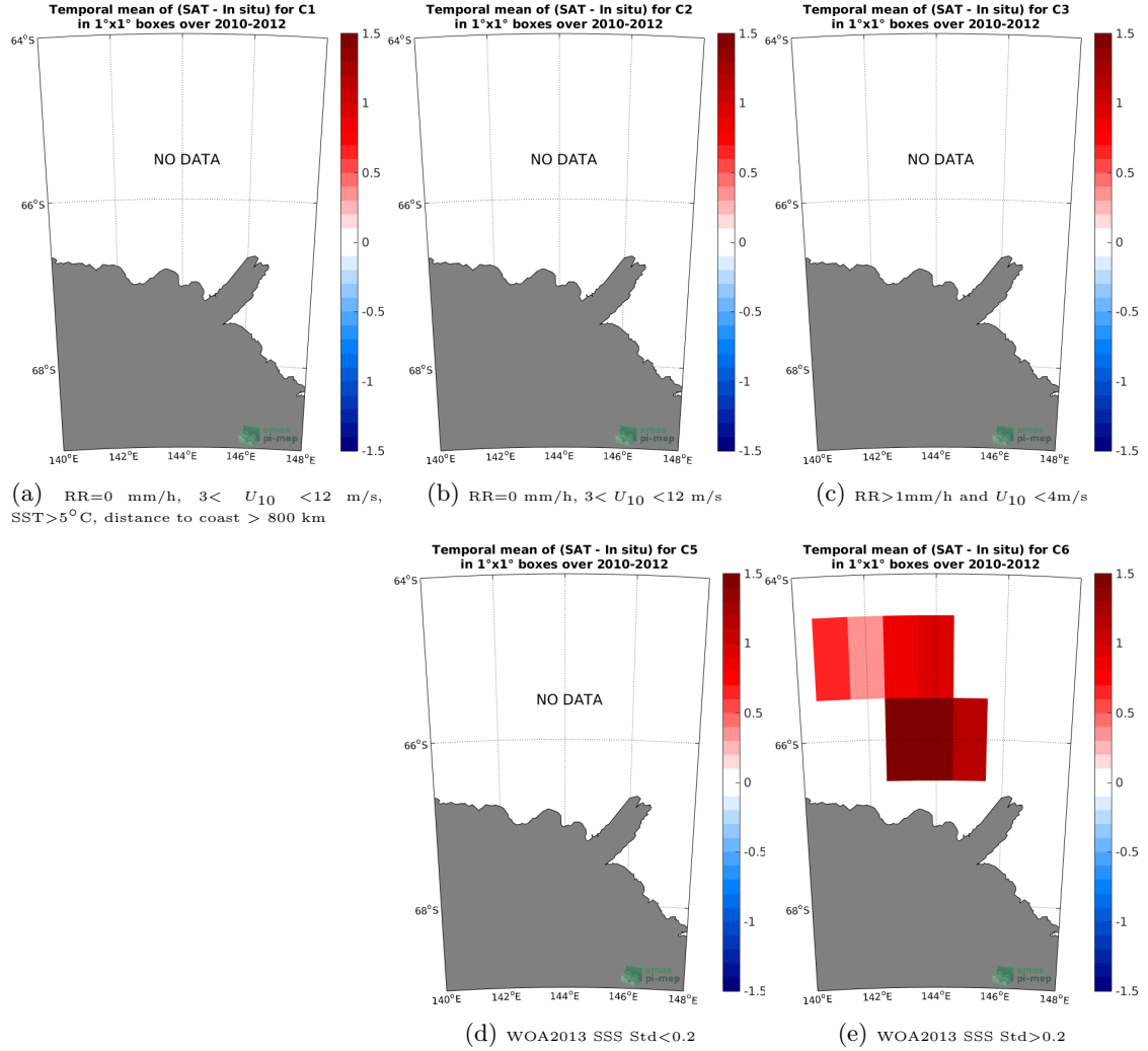
Figure 12: Temporal mean gridded over spatial boxes of size 1^\circ \times 1^\circ of \Delta SSS (SMOS-L3-CATDS-CECOS-LOCEAN-V3-9DAYS-25KM - TSG-LEGOS-Surv-Adel) for 5 different subdatasets corresponding to: RR=0 mm/h, 3 < U_{10} < 12 m/s, SST>5°C, distance to coast > 800 km (a), RR=0 mm/h, 3 < U_{10} < 12 m/s (b), RR>1mm/h and U_{10} < 4 m/s (c), WOA2013 SSS Std<0.2 (d), WOA2013 SSS Std>0.2 (e).
