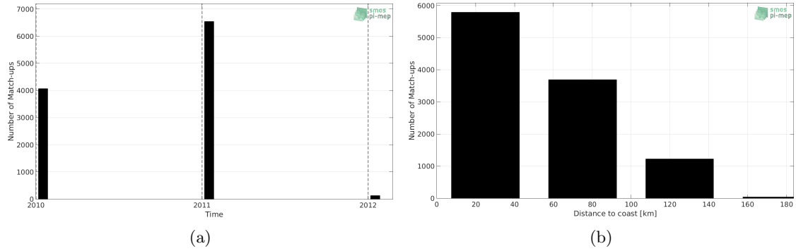
Figure 1: Number of match-ups between TSG-LEGOS-Surv-Adel and SMOS-L3-CATDS-CECOS-LOCEAN-V3-9DAYS-25KM SSS as a function of time (a) and as function of the distance to coast (b) over the Global Ocean Pi-MEP region and for the full satellite product period.
