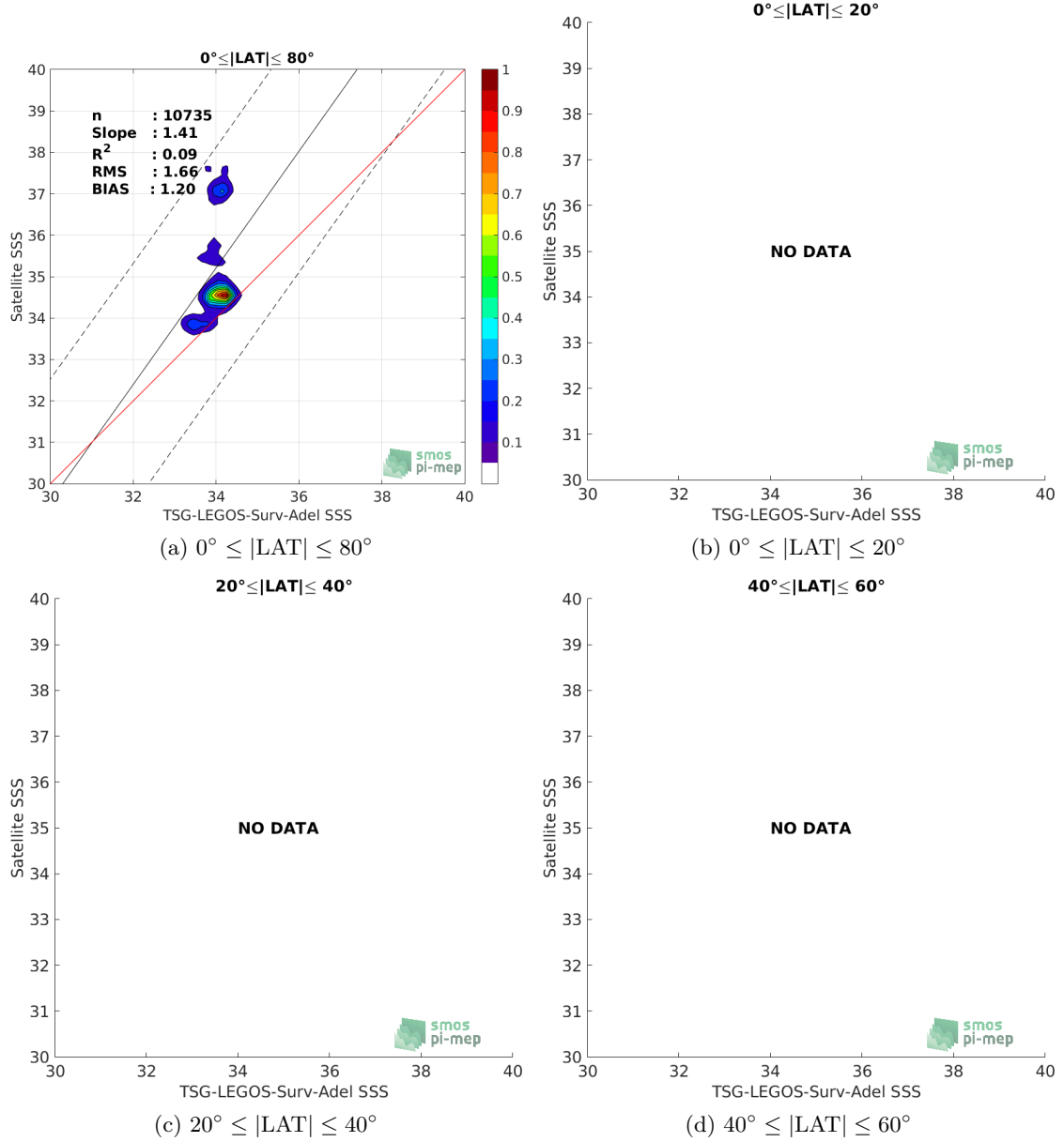
Figure 9: Contour maps of the concentration of SMOS-L3-CATDS-CECOS-LOCEAN-V3-9DAYS-25KM SSS (y-axis) versus TSG-LEGOS-Surv-Adel SSS (x-axis) at match-up pairs for different latitude bands. For each plot, the red line shows x=y . The black thin and dashed lines indicate a linear fit through the data cloud and the \pm 95\% confidence levels, respectively. The number match-up pairs n , the slope and R^2 coefficient of the linear fit, the root mean square (RMS) and the mean bias between satellite and in situ data are indicated for each latitude band in each plots.
