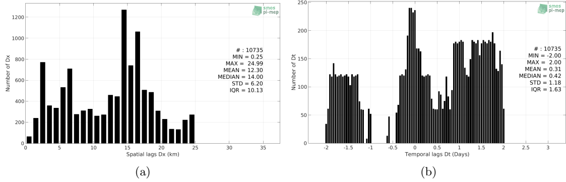
Figure 5: Histograms of the spatial (a) and temporal (b) lags between the time of the TSG-LEGOS-Surv-Adel measurements and the date of the corresponding SMOS-L3-CATDS-CECOS-LOCEAN-V3-9DAYS-25KM SSS product.
