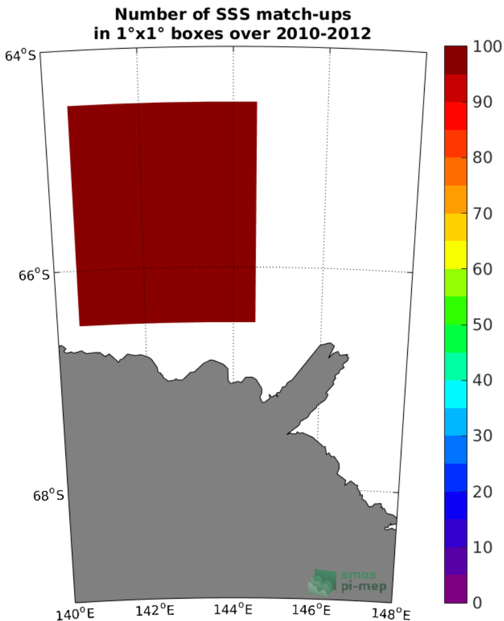
Figure 4: Number of SSS match-ups between TSG-LEGOS-Surv-Adel SSS and the SMOS-L3-CATDS-CECOS-LOCEAN-V3-9DAYS-25KM SSS product for the Global Ocean Pi-MEP region over 1°x1° boxes and for the full satellite product period.
