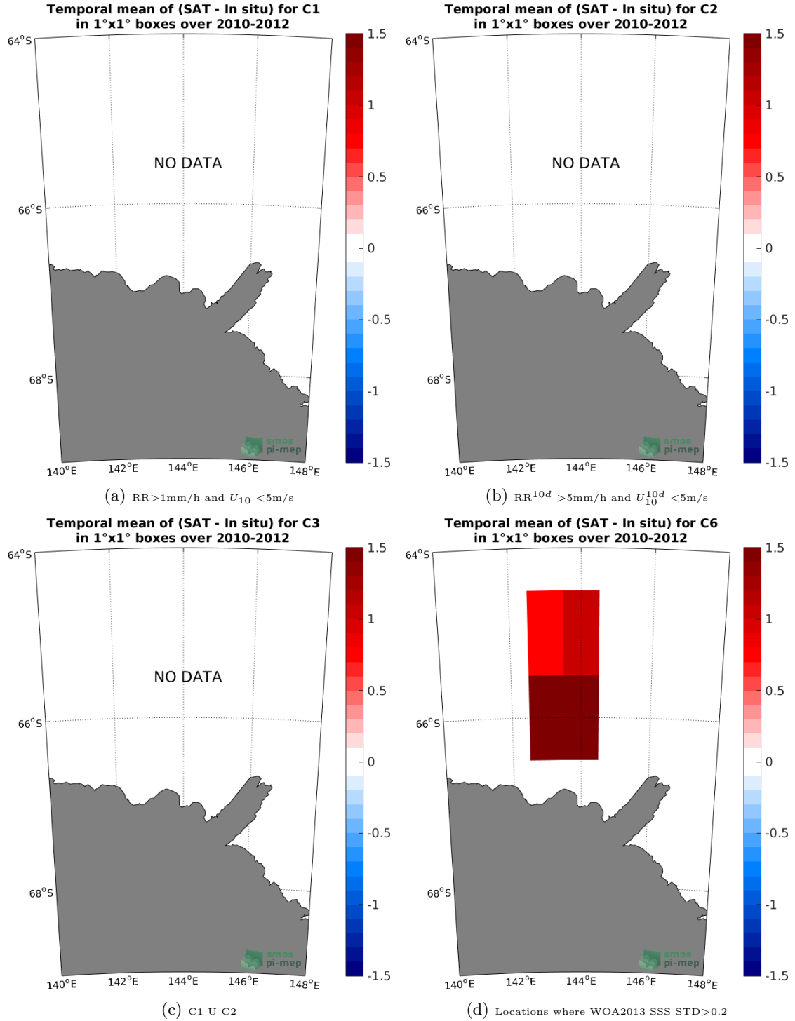
Figure 12: Temporal mean gridded over spatial boxes of size 1°x1° of \Delta\text{SSS} (SMOS-L3-CATDS-CECOS-LOCEAN-V3-9DAYS-25KM - TSG-LEGOS-Surv-Adel) for 4 different subdatasets corresponding to: RR > 1\text{mm/h} and U_{10} < 5\text{m/s} (a), RR^{10d} > 5\text{mm/h} and U_{10}^{10d} < 5\text{m/s} (b), C1 U C2 (c), Locations where WOA2013 SSS STD > 0.2 (d).
