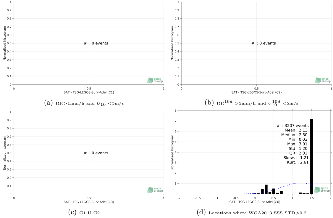
Figure 13: Normalized histogram of \Delta\text{SSS} (SMOS-L3-CATDS-CECOS-LOCEAN-V3-9DAYS-25KM - TSG-LEGOS-Surv-Adel) for 6 different subdatasets corresponding to: RR > 1\text{mm/h} and U_{10} < 5\text{m/s} (a), RR^{10d} > 5\text{mm/h} and U_{10}^{10d} < 5\text{m/s} (b), C1 U C2 (c), Locations where WOA2013 SSS STD > 0.2 (d).
