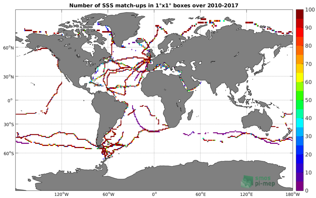
Figure 4: Number of SSS match-ups between TSG-GOSUD-Sailing-ship SSS and the SMOS-L3-CATDS-CECOS-LOCEAN-V3-9DAYS-25KM SSS product for the Global Ocean Pi-MEP region over 1^\circ \times 1^\circ boxes and for the full satellite product period.
