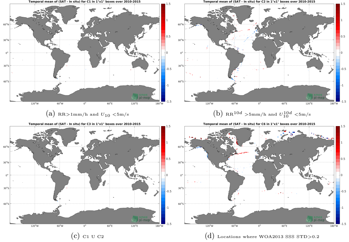
Figure 12: Temporal mean gridded over spatial boxes of size 1^\circ \times 1^\circ of \Delta SSS (SMOS-L3-CATDS-CECOS-LOCEAN-V3-9DAYS-25KM - TSG-GOSUD-Sailing-ship) for 4 different subdatasets corresponding to: RR > 1\text{mm/h} and U_{10} < 5\text{m/s} (a), RR^{10d} > 5\text{mm/h} and U_{10}^{10d} < 5\text{m/s} (b), C1 \cup C2 (c), Locations where WOA2013 SSS STD > 0.2 (d).
