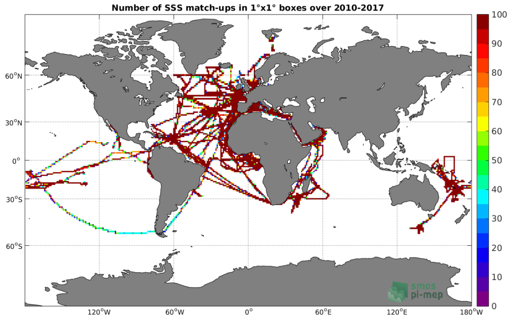
Figure 4: Number of SSS match-ups between TSG-GOSUD-Research-vessel SSS and the SMOS-L3-CATDS-CECOS-LOCEAN-V3-9DAYS-25KM SSS product for the Global Ocean Pi-MEP region over 1°x1° boxes and for the full satellite product period.
