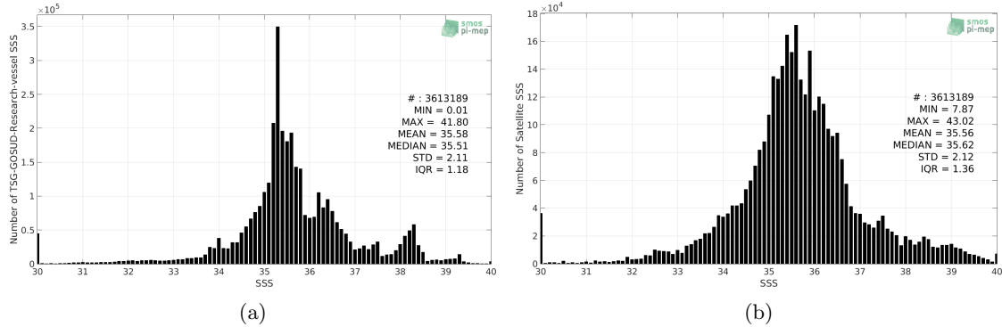
Figure 2: Histograms of SSS from TSG-GOSUD-Research-vessel (a) and SMOS-L3-CATDS-CECOS-LOCEAN-V3-9DAYS-25KM (b) considering all match-up pairs per bins of 0.1 over the Global Ocean Pi-MEP region and for the full satellite product period.
