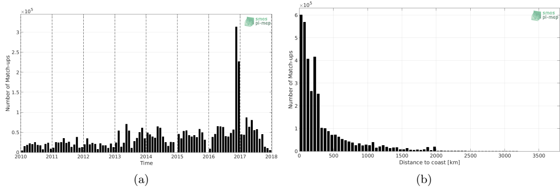
Figure 1: Number of match-ups between TSG-GOSUD-Research-vessel and SMOS-L3-CATDS-CECOS-LOCEAN-V3-9DAYS-25KM SSS as a function of time (a) and as function of the distance to coast (b) over the Global Ocean Pi-MEP region and for the full satellite product period.
