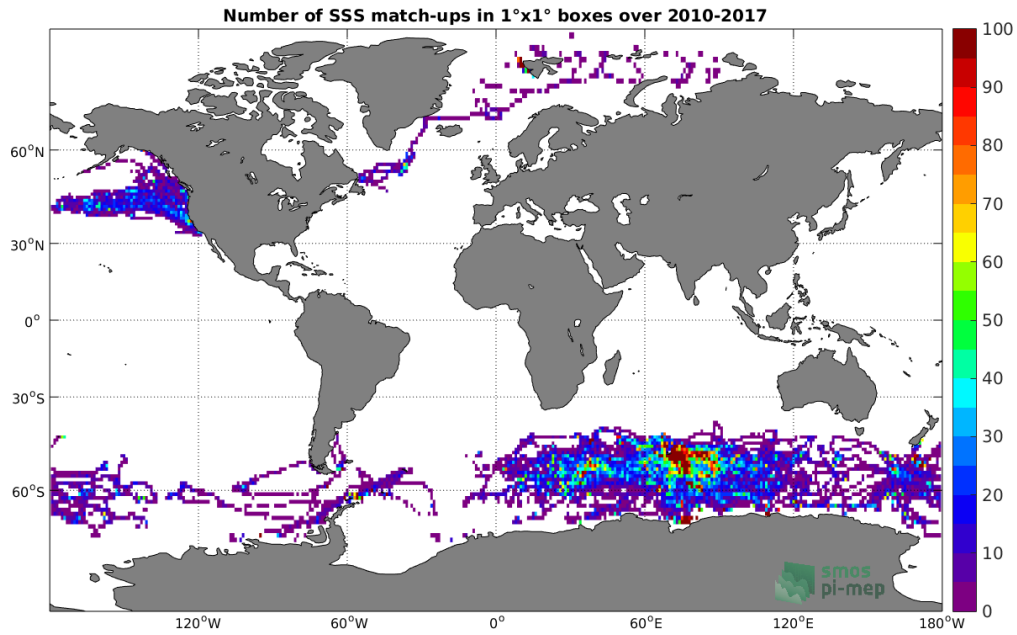
Figure 4: Number of SSS match-ups between Sea mammals SSS and the SMOS-L3-CATDS-CECOS-LOCEAN-V3-9DAYS-25KM SSS product for the Global Ocean Pi-MEP region over 1^\circ \times 1^\circ boxes and for the full satellite product period.
