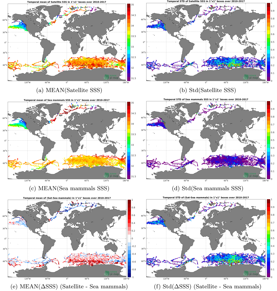
Figure 6: Temporal mean (left) and Std (right) of SSS from SMOS-L3-CATDS-CECOS-LOCEAN-V3-9DAYS-25KM (top), Sea mammals (middle), and of \Delta SSS (Satellite - Sea mammals). Only match-up pairs are used to generate these maps.
