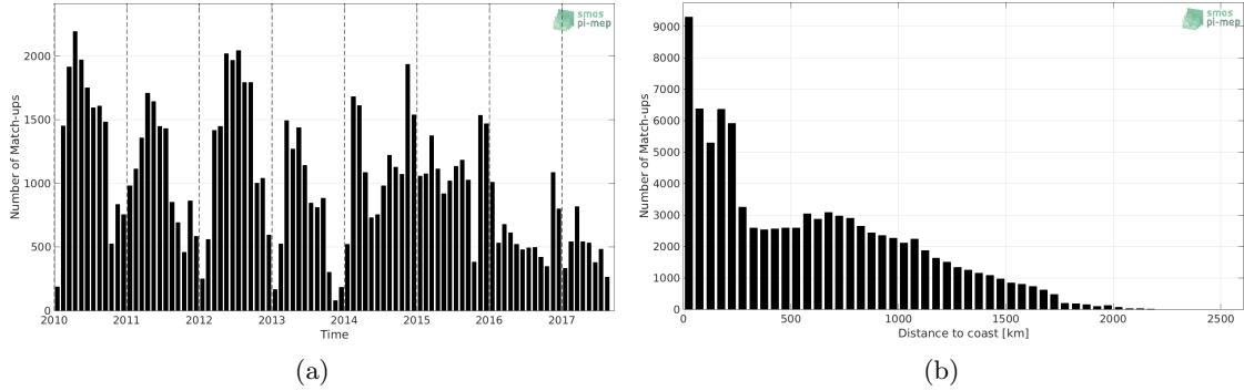
Figure 1: Number of match-ups between Sea mammals and SMOS-L3-CATDS-CECOS-LOCEAN-V3-9DAYS-25KM SSS as a function of time (a) and as function of the distance to coast (b) over the Global Ocean Pi-MEP region and for the full satellite product period.
