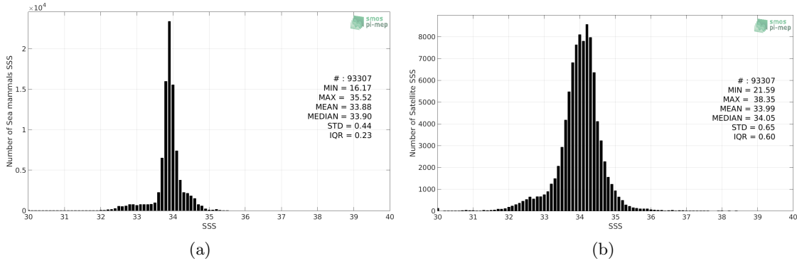
Figure 2: Histograms of SSS from Sea mammals (a) and SMOS-L3-CATDS-CECOS-LOCEAN-V3-9DAYS-25KM (b) considering all match-up pairs per bins of 0.1 over the Global Ocean Pi-MEP region and for the full satellite product period.
