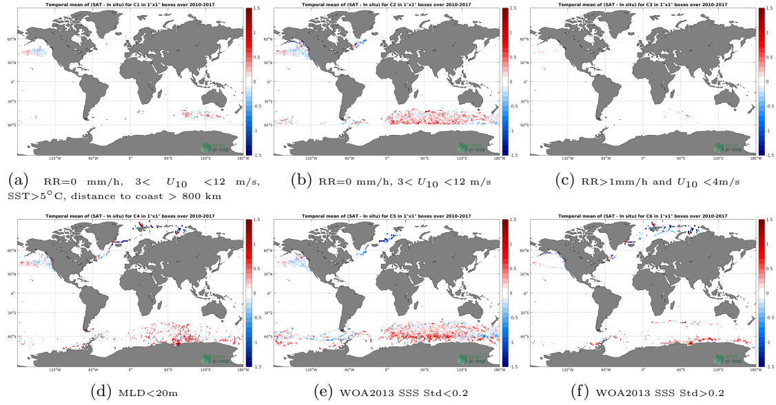
Figure 12: Temporal mean gridded over spatial boxes of size 1^\circ \times 1^\circ of \Delta SSS (SMOS-L3-CATDS-CECOS-LOCEAN-V3-9DAYS-25KM - Sea mammals) for 6 different subdatasets corresponding to: RR=0 mm/h, 3 < U_{10} < 12 m/s, SST > 5^\circ C , distance to coast > 800 km (a), RR=0 mm/h, 3 < U_{10} < 12 m/s (b), RR > 1 mm/h and U_{10} < 4 m/s (c), MLD < 20 m (d), WOA2013 SSS Std < 0.2 (e), WOA2013 SSS Std > 0.2 (f).
