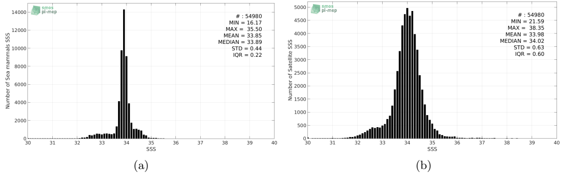
Figure 2: Histograms of SSS from Sea mammals (a) and SMOS-L3-CATDS-CECOS-LOCEAN-V3-9DAYS-25KM (b) considering all match-up pairs per bins of 0.1 over the Global Ocean Pi-MEP region and for the full satellite product period.
