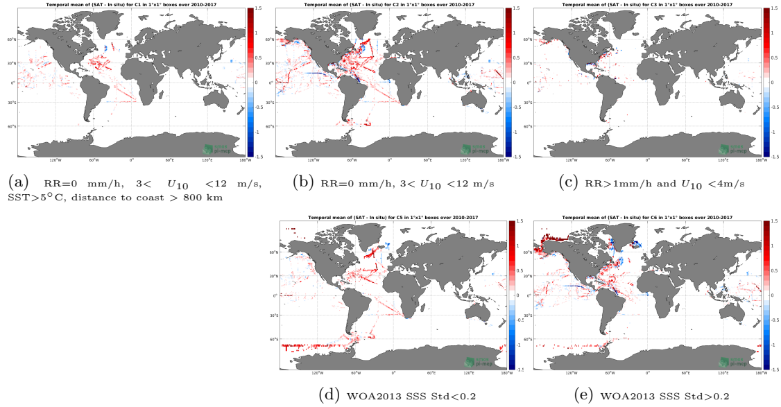
Figure 12: Temporal mean gridded over spatial boxes of size 1^\circ \times 1^\circ of \Delta SSS (SMOS-L3-CATDS-CECOS-LOCEAN-V3-18DAYS-25KM - TSG-SAMOS) for 5 different subdatasets corresponding to: RR=0 mm/h, 3 < U_{10} < 12 m/s, SST > 5^\circ C , distance to coast > 800 km (a), RR=0 mm/h, 3 < U_{10} < 12 m/s (b), RR > 1 mm/h and U_{10} < 4 m/s (c), WOA2013 SSS Std < 0.2 (d), WOA2013 SSS Std > 0.2 (e).
