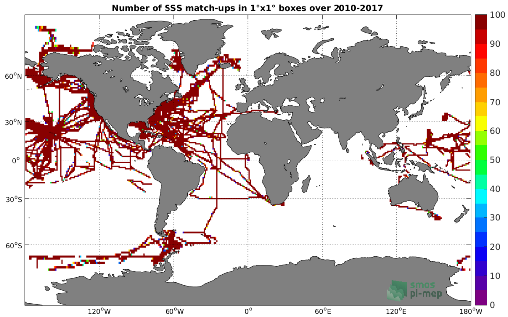
Figure 4: Number of SSS match-ups between TSG-SAMOS SSS and the SMOS-L3-CATDS-CECOS-LOCEAN-V3-18DAYS-25KM SSS product for the Global Ocean Pi-MEP region over 1°x1° boxes and for the full satellite product period.
