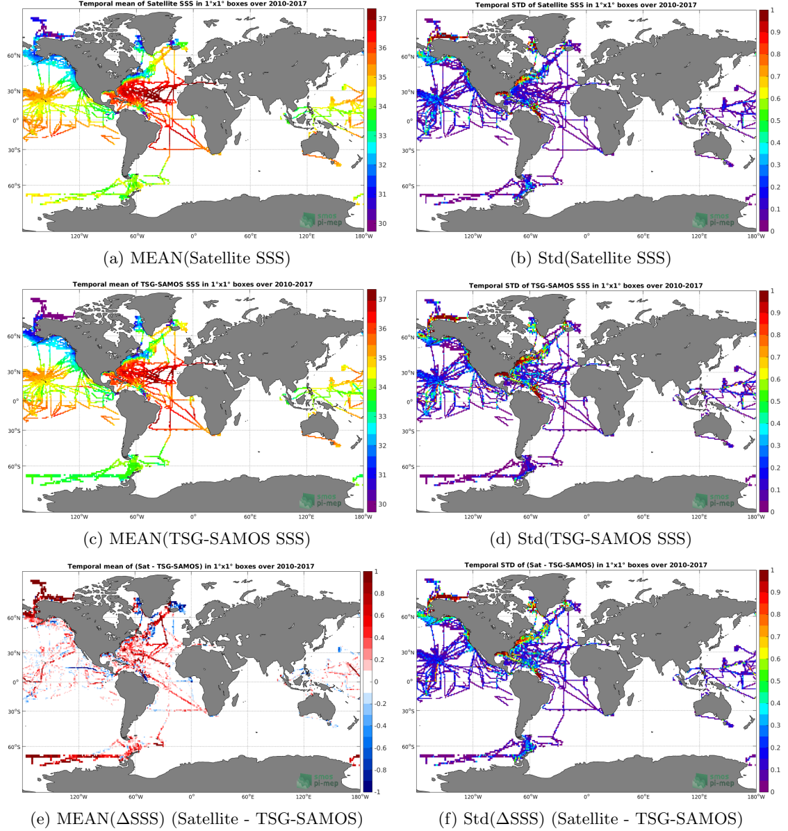
Figure 6: Temporal mean (left) and Std (right) of SSS from SMOS-L3-CATDS-CECOS-LOCEAN-V3-18DAYS-25KM (top), TSG-SAMOS (middle), and of \Delta SSS (Satellite - TSG-SAMOS). Only match-up pairs are used to generate these maps.
