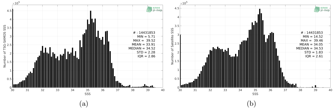
Figure 2: Histograms of SSS from TSG-SAMOS (a) and SMOS-L3-CATDS-CECOS-LOCEAN-V3-18DAYS-25KM (b) considering all match-up pairs per bins of 0.1 over the Global Ocean Pi-MEP region and for the full satellite product period.
