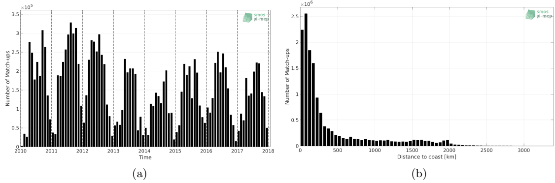
Figure 1: Number of match-ups between TSG-SAMOS and SMOS-L3-CATDS-CECOS-LOCEAN-V3-18DAYS-25KM SSS as a function of time (a) and as function of the distance to coast (b) over the Global Ocean Pi-MEP region and for the full satellite product period.
