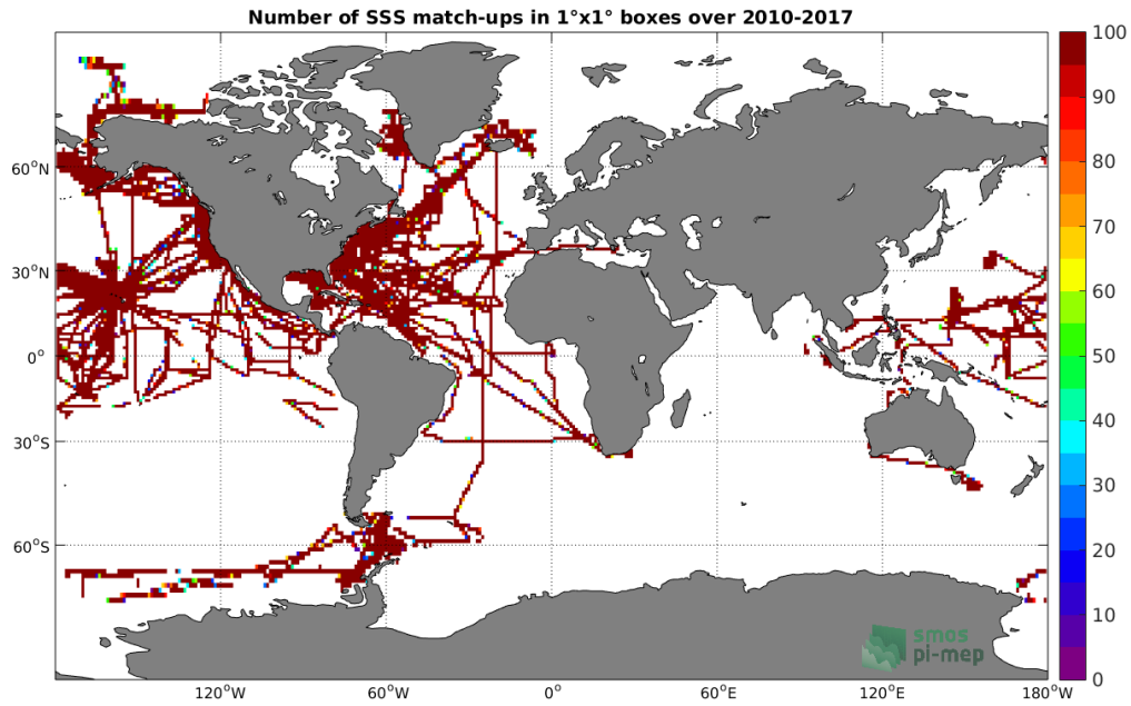
Figure 4: Number of SSS match-ups between TSG-SAMOS SSS and the SMOS-L3-CATDS-CECOS-LOCEAN-V3-18DAYS-25KM SSS product for the Global Ocean Pi-MEP region over 1^\circ \times 1^\circ boxes and for the full satellite product period.
