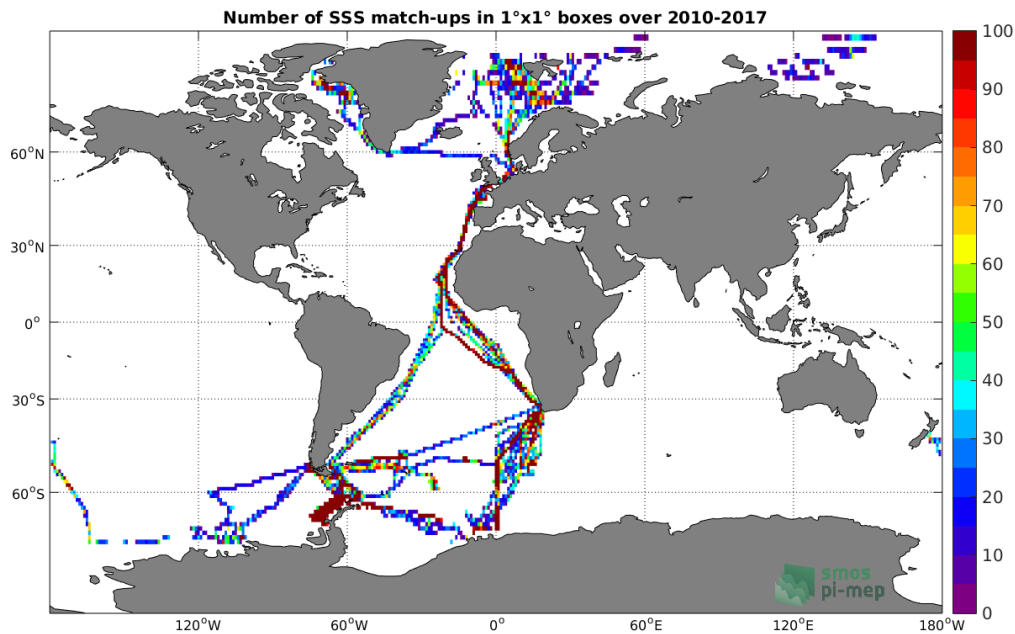
Figure 4: Number of SSS match-ups between TSG-POLARSTERN SSS and the SMOS-L3-CATDS-CECOS-LOCEAN-V3-18DAYS-25KM SSS product for the Global Ocean Pi-MEP region over 1^\circ \times 1^\circ boxes and for the full satellite product period.
