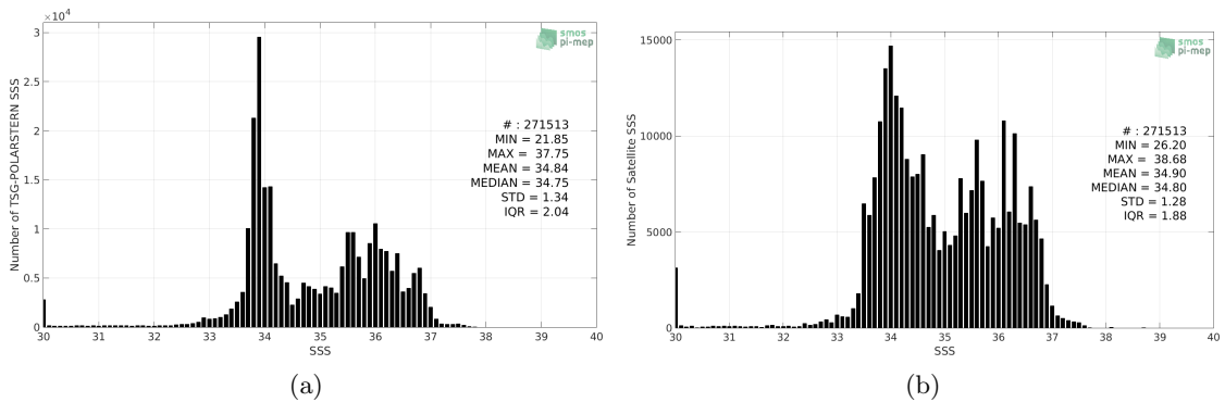
Figure 2: Histograms of SSS from TSG-POLARSTERN (a) and SMOS-L3-CATDS-CECOS-LOCEAN-V3-18DAYS-25KM (b) considering all match-up pairs per bins of 0.1 over the Global Ocean Pi-MEP region and for the full satellite product period.
