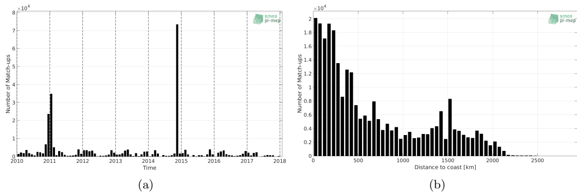
Figure 1: Number of match-ups between TSG-POLARSTERN and SMOS-L3-CATDS-CECOS-LOCEAN-V3-18DAYS-25KM SSS as a function of time (a) and as function of the distance to coast (b) over the Global Ocean Pi-MEP region and for the full satellite product period.
