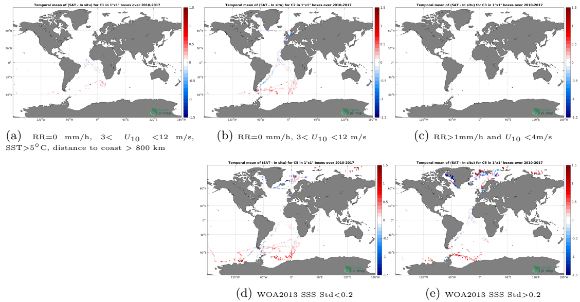
Figure 12: Temporal mean gridded over spatial boxes of size 1^\circ \times 1^\circ of \Delta SSS (SMOS-L3-CATDS-CECOS-LOCEAN-V3-18DAYS-25KM - TSG-POLARSTERN) for 5 different subdatasets corresponding to:RR=0 mm/h, 3 < U_{10} < 12 m/s, SST > 5^\circ C, distance to coast > 800 km (a), RR=0 mm/h, 3 < U_{10} < 12 m/s (b), RR > 1 mm/h and U_{10} < 4 m/s (c), WOA2013 SSS Std < 0.2 (d), WOA2013 SSS Std > 0.2 (e).
