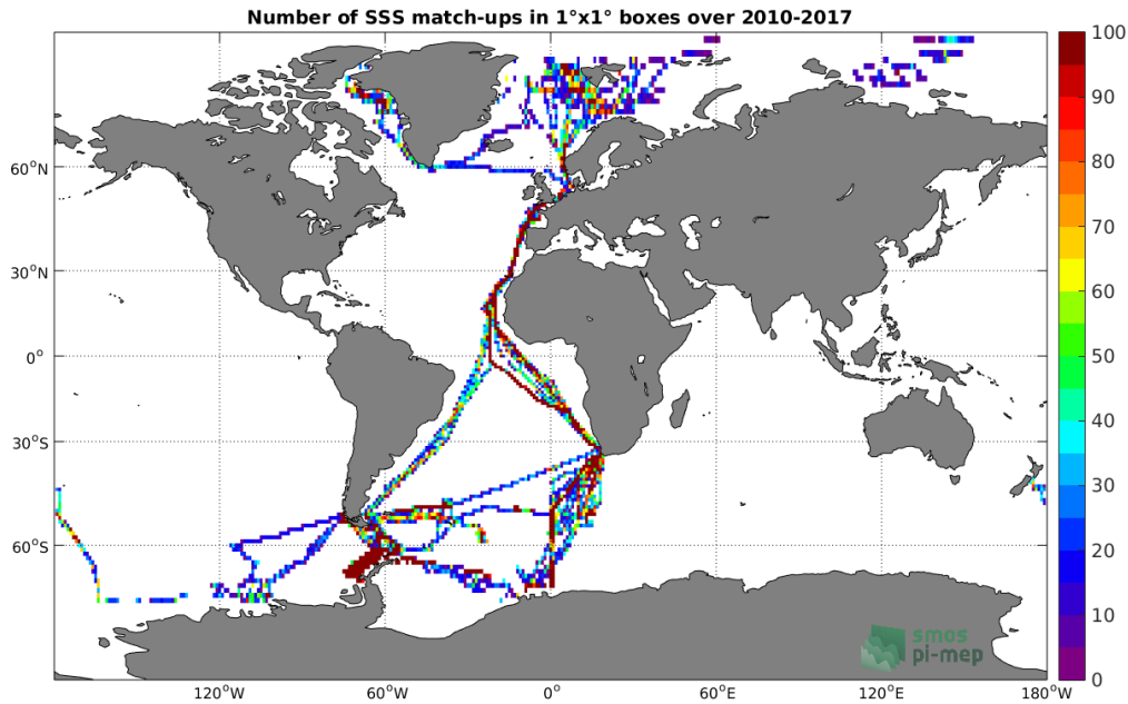
Figure 4: Number of SSS match-ups between TSG-POLARSTERN SSS and the SMOS-L3-CATDS-CECOS-LOCEAN-V3-18DAYS-25KM SSS product for the Global Ocean Pi-MEP region over 1°x1° boxes and for the full satellite product period.
