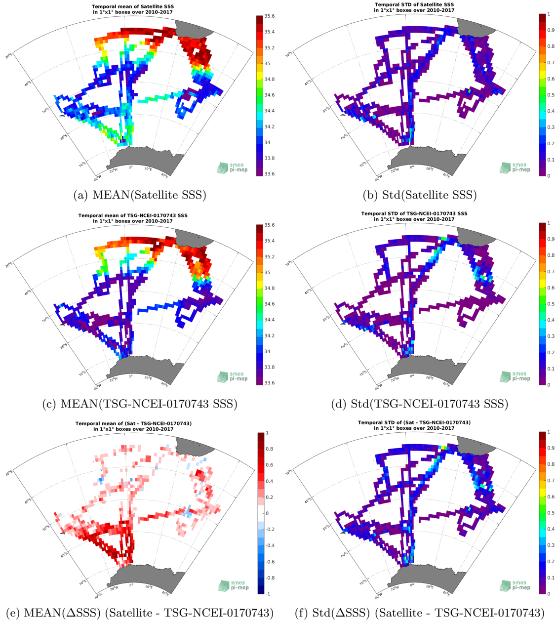
Figure 6: Temporal mean (left) and Std (right) of SSS from SMOS-L3-CATDS-CECOS-LOCEAN-V3-18DAYS-25KM (top), TSG-NCEI-0170743 (middle), and of \Delta SSS (Satellite - TSG-NCEI-0170743). Only match-up pairs are used to generate these maps.
