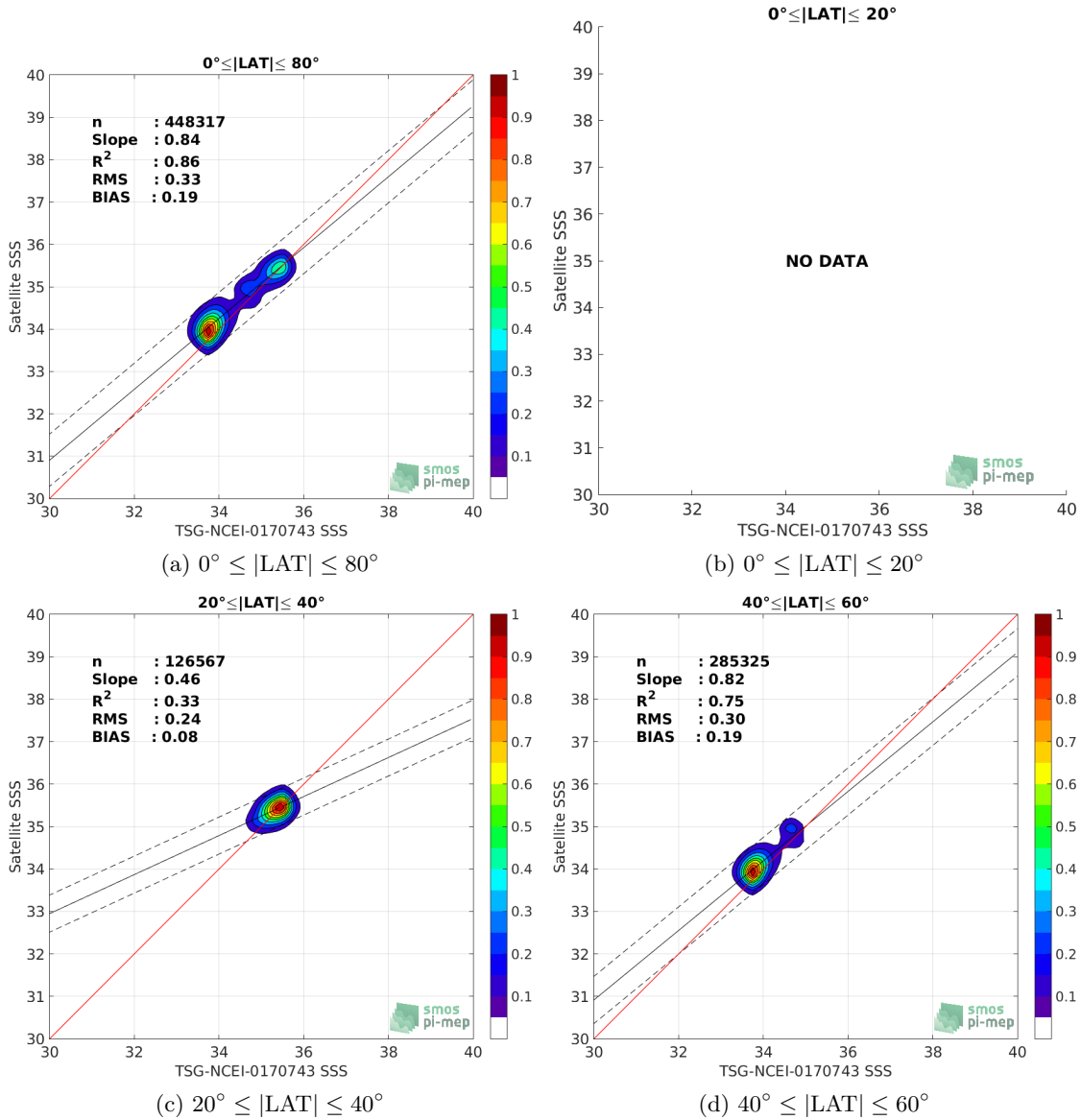
Figure 9: Contour maps of the concentration of SMOS-L3-CATDS-CECOS-LOCEAN-V3-18DAYS-25KM SSS (y-axis) versus TSG-NCEI-0170743 SSS (x-axis) at match-up pairs for different latitude bands. For each plot, the red line shows x=y . The black thin and dashed lines indicate a linear fit through the data cloud and the \pm 95\% confidence levels, respectively. The number match-up pairs n , the slope and R^2 coefficient of the linear fit, the root mean square (RMS) and the mean bias between satellite and in situ data are indicated for each latitude band in each plots.
