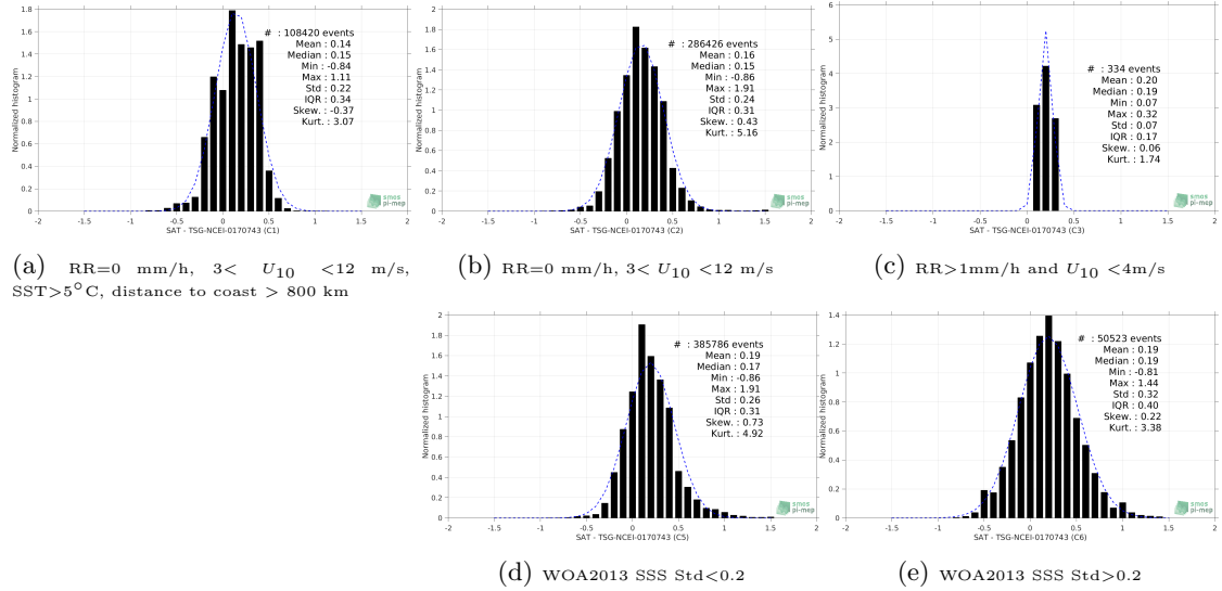
Figure 13: Normalized histogram of \Delta SSS (SMOS-L3-CATDS-CECOS-LOCEAN-V3-18DAYS-25KM - TSG-NCEI-0170743) for 5 different subdatasets corresponding to: RR=0 mm/h, 3 < U_{10} < 12 m/s, SST > 5°C, distance to coast > 800 km (a), RR=0 mm/h, 3 < U_{10} < 12 m/s (b), RR > 1mm/h and U_{10} < 4 m/s (c), WOA2013 SSS Std < 0.2 (d), WOA2013 SSS Std > 0.2 (e).
