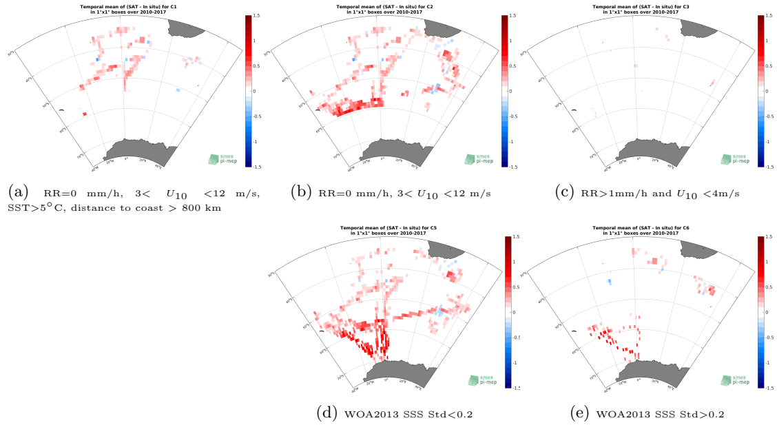
Figure 12: Temporal mean gridded over spatial boxes of size 1^\circ \times 1^\circ of \Delta SSS (SMOS-L3-CATDS-CECOS-LOCEAN-V3-18DAYS-25KM - TSG-NCEI-0170743) for 5 different subdatasets corresponding to:RR=0 mm/h, 3 < U_{10} < 12 m/s, SST >5^\circ C, distance to coast > 800 km (a), RR=0 mm/h, 3 < U_{10} < 12 m/s (b), RR >1 mm/h and U_{10} < 4 m/s (c), WOA2013 SSS Std <0.2 (d), WOA2013 SSS Std >0.2 (e).
