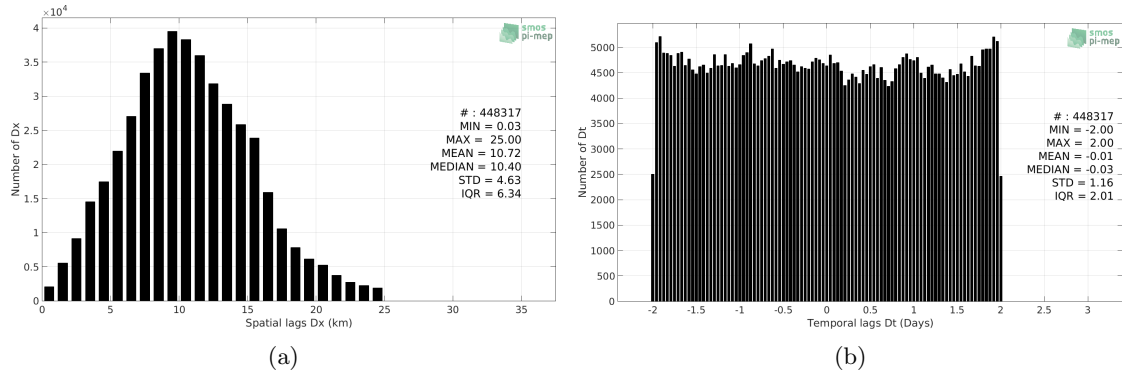
Figure 5: Histograms of the spatial (a) and temporal (b) lags between the time of the TSG-NCEI-0170743 measurements and the date of the corresponding SMOS-L3-CATDS-CECOS-LOCEAN-V3-18DAYS-25KM SSS product.
