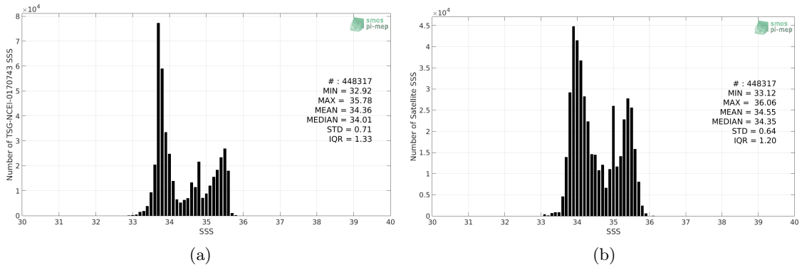
Figure 2: Histograms of SSS from TSG-NCEI-0170743 (a) and SMOS-L3-CATDS-CECOS-LOCEAN-V3-18DAYS-25KM (b) considering all match-up pairs per bins of 0.1 over the Global Ocean Pi-MEP region and for the full satellite product period.
