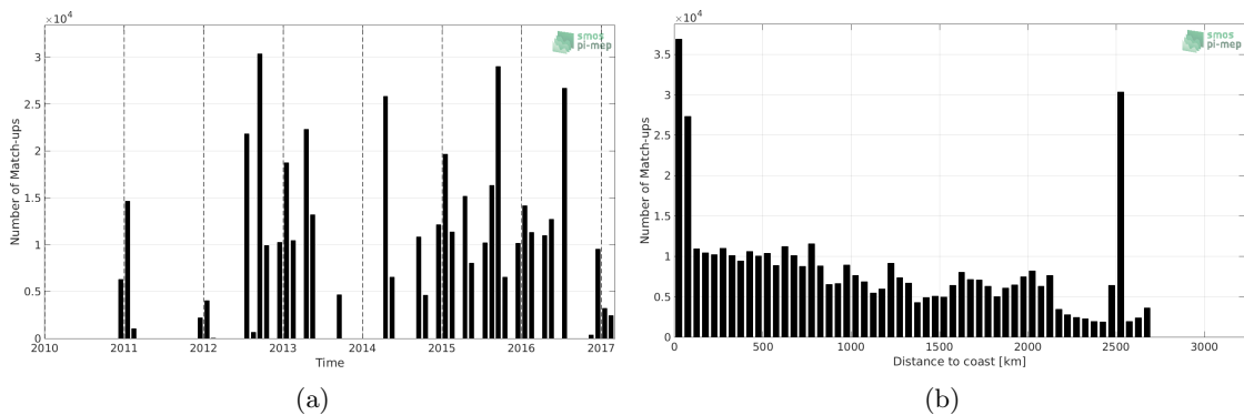
Figure 1: Number of match-ups between TSG-NCEI-0170743 and SMOS-L3-CATDS-CECOS-LOCEAN-V3-18DAYS-25KM SSS as a function of time (a) and as function of the distance to coast (b) over the Global Ocean Pi-MEP region and for the full satellite product period.
