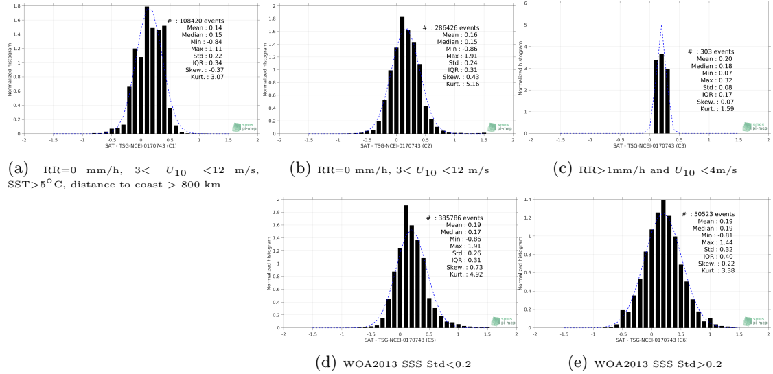
Figure 13: Normalized histogram of \Delta SSS (SMOS-L3-CATDS-CECOS-LOCEAN-V3-18DAYS-25KM - TSG-NCEI-0170743) for 5 different subdatasets corresponding to: RR=0 mm/h, 3 < U_{10} < 12 m/s, SST>5°C, distance to coast > 800 km (a), RR=0 mm/h, 3 < U_{10} < 12 m/s (b), RR>1mm/h and U_{10} < 4 m/s (c), WOA2013 SSS Std<0.2 (d), WOA2013 SSS Std>0.2 (e).
