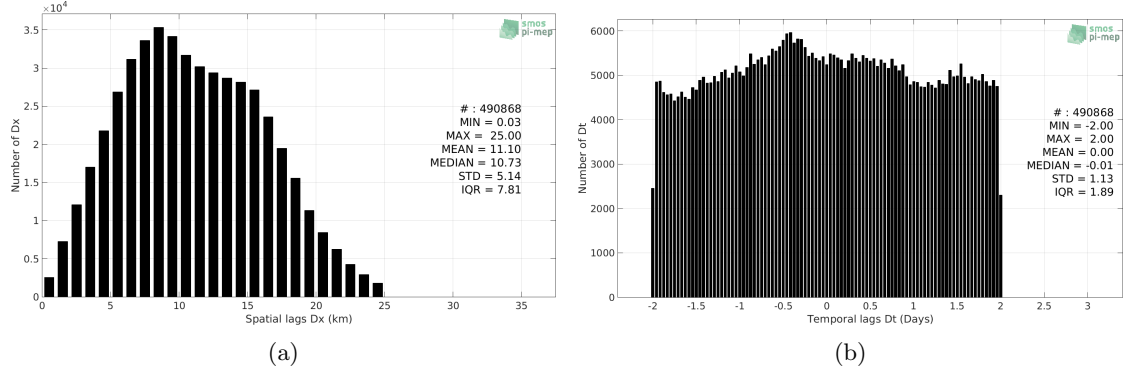
Figure 5: Histograms of the spatial (a) and temporal (b) lags between the time of the TSG-LEGOS-Survostral measurements and the date of the corresponding SMOS-L3-CATDS-CECOS-LOCEAN-V3-18DAYS-25KM SSS product.
