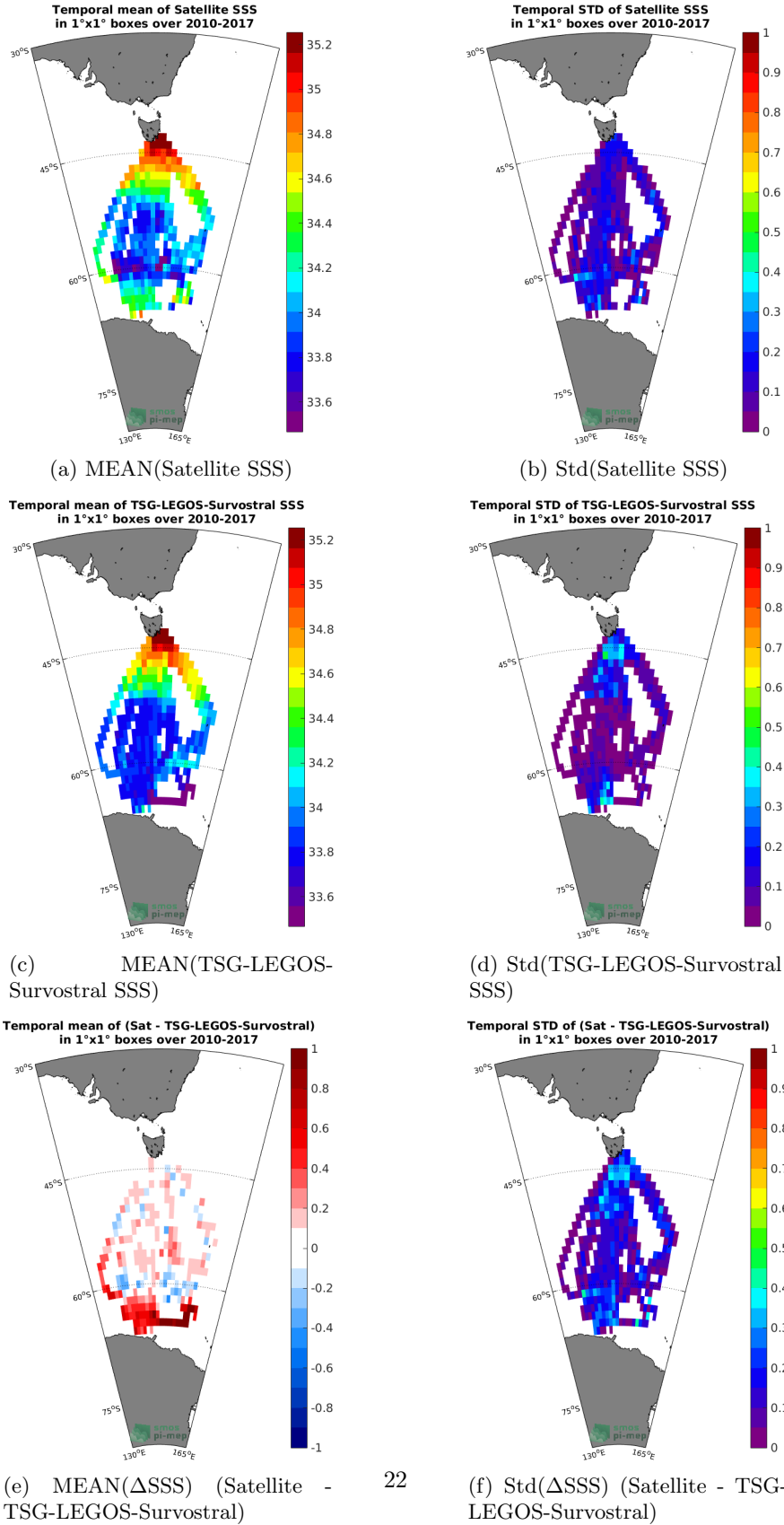
Figure 6: Temporal mean (left) and Std (right) of SSS from SMOS-L3-CATDS-CECOS-LOCEAN-V3-18DAYS-25KM (top), TSG-LEGOS-Survostral (middle), and of \Delta SSS (Satellite - TSG-LEGOS-Survostral). Only match-up pairs are used to generate these maps.
