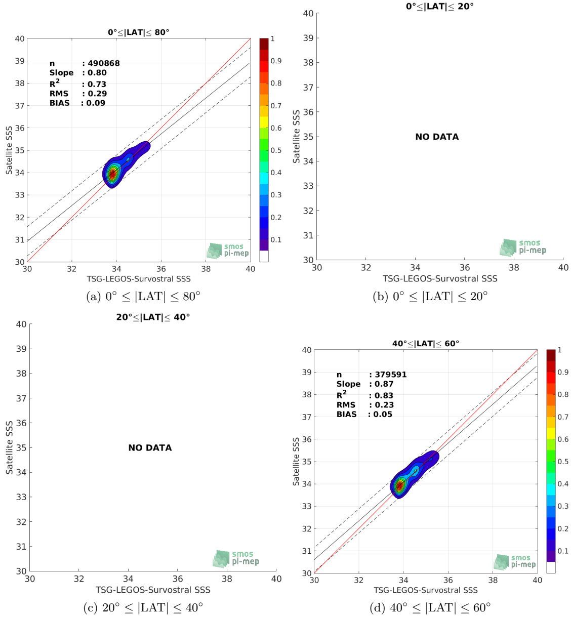
Figure 9: Contour maps of the concentration of SMOS-L3-CATDS-CECOS-LOCEAN-V3-18DAYS-25KM SSS (y-axis) versus TSG-LEGOS-Survostral SSS (x-axis) at match-up pairs for different latitude bands. For each plot, the red line shows x=y . The black thin and dashed lines indicate a linear fit through the data cloud and the \pm 95\% confidence levels, respectively. The number match-up pairs n , the slope and R^2 coefficient of the linear fit, the root mean square (RMS) and the mean bias between satellite and in situ data are indicated for each latitude band in each plots.
