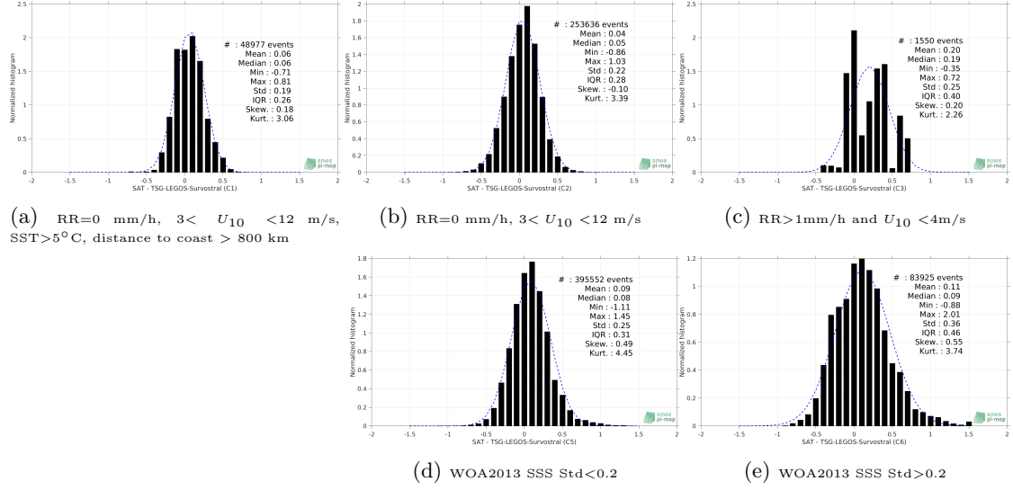
Figure 13: Normalized histogram of \Delta\text{SSS} (SMOS-L3-CATDS-CECOS-LOCEAN-V3-18DAYS-25KM - TSG-LEGOS-Survostral) for 5 different subdatasets corresponding to: RR=0 mm/h, 3 < U_{10} < 12 m/s, SST >5^{\circ}\text{C} , distance to coast > 800 km (a), RR=0 mm/h, 3 < U_{10} < 12 m/s (b), RR>1\text{mm/h} and U_{10} < 4\text{m/s} (c), WOA2013 SSS Std <0.2 (d), WOA2013 SSS Std >0.2 (e).
