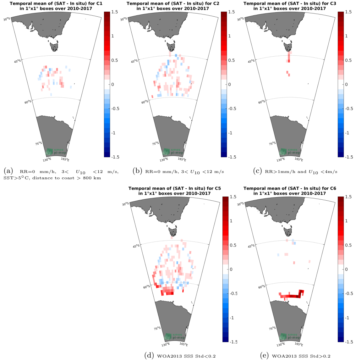
Figure 12: Temporal mean gridded over spatial boxes of size 1°x1° of \Delta\text{SSS} (SMOS-L3-CATDS-CECOS-LOCEAN-V3-18DAYS-25KM - TSG-LEGOS-Survostral) for 5 different subdatasets corresponding to: RR=0 mm/h, 3 < U_{10} < 12 m/s, SST > 5^\circ\text{C} , distance to coast > 800 km (a), RR=0 mm/h, 3 < U_{10} < 12 m/s (b), RR > 1 mm/h and U_{10} < 4 m/s (c), WOA2013 SSS Std < 0.2 (d), WOA2013 SSS Std > 0.2 (e).
