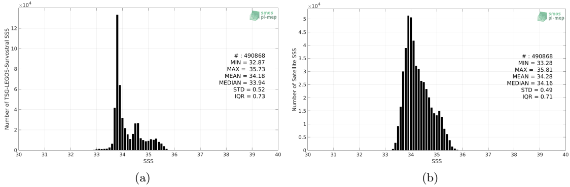
Figure 2: Histograms of SSS from TSG-LEGOS-Survostral (a) and SMOS-L3-CATDS-CECOS-LOCEAN-V3-18DAYS-25KM (b) considering all match-up pairs per bins of 0.1 over the Global Ocean Pi-MEP region and for the full satellite product period.
