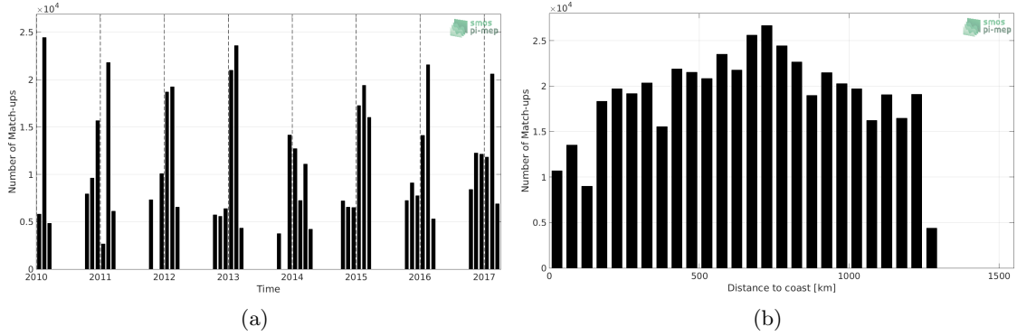
Figure 1: Number of match-ups between TSG-LEGOS-Survostral and SMOS-L3-CATDS-CECOS-LOCEAN-V3-18DAYS-25KM SSS as a function of time (a) and as function of the distance to coast (b) over the Global Ocean Pi-MEP region and for the full satellite product period.
