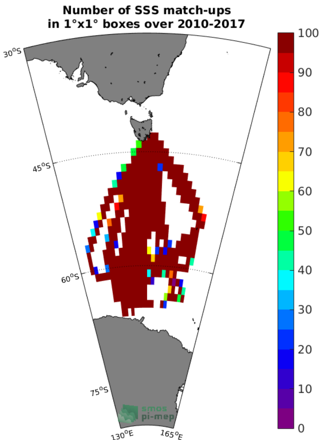
Figure 4: Number of SSS match-ups between TSG-LEGOS-Survostral SSS and the SMOS-L3-CATDS-CECOS-LOCEAN-V3-18DAYS-25KM SSS product for the Global Ocean Pi-MEP region over 1°x1° boxes and for the full satellite product period.
