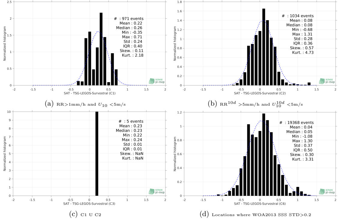
Figure 13: Normalized histogram of \Delta SSS (SMOS-L3-CATDS-CECOS-LOCEAN-V3-18DAYS-25KM - TSG-LEGOS-Survostral) for 6 different subdatasets corresponding to: RR > 1\text{mm/h} and U_{10} < 5\text{m/s} (a), RR^{10d} > 5\text{mm/h} and U_{10}^{10d} < 5\text{m/s} (b), C1 U C2 (c), Locations where WOA2013 SSS STD > 0.2 (d).
