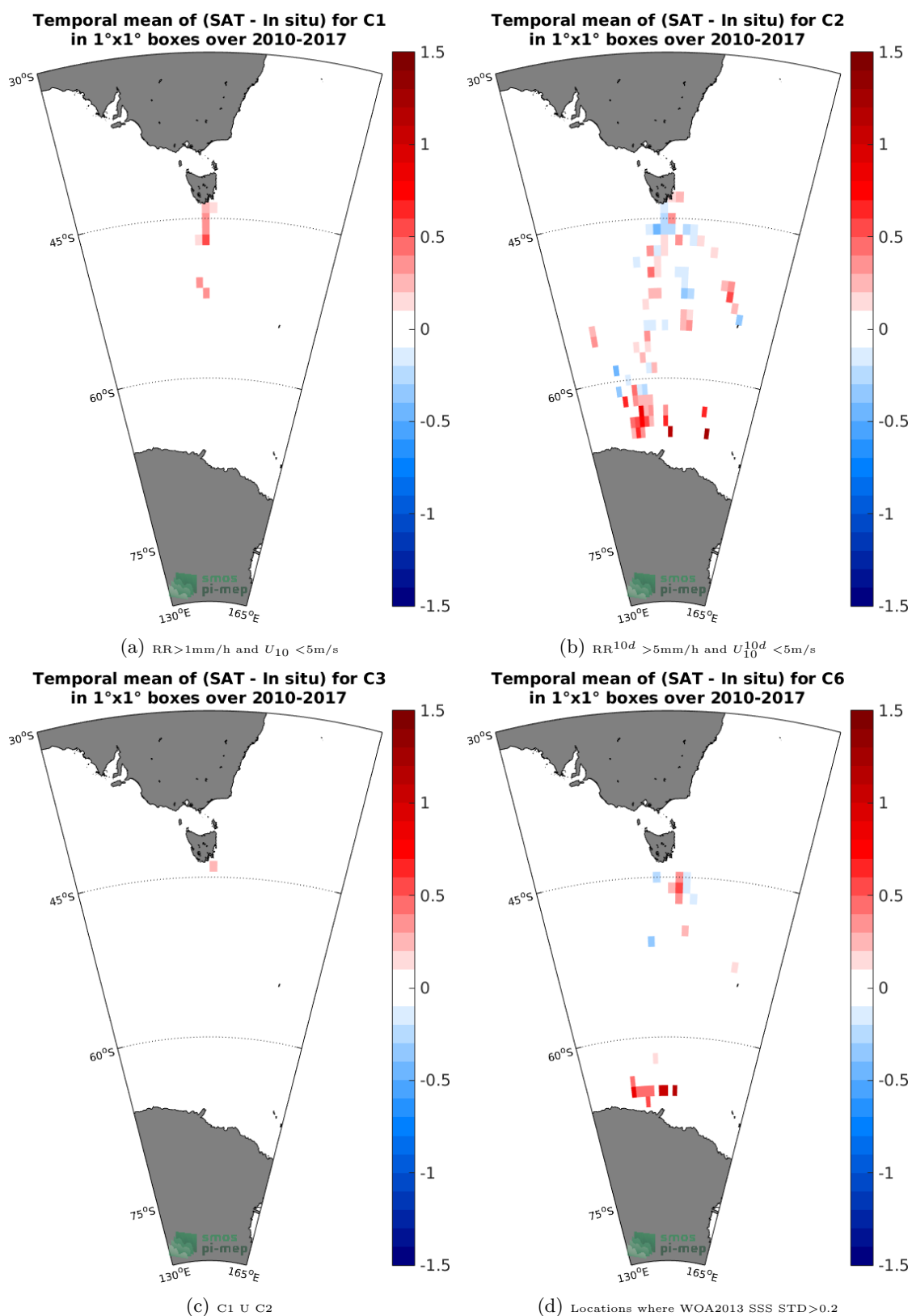
Figure 12: Temporal mean gridded over spatial boxes of size 1°x1° of \Delta\text{SSS} (SMOS-L3-CATDS-CECOS-LOCEAN-V3-18DAYS-25KM - TSG-LEGOS-Survostral) for 4 different subdatasets corresponding to: RR > 1\text{mm/h} and U_{10} < 5\text{m/s} (a), RR^{10d} > 5\text{mm/h} and U_{10}^{10d} < 5\text{m/s} (b), C1 U C2 (c), Locations where WOA2013 SSS STD > 0.2 (d).
