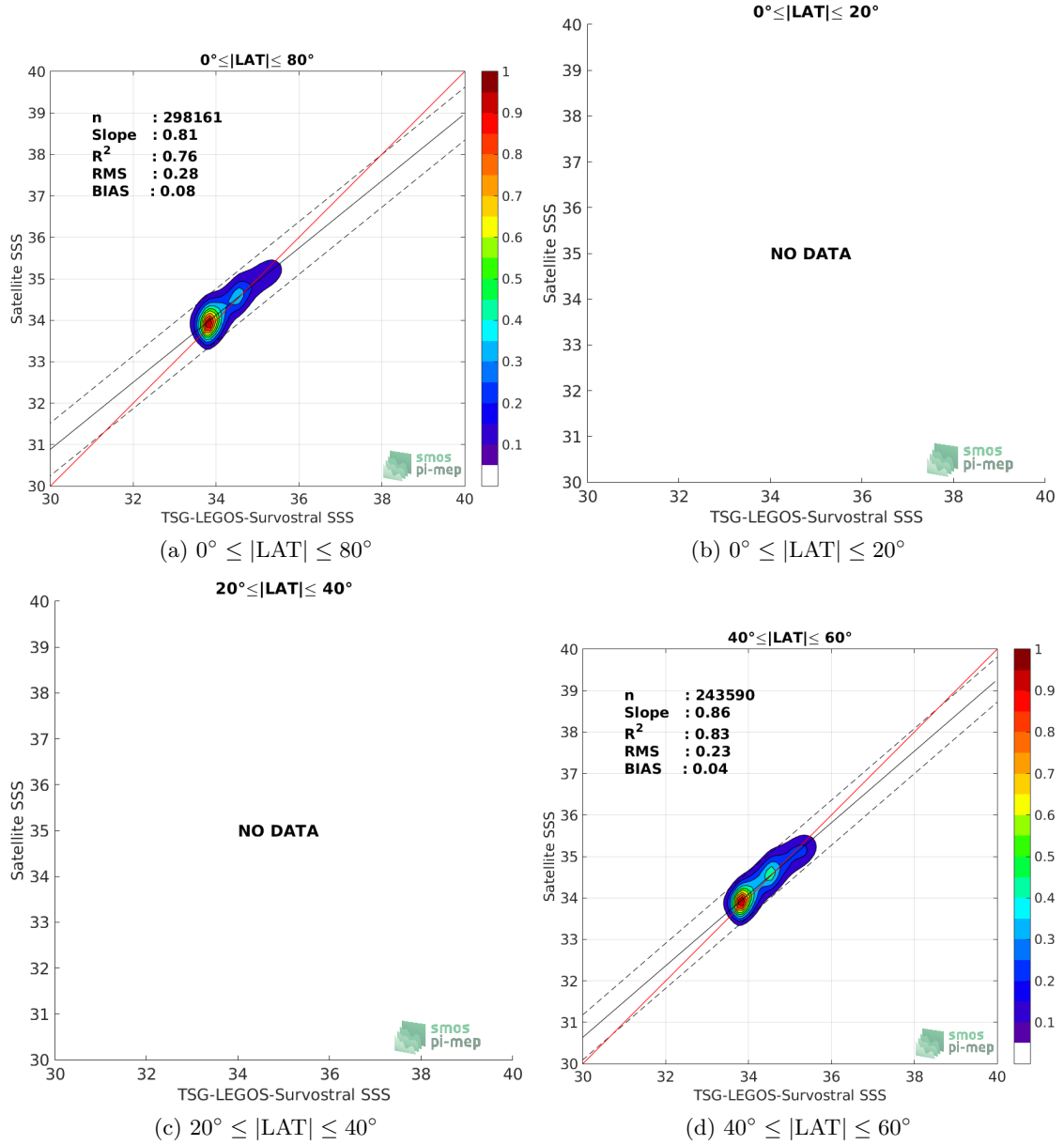
Figure 9: Contour maps of the concentration of SMOS-L3-CATDS-CECOS-LOCEAN-V3-18DAYS-25KM SSS (y-axis) versus TSG-LEGOS-Survostral SSS (x-axis) at match-up pairs for different latitude bands. For each plot, the red line shows x=y . The black thin and dashed lines indicate a linear fit through the data cloud and the \pm 95\% confidence levels, respectively. The number match-up pairs n , the slope and R^2 coefficient of the linear fit, the root mean square (RMS) and the mean bias between satellite and in situ data are indicated for each latitude band in each plots.
