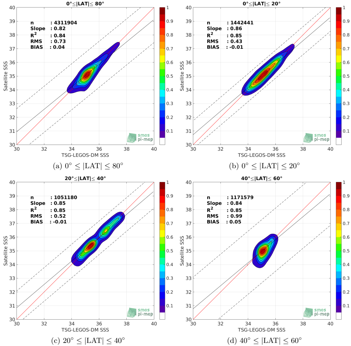
Figure 9: Contour maps of the concentration of SMOS-L3-CATDS-CECOS-LOCEAN-V3-18DAYS-25KM SSS (y-axis) versus TSG-LEGOS-DM SSS (x-axis) at match-up pairs for different latitude bands. For each plot, the red line shows x=y . The black thin and dashed lines indicate a linear fit through the data cloud and the \pm 95\% confidence levels, respectively. The number match-up pairs n , the slope and R^2 coefficient of the linear fit, the root mean square (RMS) and the mean bias between satellite and in situ data are indicated for each latitude band in each plots.
