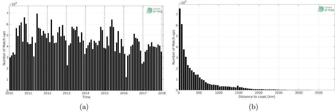
Figure 1: Number of match-ups between TSG-LEGOS-DM and SMOS-L3-CATDS-CECOS-LOCEAN-V3-18DAYS-25KM SSS as a function of time (a) and as function of the distance to coast (b) over the Global Ocean Pi-MEP region and for the full satellite product period.
