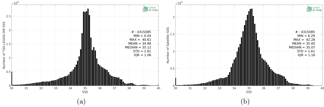
Figure 2: Histograms of SSS from TSG-LEGOS-DM (a) and SMOS-L3-CATDS-CECOS-LOCEAN-V3-18DAYS-25KM (b) considering all match-up pairs per bins of 0.1 over the Global Ocean Pi-MEP region and for the full satellite product period.
