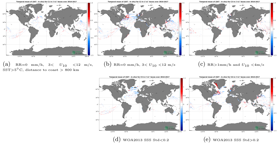
Figure 12: Temporal mean gridded over spatial boxes of size 1^\circ \times 1^\circ of \Delta SSS (SMOS-L3-CATDS-CECOS-LOCEAN-V3-18DAYS-25KM - TSG-LEGOS-DM) for 5 different subdatasets corresponding to: RR=0 mm/h, 3 < U_{10} < 12 m/s, SST > 5^\circ C , distance to coast > 800 km (a), RR=0 mm/h, 3 < U_{10} < 12 m/s (b), RR > 1 mm/h and U_{10} < 4 m/s (c), WOA2013 SSS Std < 0.2 (d), WOA2013 SSS Std > 0.2 (e).
