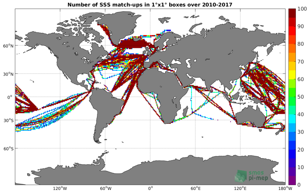
Figure 4: Number of SSS match-ups between TSG-LEGOS-DM SSS and the SMOS-L3-CATDS-CECOS-LOCEAN-V3-18DAYS-25KM SSS product for the Global Ocean Pi-MEP region over 1°x1° boxes and for the full satellite product period.
