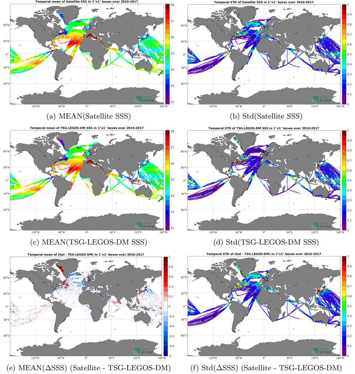
Figure 6: Temporal mean (left) and Std (right) of SSS from SMOS-L3-CATDS-CECOS-LOCEAN-V3-18DAYS-25KM (top), TSG-LEGOS-DM (middle), and of \Delta SSS (Satellite - TSG-LEGOS-DM). Only match-up pairs are used to generate these maps.
