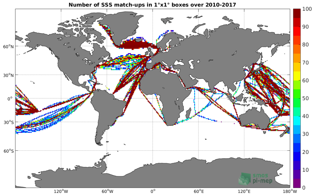
Figure 4: Number of SSS match-ups between TSG-LEGOS-DM SSS and the SMOS-L3-CATDS-CECOS-LOCEAN-V3-18DAYS-25KM SSS product for the Global Ocean Pi-MEP region over 1^\circ \times 1^\circ boxes and for the full satellite product period.
