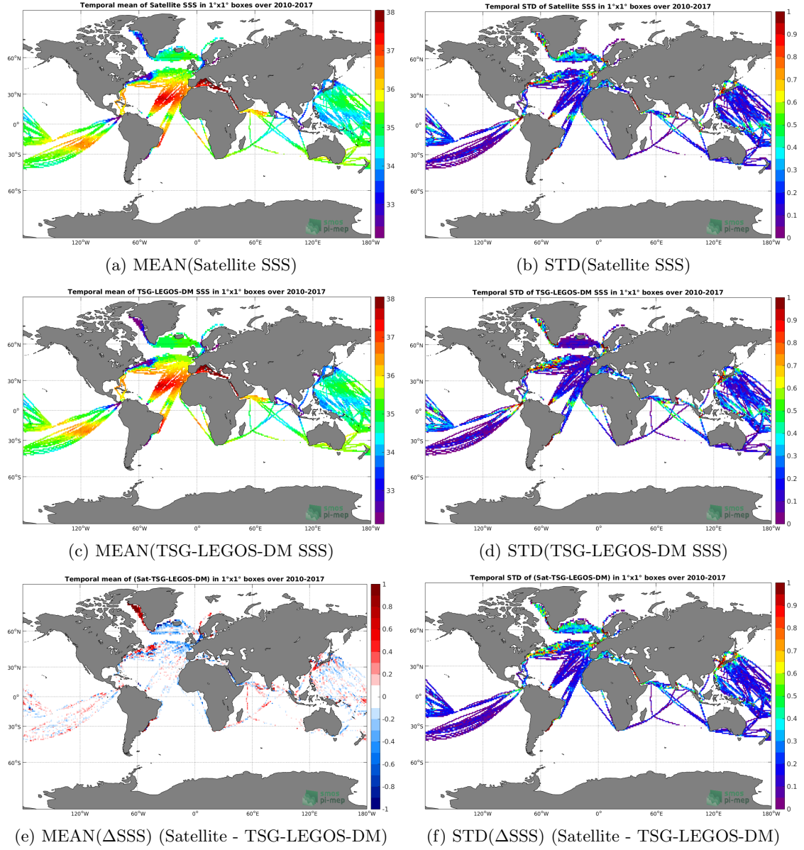
Figure 6: Temporal mean (left) and STD (right) of SSS from SMOS-L3-CATDS-CECOS-LOCEAN-V3-18DAYS-25KM (top), TSG-LEGOS-DM (middle), and of ΔSSS (Satellite - TSG-LEGOS-DM). Only match-up pairs are used to generate these maps.
