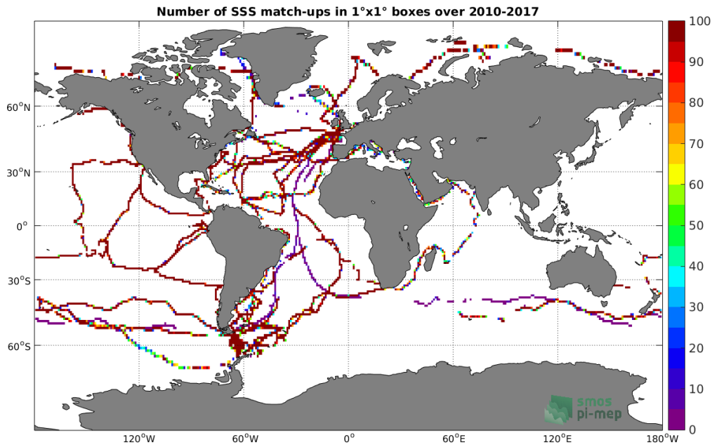
Figure 4: Number of SSS match-ups between TSG-GOSUD-Sailing-ship SSS and the SMOS-L3-CATDS-CECOS-LOCEAN-V3-18DAYS-25KM SSS product for the Global Ocean Pi-MEP region over 1°x1° boxes and for the full satellite product period.
