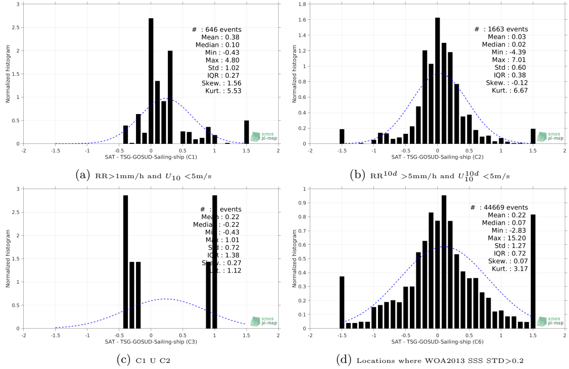
Figure 13: Normalized histogram of \Delta SSS (SMOS-L3-CATDS-CECOS-LOCEAN-V3-18DAYS-25KM - TSG-GOSUD-Sailing-ship) for 6 different subdatasets corresponding to: RR > 1mm/h and U_{10} < 5 m/s (a), RR^{10d} > 5 mm/h and U_{10}^{10d} < 5 m/s (b), C1 U C2 (c), Locations where WOA2013 SSS STD > 0.2 (d).
