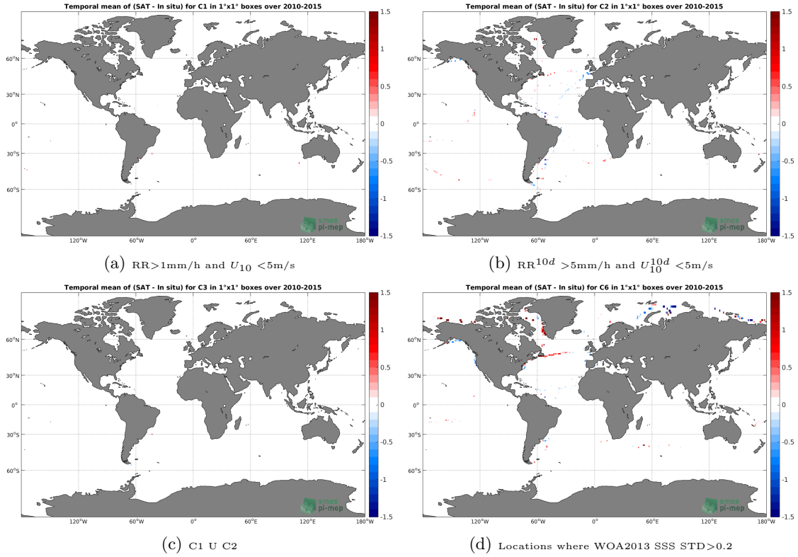
Figure 12: Temporal mean gridded over spatial boxes of size 1^\circ \times 1^\circ of \Delta SSS (SMOS-L3-CATDS-CECOS-LOCEAN-V3-18DAYS-25KM - TSG-GOSUD-Sailing-ship) for 4 different subdatasets corresponding to: RR > 1\text{mm/h} and U_{10} < 5\text{m/s} (a), RR^{10d} > 5\text{mm/h} and U_{10}^{10d} < 5\text{m/s} (b), C1 U C2 (c), Locations where WOA2013 SSS STD > 0.2 (d).
