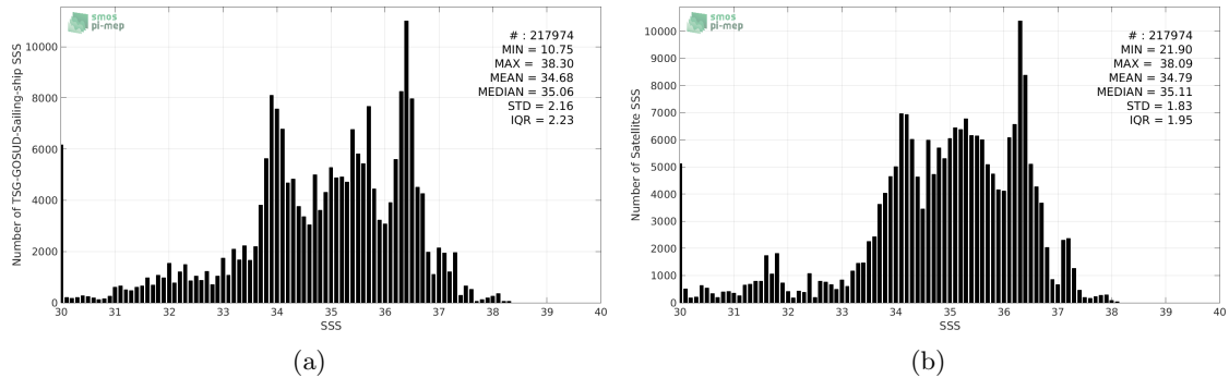
Figure 2: Histograms of SSS from TSG-GOSUD-Sailing-ship (a) and SMOS-L3-CATDS-CECOS-LOCEAN-V3-18DAYS-25KM (b) considering all match-up pairs per bins of 0.1 over the Global Ocean Pi-MEP region and for the full satellite product period.
