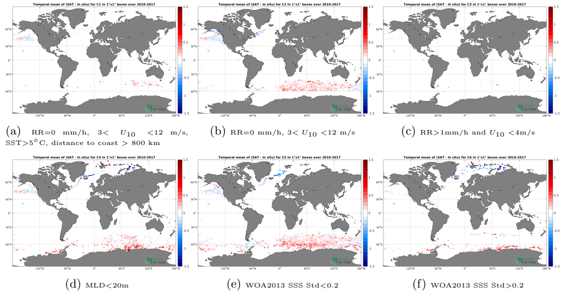
Figure 12: Temporal mean gridded over spatial boxes of size 1^\circ \times 1^\circ of \Delta SSS (SMOS-L3-CATDS-CECOS-LOCEAN-V3-18DAYS-25KM - Sea mammals) for 6 different subdatasets corresponding to: RR=0 mm/h, 3 < U_{10} < 12 m/s, SST >5^\circ C, distance to coast > 800 km (a), RR=0 mm/h, 3 < U_{10} < 12 m/s (b), RR >1 mm/h and U_{10} < 4 m/s (c),MLD <20 m (d),WOA2013 SSS Std <0.2 (e),WOA2013 SSS Std >0.2 (f).
