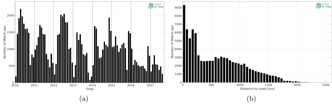
Figure 1: Number of match-ups between Sea mammals and SMOS-L3-CATDS-CECOS-LOCEAN-V3-18DAYS-25KM SSS as a function of time (a) and as function of the distance to coast (b) over the Global Ocean Pi-MEP region and for the full satellite product period.
