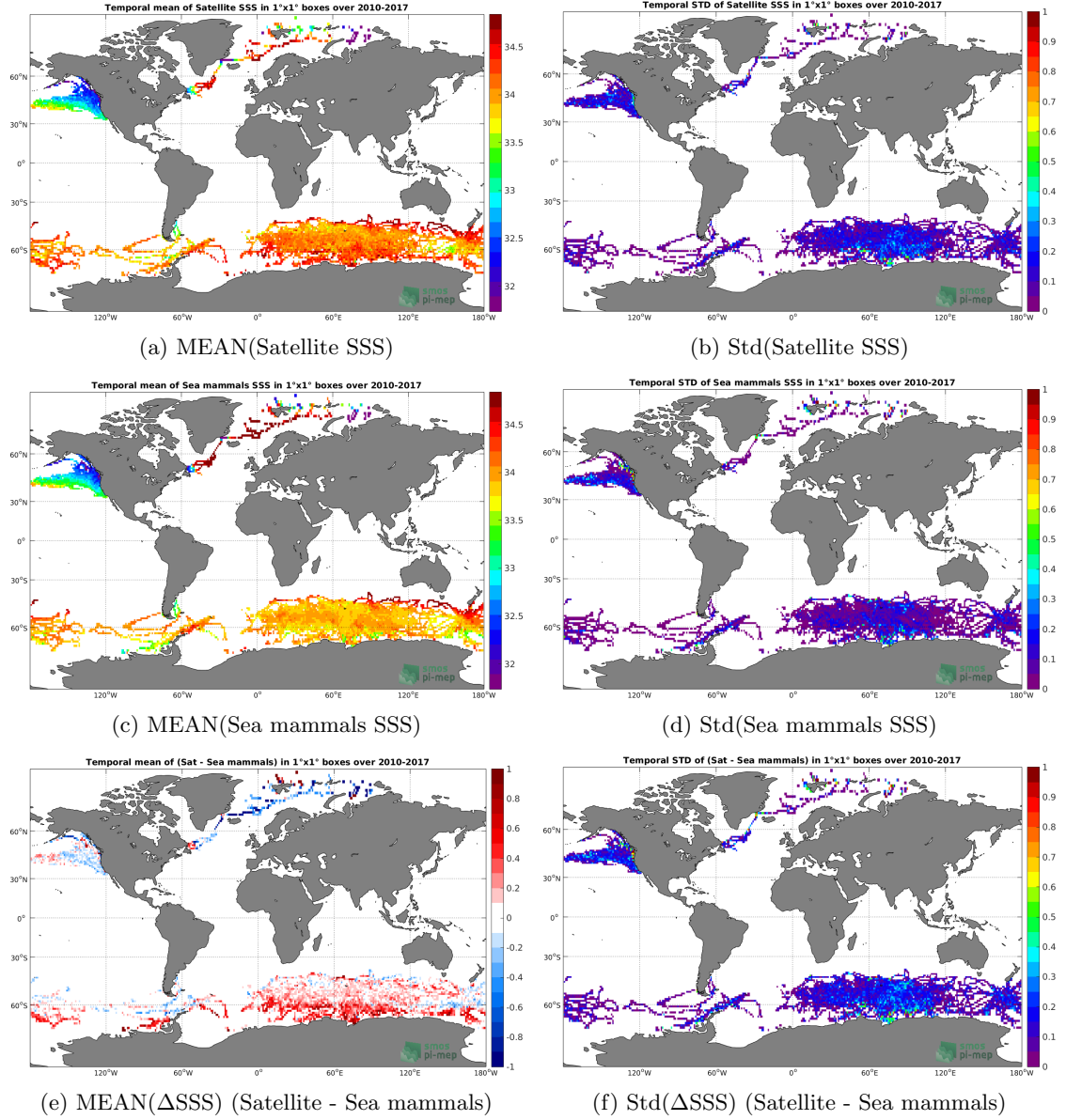
Figure 6: Temporal mean (left) and Std (right) of SSS from SMOS-L3-CATDS-CECOS-LOCEAN-V3-18DAYS-25KM (top), Sea mammals (middle), and of \Delta SSS (Satellite - Sea mammals). Only match-up pairs are used to generate these maps.
