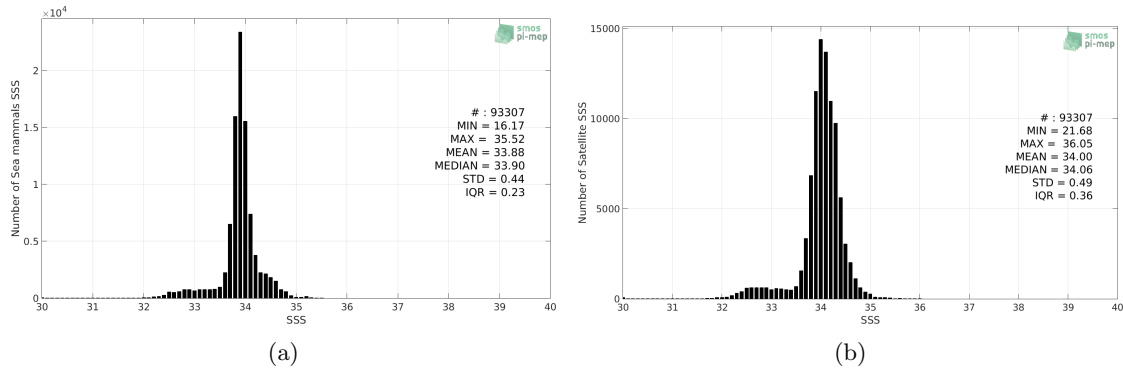
Figure 2: Histograms of SSS from Sea mammals (a) and SMOS-L3-CATDS-CECOS-LOCEAN-V3-18DAYS-25KM (b) considering all match-up pairs per bins of 0.1 over the Global Ocean Pi-MEP region and for the full satellite product period.
