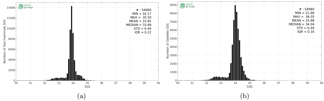
Figure 2: Histograms of SSS from Sea mammals (a) and SMOS-L3-CATDS-CECOS-LOCEAN-V3-18DAYS-25KM (b) considering all match-up pairs per bins of 0.1 over the Global Ocean Pi-MEP region and for the full satellite product period.
