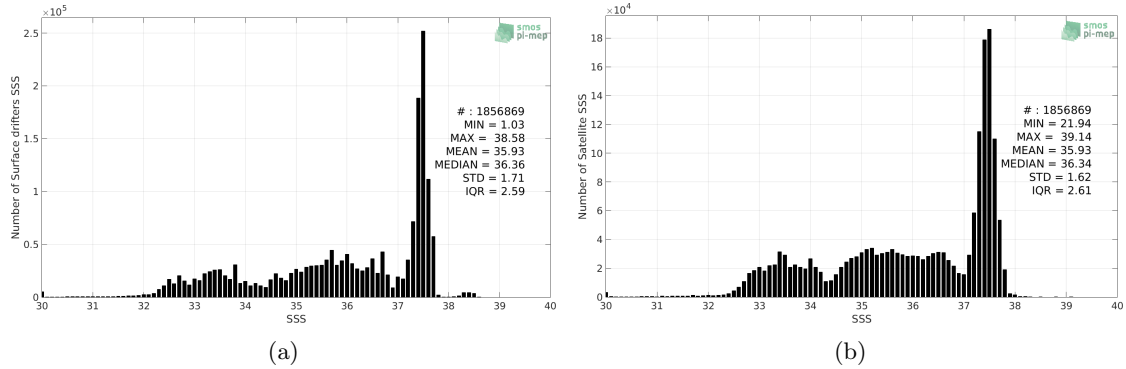
Figure 2: Histograms of SSS from Surface drifters (a) and SMOS-L3-CATDS-CECOS-LOCEAN-V3-18DAYS-25KM (b) considering all match-up pairs per bins of 0.1 over the Global Ocean Pi-MEP region and for the full satellite product period.
