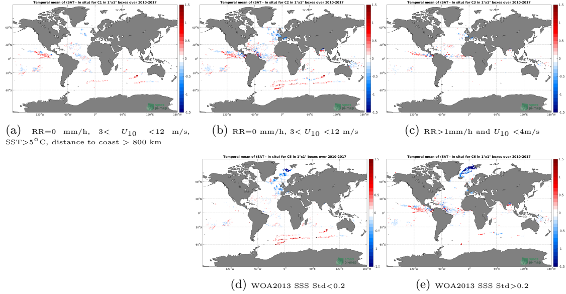
Figure 11: Temporal mean gridded over spatial boxes of size 1^\circ \times 1^\circ of \Delta SSS (SMOS-L3-CATDS-CECOS-LOCEAN-V3-18DAYS-25KM - Surface drifters) for 5 different subdatasets corresponding to: RR=0 mm/h, 3 < U_{10} < 12 m/s, SST >5^\circ C, distance to coast > 800 km (a), RR=0 mm/h, 3 < U_{10} < 12 m/s (b), RR >1 mm/h and U_{10} < 4 m/s (c), WOA2013 SSS Std <0.2 (d), WOA2013 SSS Std >0.2 (e).
