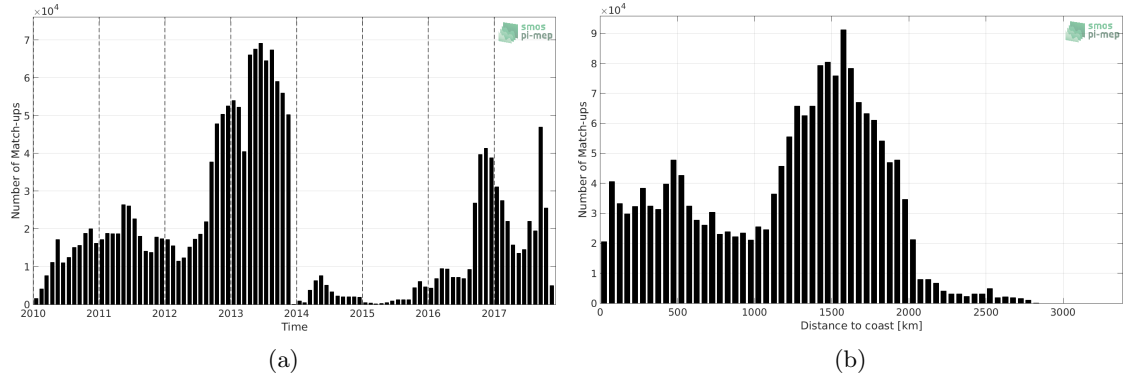
Figure 1: Number of match-ups between Surface drifters and SMOS-L3-CATDS-CECOS-LOCEAN-V3-18DAYS-25KM SSS as a function of time (a) and as function of the distance to coast (b) over the Global Ocean Pi-MEP region and for the full satellite product period.
