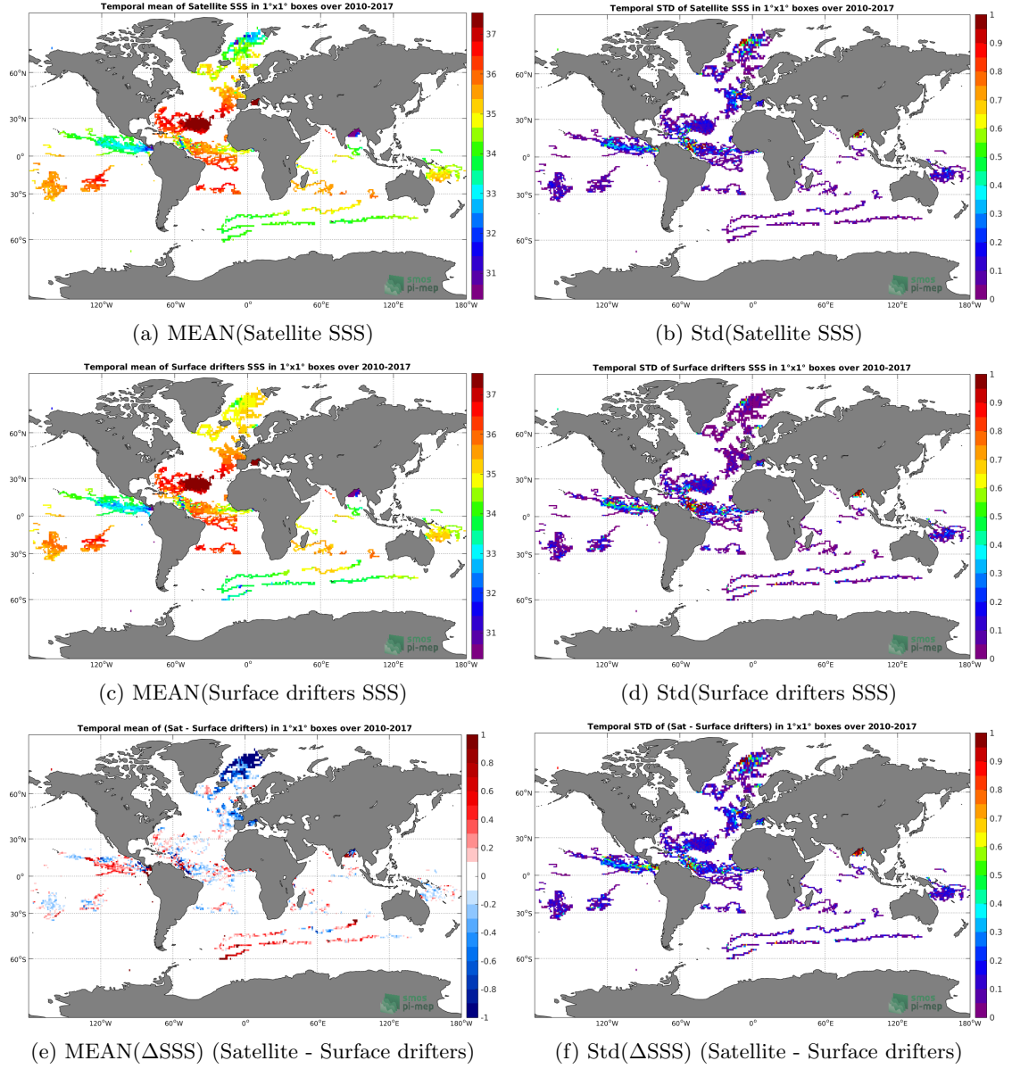
Figure 5: Temporal mean (left) and Std (right) of SSS from SMOS-L3-CATDS-CECOS-LOCEAN-V3-18DAYS-25KM (top), Surface drifters (middle), and of \Delta SSS (Satellite - Surface drifters). Only match-up pairs are used to generate these maps.
