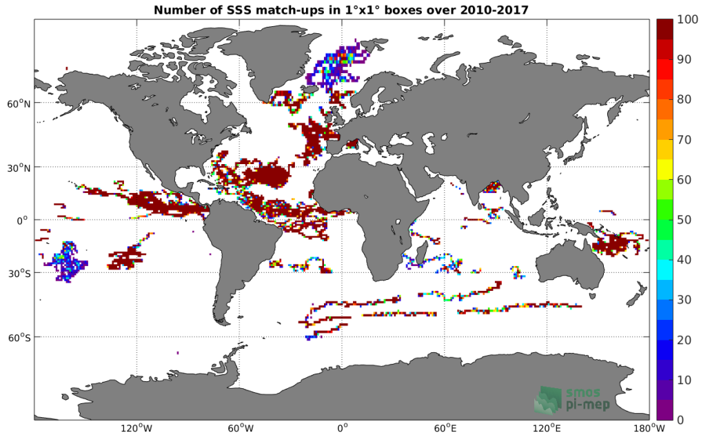
Figure 3: Number of SSS match-ups between Surface drifters SSS and the SMOS-L3-CATDS-CECOS-LOCEAN-V3-18DAYS-25KM SSS product for the Global Ocean Pi-MEP region over 1^\circ \times 1^\circ boxes and for the full satellite product period.
