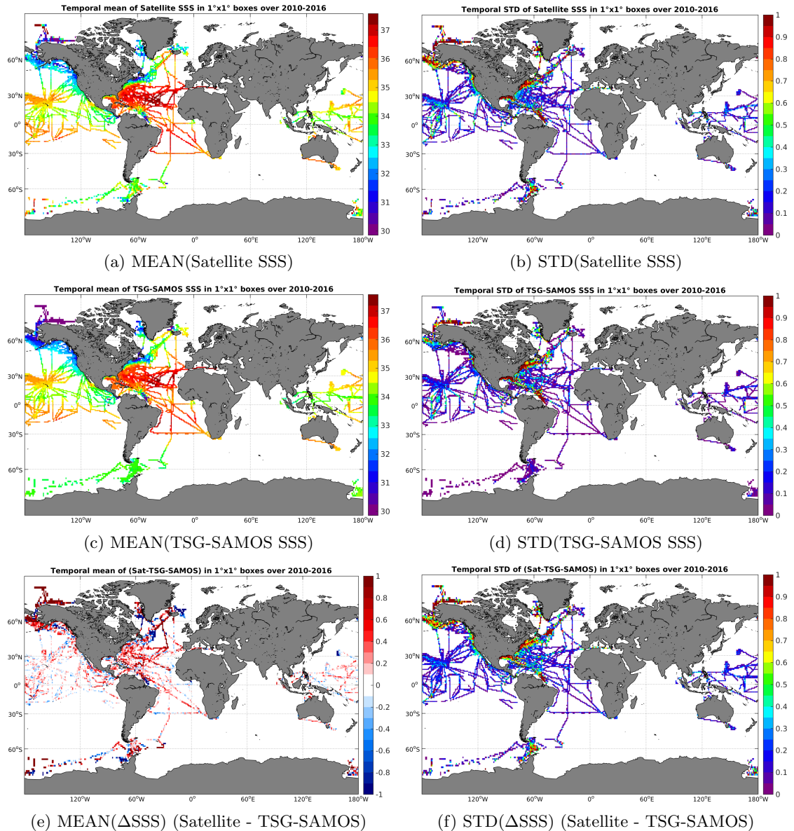
Figure 6: Temporal mean (left) and STD (right) of SSS from SMOS-L3-CATDS-CECOS-LOCEAN-V2-9DAYS-25KM (top), TSG-SAMOS (middle), and of \Delta SSS (Satellite - TSG-SAMOS). Only match-up pairs are used to generate these maps.
