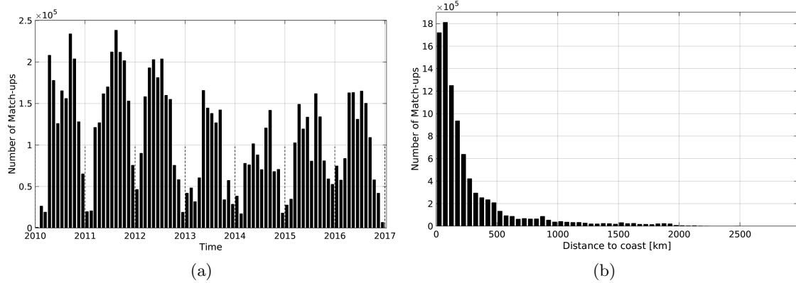
Figure 1: Number of match-ups between TSG-SAMOS and SMOS-L3-CATDS-CECOS-LOCEAN-V2-9DAYS-25KM SSS as a function of time (a) and as function of the distance to coast (b) over the Global Ocean Pi-MEP region and for the full satellite product period.
