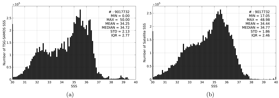
Figure 2: Histograms of SSS from TSG-SAMOS (a) and SMOS-L3-CATDS-CECOS-LOCEAN-V2-9DAYS-25KM (b) considering all match-up pairs per bins of 0.1 over the Global Ocean Pi-MEP region and for the full satellite product period.
