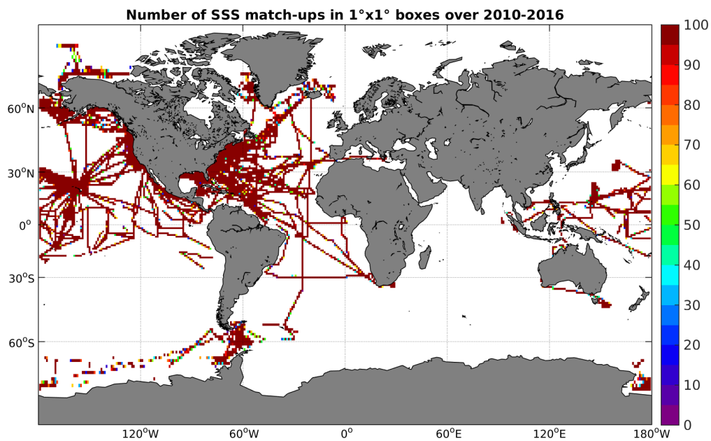
Figure 4: Number of SSS match-ups between TSG-SAMOS SSS and the SMOS-L3-CATDS-CECOS-LOCEAN-V2-9DAYS-25KM SSS product for the Global Ocean Pi-MEP region over 1°x1° boxes and for the full satellite product period.
