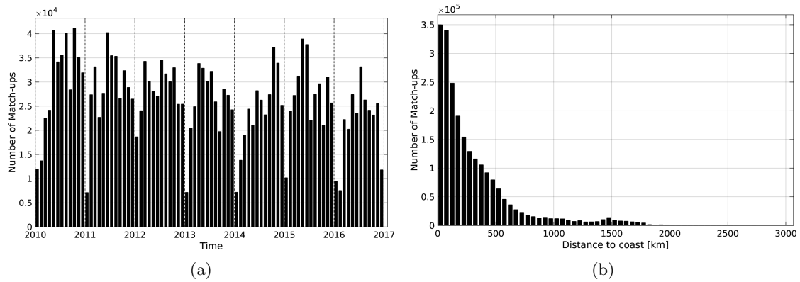
Figure 1: Number of match-ups between TSG-LEGOS-DM and SMOS-L3-CATDS-CECOS-LOCEAN-V2-9DAYS-25KM SSS as a function of time (a) and as function of the distance to coast (b) over the Global Ocean Pi-MEP region and for the full satellite product period.
