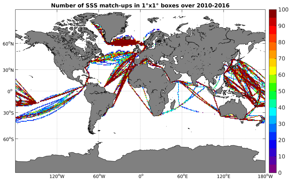
Figure 4: Number of SSS match-ups between TSG-LEGOS-DM SSS and the SMOS-L3-CATDS-CECOS-LOCEAN-V2-9DAYS-25KM SSS product for the Global Ocean Pi-MEP region over 1^\circ \times 1^\circ boxes and for the full satellite product period.
