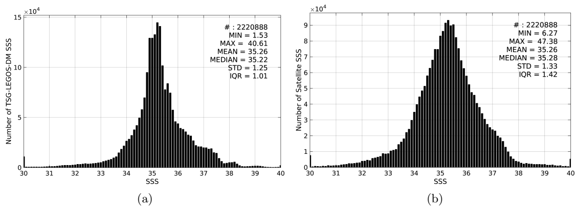
Figure 2: Histograms of SSS from TSG-LEGOS-DM (a) and SMOS-L3-CATDS-CECOS-LOCEAN-V2-9DAYS-25KM (b) considering all match-up pairs per bins of 0.1 over the Global Ocean Pi-MEP region and for the full satellite product period.
