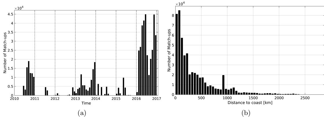
Figure 1: Number of match-ups between TSG-GOSUD-Sailing-ship and SMOS-L3-CATDS-CECOS-LOCEAN-V2-9DAYS-25KM SSS as a function of time (a) and as function of the distance to coast (b) over the Global Ocean Pi-MEP region and for the full satellite product period.
