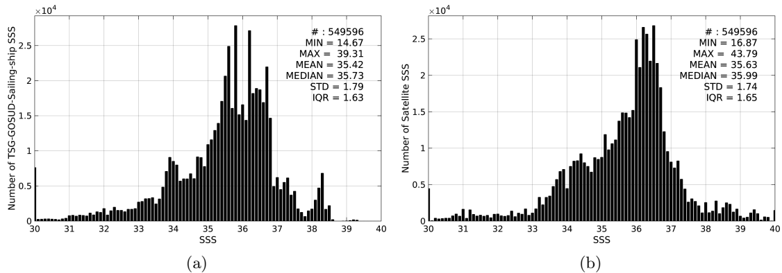
Figure 2: Histograms of SSS from TSG-GOSUD-Sailing-ship (a) and SMOS-L3-CATDS-CECOS-LOCEAN-V2-9DAYS-25KM (b) considering all match-up pairs per bins of 0.1 over the Global Ocean Pi-MEP region and for the full satellite product period.
