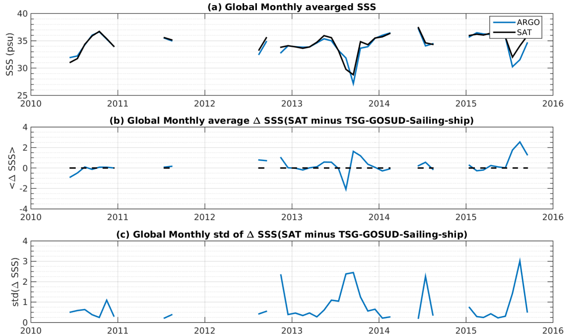
Figure 7: Time series of the monthly averaged mean SSS (top), mean \Delta SSS (Satellite - TSG-GOSUD-Sailing-ship) and STD of \Delta SSS (Satellite - TSG-GOSUD-Sailing-ship) over the Global Ocean Pi-MEP region considering all match-ups collected by the Pi-MEP platform.
