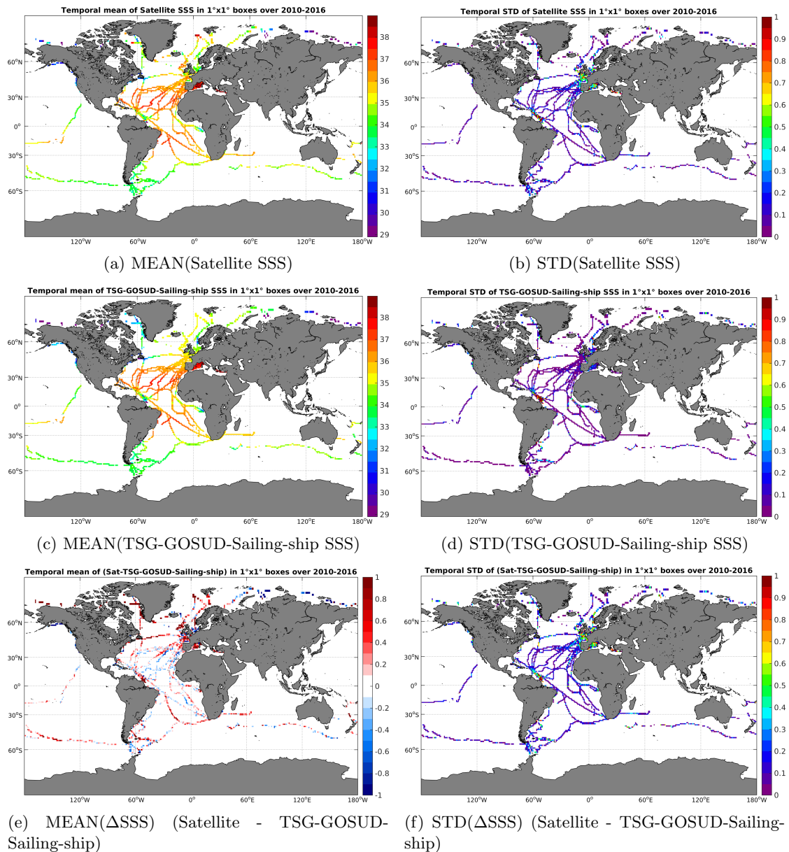
Figure 6: Temporal mean (left) and STD (right) of SSS from SMOS-L3-CATDS-CECOS-LOCEAN-V2-9DAYS-25KM (top), TSG-GOSUD-Sailing-ship (middle), and of \Delta SSS (Satellite - TSG-GOSUD-Sailing-ship). Only match-up pairs are used to generate these maps.
