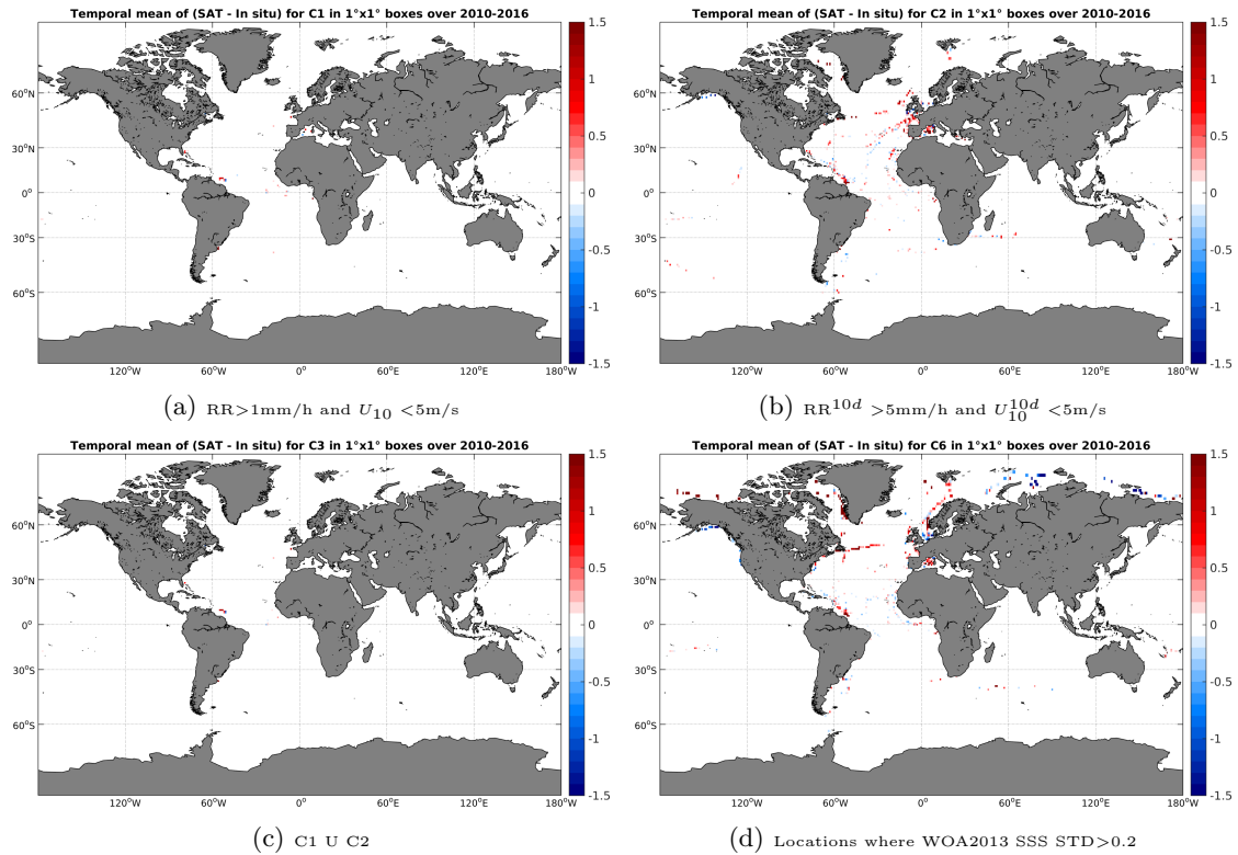
Figure 12: Temporal mean gridded over spatial boxes of size 1^\circ \times 1^\circ of \Delta SSS (SMOS-L3-CATDS-CECOS-LOCEAN-V2-9DAYS-25KM - TSG-GOSUD-Sailing-ship) for 4 different subdatasets corresponding to: RR > 1\text{mm/h} and U_{10} < 5\text{m/s} (a), RR^{10d} > 5\text{mm/h} and U_{10}^{10d} < 5\text{m/s} (b), C1 U C2 (c), Locations where WOA2013 SSS STD > 0.2 (d).
