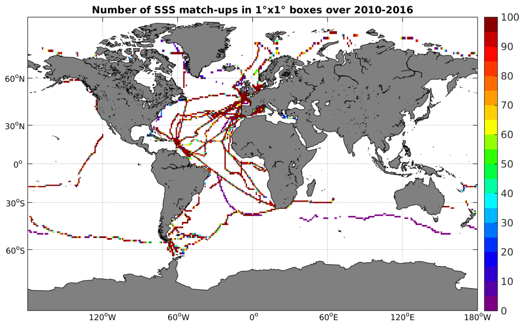
Figure 4: Number of SSS match-ups between TSG-GOSUD-Sailing-ship SSS and the SMOS-L3-CATDS-CECOS-LOCEAN-V2-9DAYS-25KM SSS product for the Global Ocean Pi-MEP region over 1^\circ \times 1^\circ boxes and for the full satellite product period.
