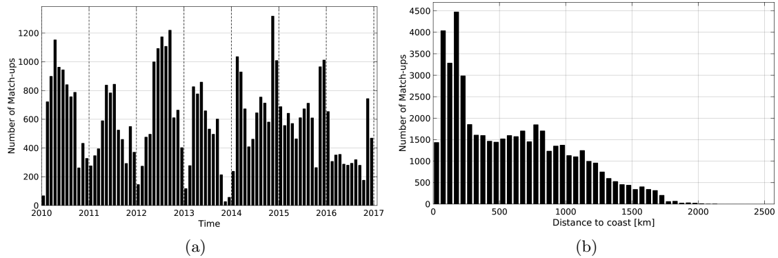
Figure 1: Number of match-ups between Sea mammals and SMOS-L3-CATDS-CECOS-LOCEAN-V2-9DAYS-25KM SSS as a function of time (a) and as function of the distance to coast (b) over the Global Ocean Pi-MEP region and for the full satellite product period.
