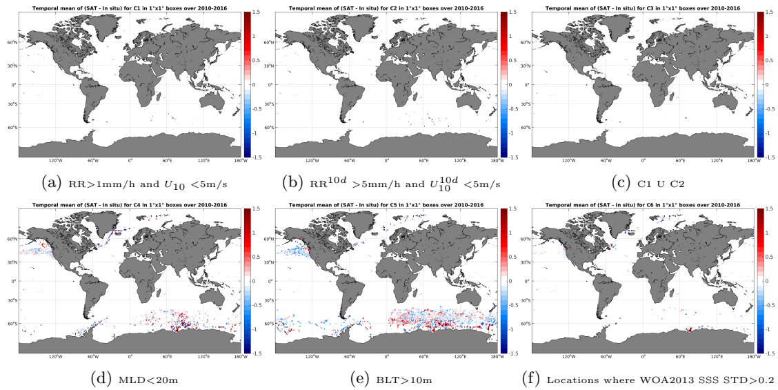
Figure 12: Temporal mean gridded over spatial boxes of size 1^\circ \times 1^\circ of \Delta SSS (SMOS-L3-CATDS-CECOS-LOCEAN-V2-9DAYS-25KM - Sea mammals) for 6 different subdatasets corresponding to: RR > 1\text{mm/h} and U_{10} < 5\text{m/s} (a), RR^{10d} > 5\text{mm/h} and U_{10}^{10d} < 5\text{m/s} (b), C1 U C2 (c), MLD < 20\text{m} (d), BLT > 10\text{m} (e), Locations where WOA2013 SSS STD > 0.2 (f).
