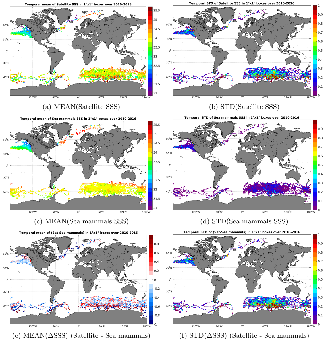
Figure 6: Temporal mean (left) and STD (right) of SSS from SMOS-L3-CATDS-CECOS-LOCEAN-V2-9DAYS-25KM (top), Sea mammals (middle), and of \Delta SSS (Satellite - Sea mammals). Only match-up pairs are used to generate these maps.
