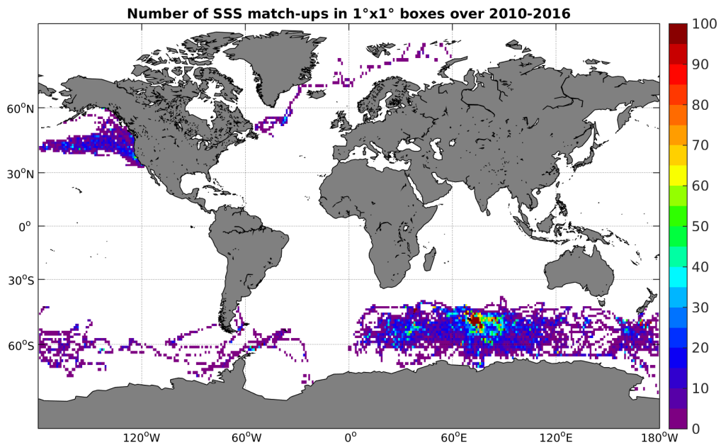
Figure 4: Number of SSS match-ups between Sea mammals SSS and the SMOS-L3-CATDS-CECOS-LOCEAN-V2-9DAYS-25KM SSS product for the Global Ocean Pi-MEP region over 1°x1° boxes and for the full satellite product period.
