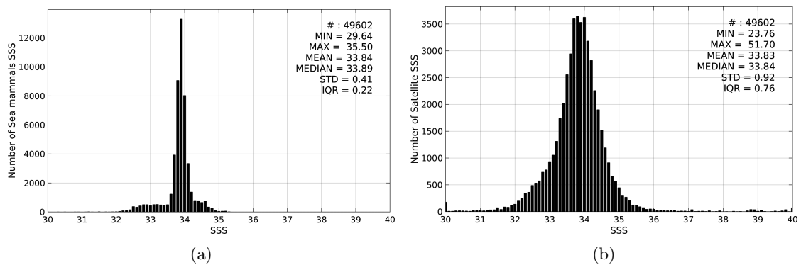
Figure 2: Histograms of SSS from Sea mammals (a) and SMOS-L3-CATDS-CECOS-LOCEAN-V2-9DAYS-25KM (b) considering all match-up pairs per bins of 0.1 over the Global Ocean Pi-MEP region and for the full satellite product period.
