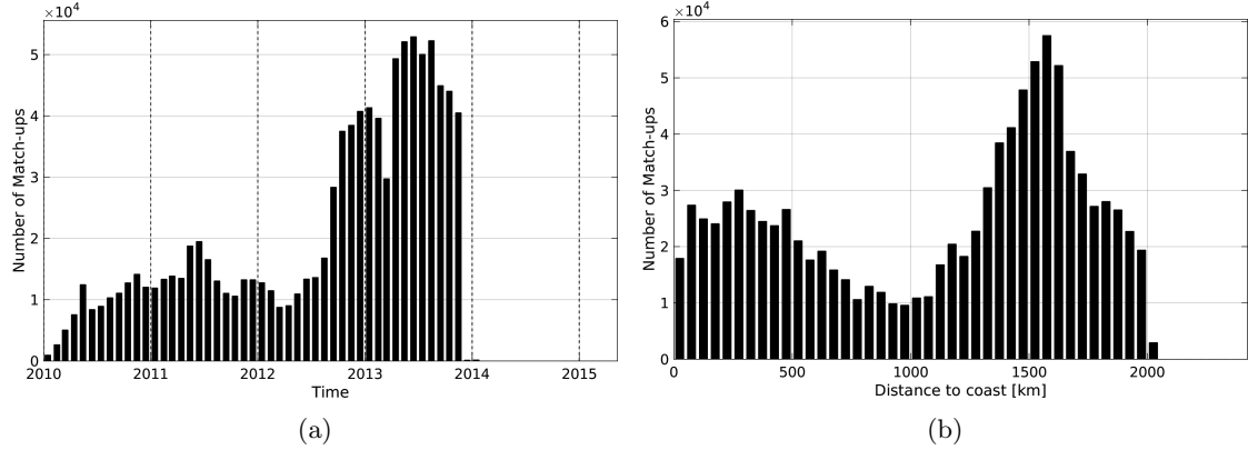
Figure 1: Number of match-ups between Surface drifters and SMOS-L3-CATDS-CECOS-LOCEAN-V2-9DAYS-25KM SSS as a function of time (a) and as function of the distance to coast (b) over the Global Ocean Pi-MEP region and for the full satellite product period.
