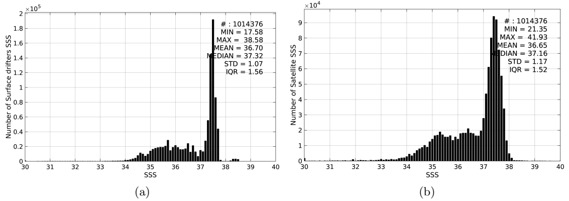
Figure 2: Histograms of SSS from Surface drifters (a) and SMOS-L3-CATDS-CECOS-LOCEAN-V2-9DAYS-25KM (b) considering all match-up pairs per bins of 0.1 over the Global Ocean Pi-MEP region and for the full satellite product period.
