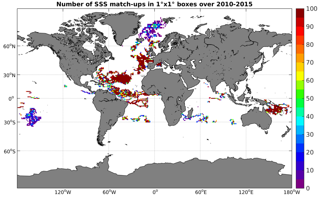
Figure 3: Number of SSS match-ups between Surface drifters SSS and the SMOS-L3-CATDS-CECOS-LOCEAN-V2-9DAYS-25KM SSS product for the Global Ocean Pi-MEP region over 1°x1° boxes and for the full satellite product period.
