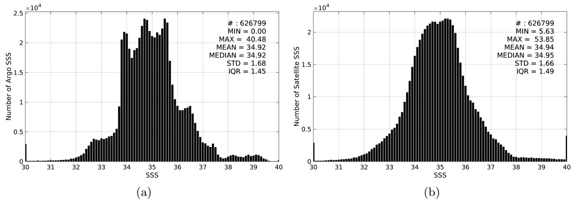
Figure 2: Histograms of SSS from Argo (a) and SMOS-L3-CATDS-CECOS-LOCEAN-V2-9DAYS-25KM (b) considering all match-up pairs per bins of 0.1 over the Global Ocean Pi-MEP region and for the full satellite product period.
