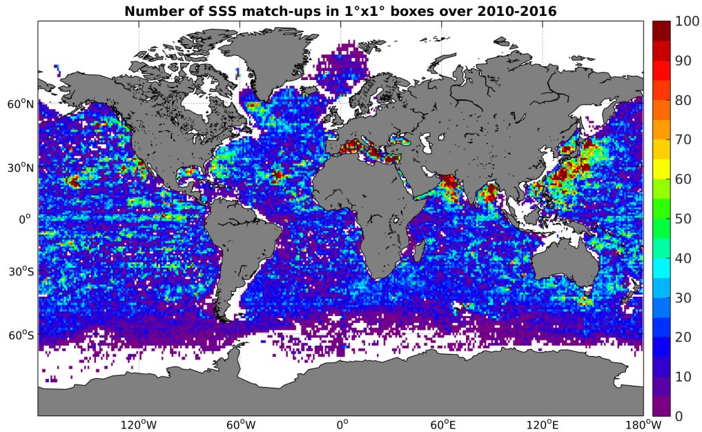
Figure 4: Number of SSS match-ups between Argo SSS and the SMOS-L3-CATDS-CECOS-LOCEAN-V2-9DAYS-25KM SSS product for the Global Ocean Pi-MEP region over 1^\circ \times 1^\circ boxes and for the full satellite product period.
