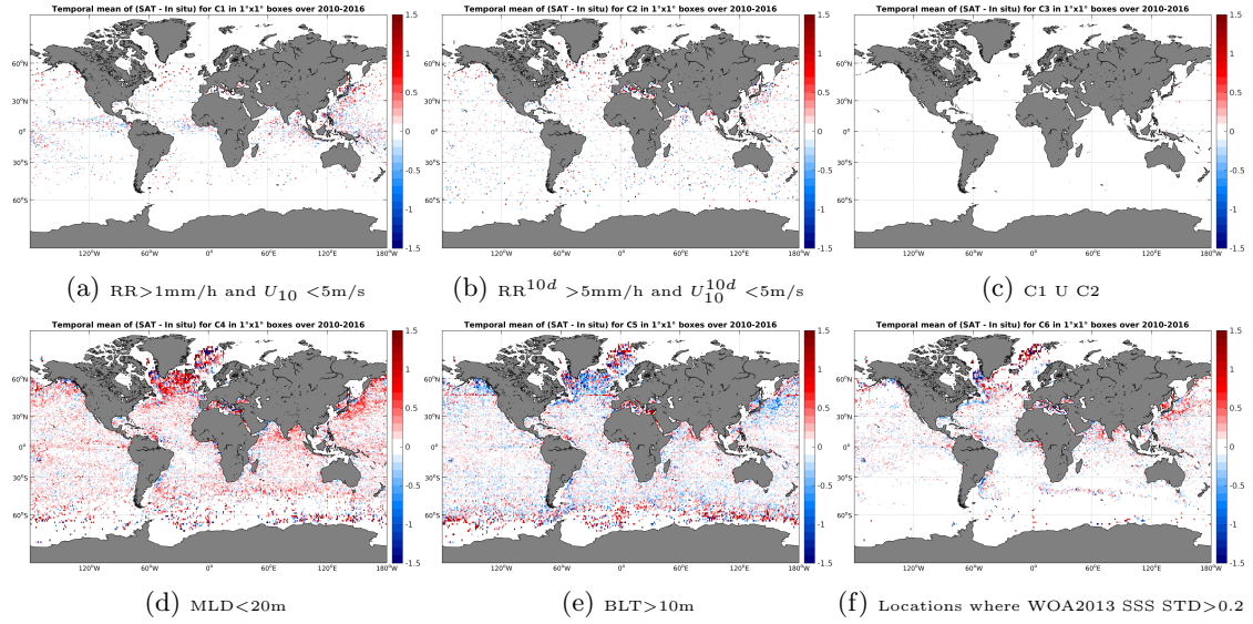
Figure 12: Temporal mean gridded over spatial boxes of size 1^\circ \times 1^\circ of \Delta SSS (SMOS-L3-CATDS-CECOS-LOCEAN-V2-9DAYS-25KM - Argo) for 6 different subdatasets corresponding to: RR > 1\text{mm/h} and U_{10} < 5\text{m/s} (a), RR^{10d} > 5\text{mm/h} and U_{10}^{10d} < 5\text{m/s} (b), C1 U C2 (c), MLD < 20\text{m} (d), BLT > 10\text{m} (e), Locations where WOA2013 SSS STD > 0.2 (f).
