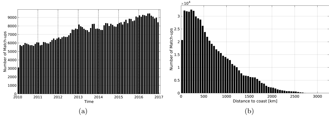
Figure 1: Number of match-ups between Argo and SMOS-L3-CATDS-CECOS-LOCEAN-V2-9DAYS-25KM SSS as a function of time (a) and as function of the distance to coast (b) over the Global Ocean Pi-MEP region and for the full satellite product period.
