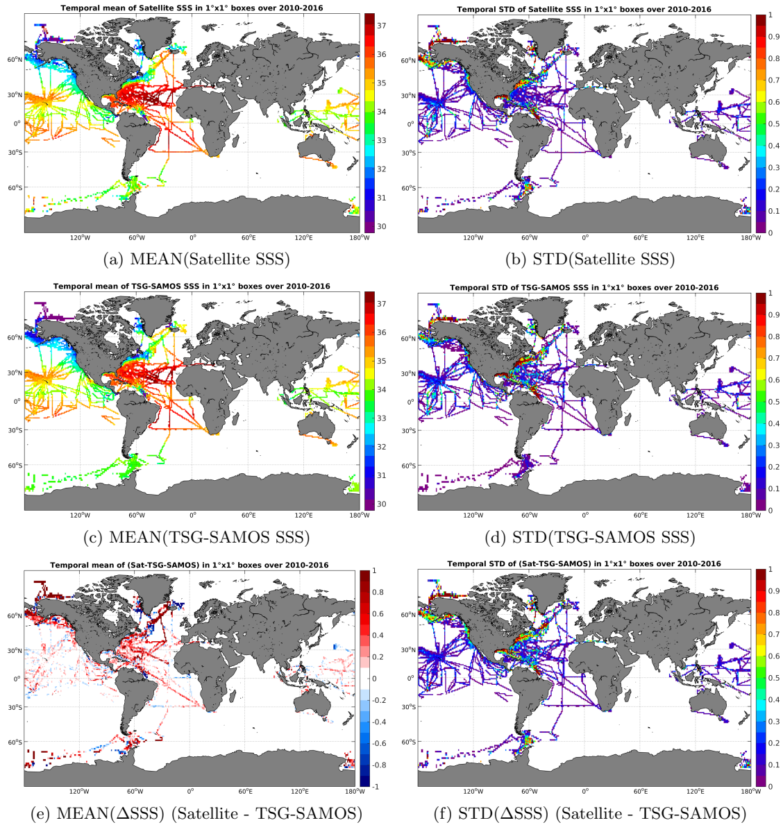
Figure 6: Temporal mean (left) and STD (right) of SSS from SMOS-L3-CATDS-CECOS-LOCEAN-V2-18DAYS-25KM (top), TSG-SAMOS (middle), and of \Delta SSS (Satellite - TSG-SAMOS). Only match-up pairs are used to generate these maps.
