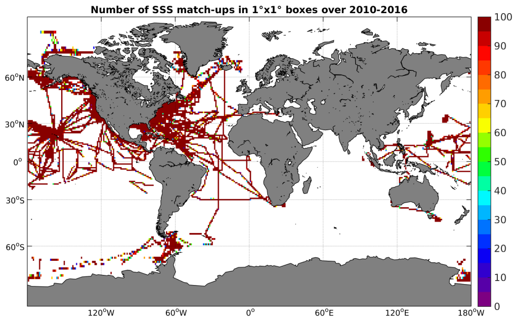
Figure 4: Number of SSS match-ups between TSG-SAMOS SSS and the SMOS-L3-CATDS-CECOS-LOCEAN-V2-18DAYS-25KM SSS product for the Global Ocean Pi-MEP region over 1^\circ \times 1^\circ boxes and for the full satellite product period.
