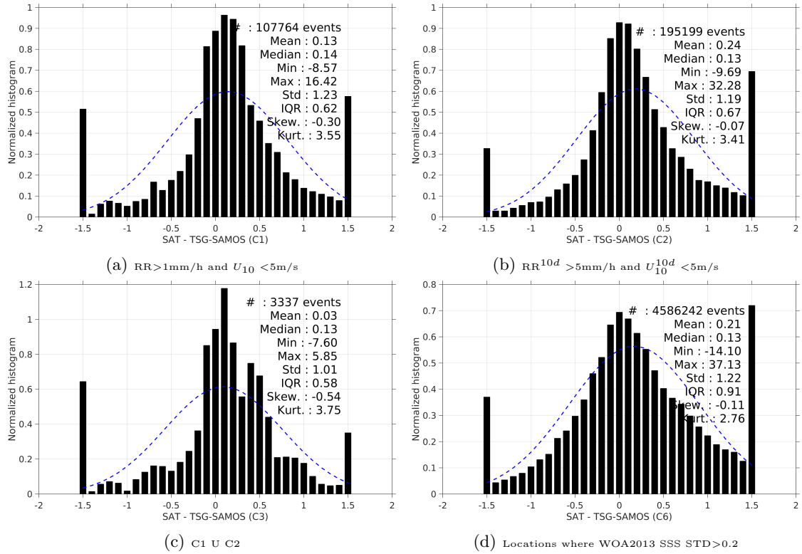
Figure 13: Normalized histogram of \Delta\text{SSS} (SMOS-L3-CATDS-CECOS-LOCEAN-V2-18DAYS-25KM - TSG-SAMOS) for 6 different subdatasets corresponding to: RR > 1\text{mm/h} and U_{10} < 5\text{m/s} (a), RR^{10d} > 5\text{mm/h} and U_{10}^{10d} < 5\text{m/s} (b), C1 U C2 (c), Locations where WOA2013 SSS STD > 0.2 (d).
