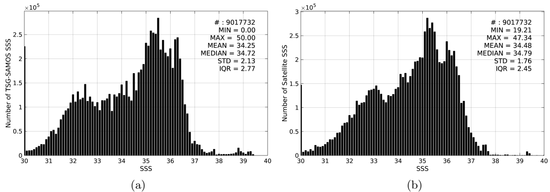
Figure 2: Histograms of SSS from TSG-SAMOS (a) and SMOS-L3-CATDS-CECOS-LOCEAN-V2-18DAYS-25KM (b) considering all match-up pairs per bins of 0.1 over the Global Ocean Pi-MEP region and for the full satellite product period.
