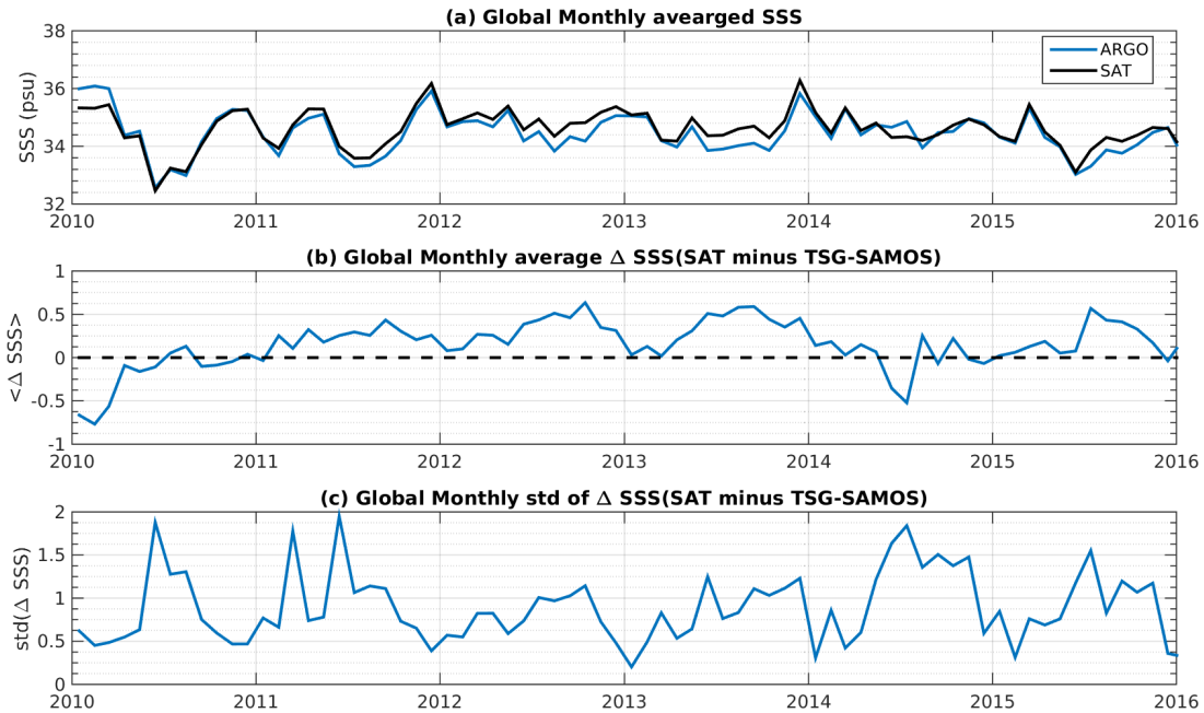
Figure 7: Time series of the monthly averaged mean SSS (top), mean \Delta SSS (Satellite - TSG-SAMOS) and STD of \Delta SSS (Satellite - TSG-SAMOS) over the Global Ocean Pi-MEP region considering all match-ups collected by the Pi-MEP platform.
