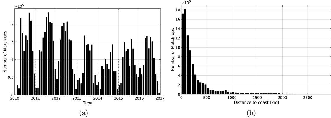
Figure 1: Number of match-ups between TSG-SAMOS and SMOS-L3-CATDS-CECOS-LOCEAN-V2-18DAYS-25KM SSS as a function of time (a) and as function of the distance to coast (b) over the Global Ocean Pi-MEP region and for the full satellite product period.
