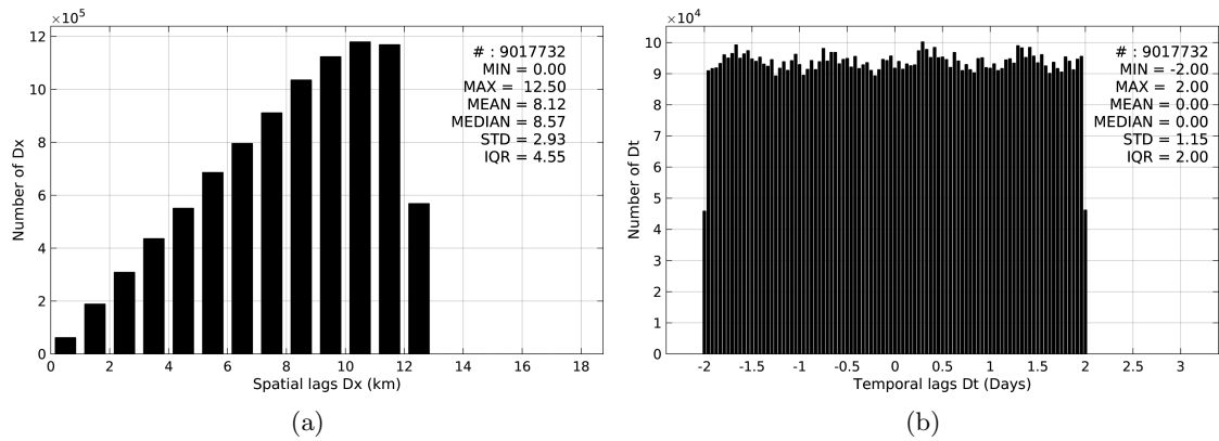
Figure 5: Histograms of the spatial (a) and temporal (b) lags between the time of the TSG-SAMOS measurements and the date of the corresponding SMOS-L3-CATDS-CECOS-LOCEAN-V2-18DAYS-25KM SSS product.
