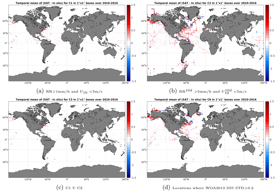
Figure 12: Temporal mean gridded over spatial boxes of size 1^\circ \times 1^\circ of \Delta SSS (SMOS-L3-CATDS-CECOS-LOCEAN-V2-18DAYS-25KM - TSG-SAMOS) for 4 different subdatasets corresponding to: RR > 1\text{mm/h} and U_{10} < 5\text{m/s} (a), RR^{10d} > 5\text{mm/h} and U_{10}^{10d} < 5\text{m/s} (b), C1 U C2 (c), Locations where WOA2013 SSS STD > 0.2 (d).
