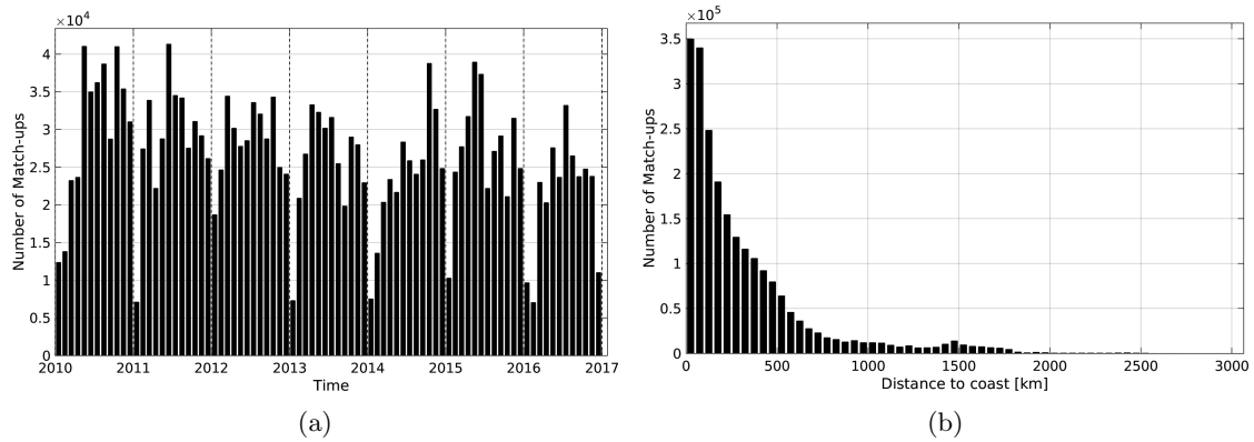
Figure 1: Number of match-ups between TSG-LEGOS-DM and SMOS-L3-CATDS-CECOS-LOCEAN-V2-18DAYS-25KM SSS as a function of time (a) and as function of the distance to coast (b) over the Global Ocean Pi-MEP region and for the full satellite product period.
