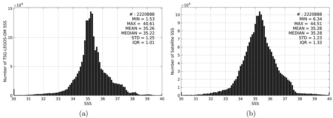
Figure 2: Histograms of SSS from TSG-LEGOS-DM (a) and SMOS-L3-CATDS-CECOS-LOCEAN-V2-18DAYS-25KM (b) considering all match-up pairs per bins of 0.1 over the Global Ocean Pi-MEP region and for the full satellite product period.
