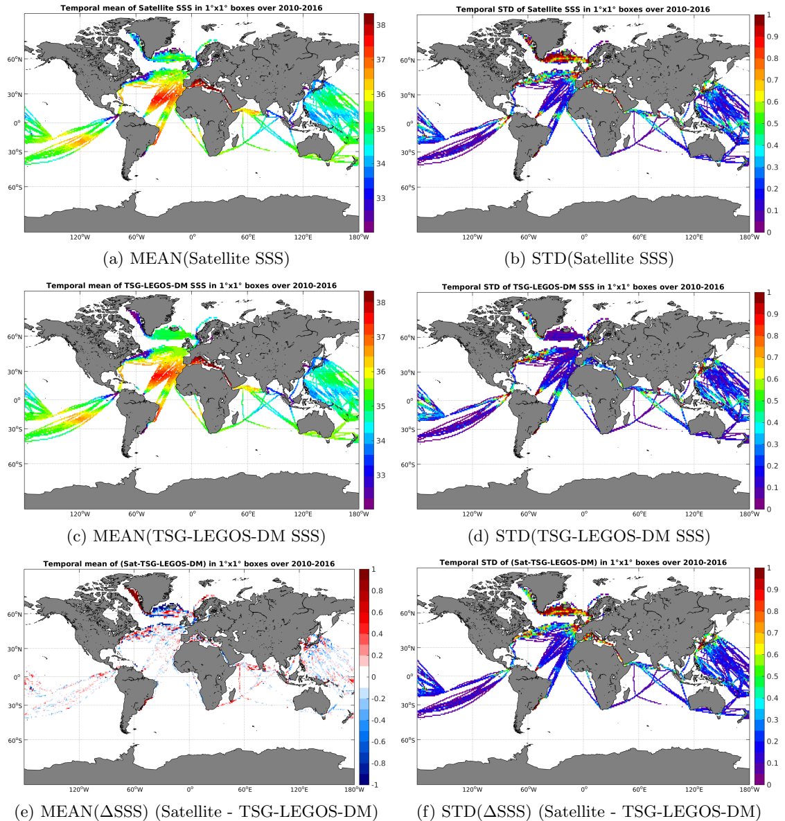
Figure 6: Temporal mean (left) and STD (right) of SSS from SMOS-L3-CATDS-CECOS-LOCEAN-V2-18DAYS-25KM (top), TSG-LEGOS-DM (middle), and of \Delta SSS (Satellite - TSG-LEGOS-DM). Only match-up pairs are used to generate these maps.
