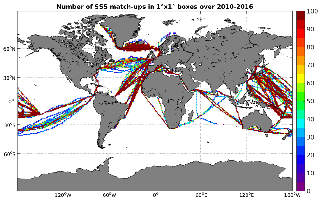
Figure 4: Number of SSS match-ups between TSG-LEGOS-DM SSS and the SMOS-L3-CATDS-CECOS-LOCEAN-V2-18DAYS-25KM SSS product for the Global Ocean Pi-MEP region over 1^\circ \times 1^\circ boxes and for the full satellite product period.
