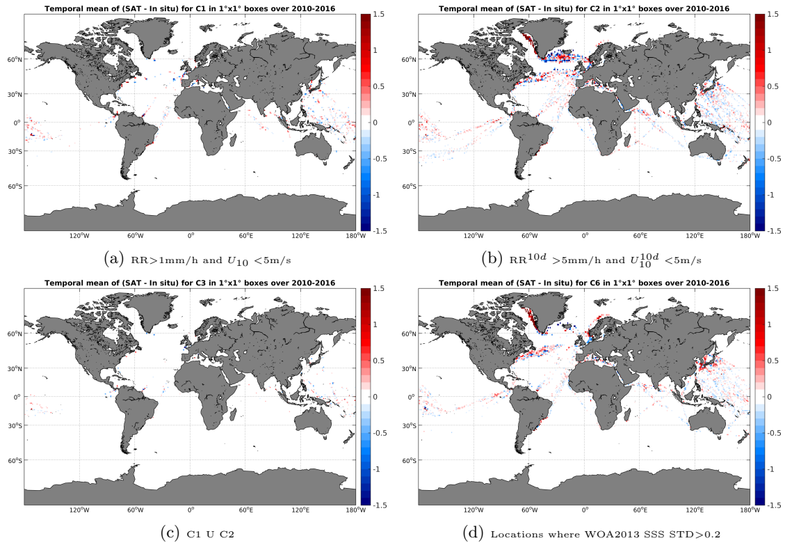
Figure 12: Temporal mean gridded over spatial boxes of size 1^\circ \times 1^\circ of \Delta SSS (SMOS-L3-CATDS-CECOS-LOCEAN-V2-18DAYS-25KM - TSG-LEGOS-DM) for 4 different subdatasets corresponding to:RR>1mm/h and U_{10} < 5 m/s (a), RR^{10d} > 5 mm/h and U_{10}^{10d} < 5 m/s (b), C1 U C2 (c),Locations where WOA2013 SSS STD>0.2 (d).
