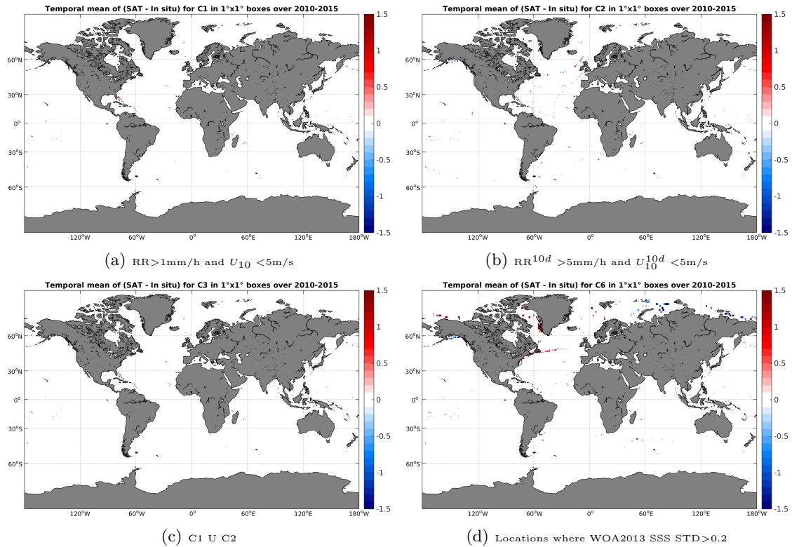
Figure 12: Temporal mean gridded over spatial boxes of size 1^\circ \times 1^\circ of \Delta SSS (SMOS-L3-CATDS-CECOS-LOCEAN-V2-18DAYS-25KM - TSG-GOSUD-Sailing-ship) for 4 different subdatasets corresponding to: RR > 1\text{mm/h} and U_{10} < 5\text{m/s} (a), RR^{10d} > 5\text{mm/h} and U_{10}^{10d} < 5\text{m/s} (b), C1 U C2 (c), Locations where WOA2013 SSS STD > 0.2 (d).
