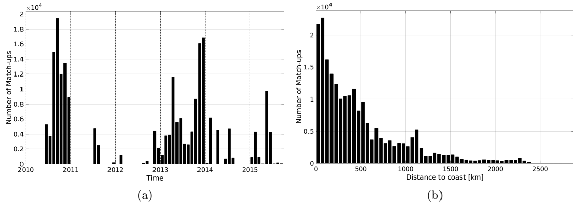
Figure 1: Number of match-ups between TSG-GOSUD-Sailing-ship and SMOS-L3-CATDS-CECOS-LOCEAN-V2-18DAYS-25KM SSS as a function of time (a) and as function of the distance to coast (b) over the Global Ocean Pi-MEP region and for the full satellite product period.
