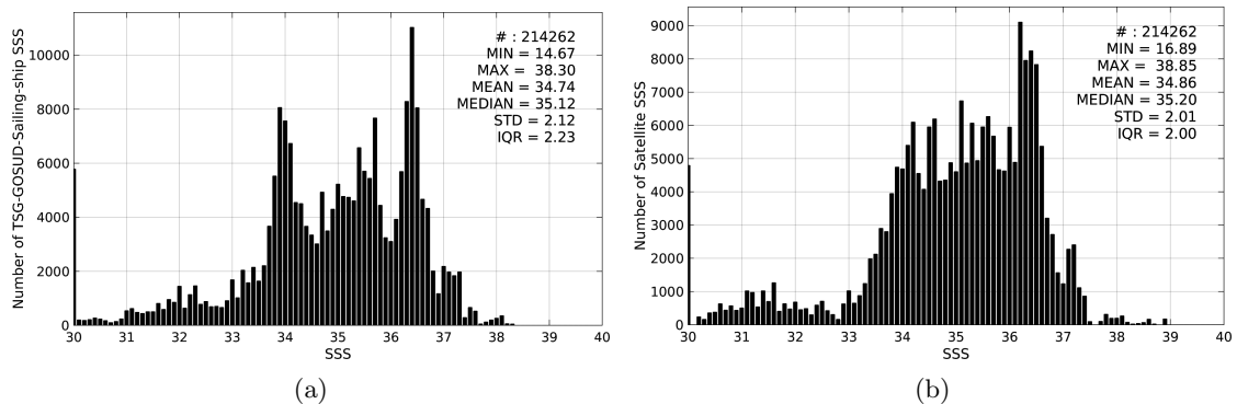
Figure 2: Histograms of SSS from TSG-GOSUD-Sailing-ship (a) and SMOS-L3-CATDS-CECOS-LOCEAN-V2-18DAYS-25KM (b) considering all match-up pairs per bins of 0.1 over the Global Ocean Pi-MEP region and for the full satellite product period.
