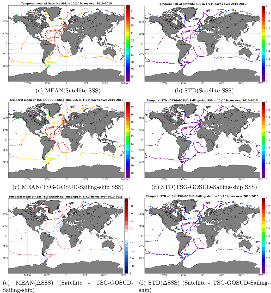
Figure 6: Temporal mean (left) and STD (right) of SSS from SMOS-L3-CATDS-CECOS-LOCEAN-V2-18DAYS-25KM (top), TSG-GOSUD-Sailing-ship (middle), and of \Delta SSS (Satellite - TSG-GOSUD-Sailing-ship). Only match-up pairs are used to generate these maps.
