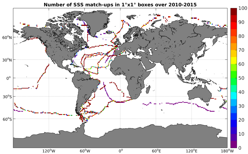
Figure 4: Number of SSS match-ups between TSG-GOSUD-Sailing-ship SSS and the SMOS-L3-CATDS-CECOS-LOCEAN-V2-18DAYS-25KM SSS product for the Global Ocean Pi-MEP region over 1^\circ \times 1^\circ boxes and for the full satellite product period.
