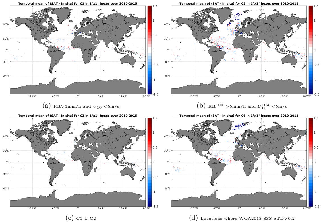
Figure 11: Temporal mean gridded over spatial boxes of size 1^\circ \times 1^\circ of \Delta SSS (SMOS-L3-CATDS-CECOS-LOCEAN-V2-18DAYS-25KM - Surface drifters) for 4 different subdatasets corresponding to: RR > 1\text{mm/h} and U_{10} < 5\text{m/s} (a), RR^{10d} > 5\text{mm/h} and U_{10}^{10d} < 5\text{m/s} (b), C1 U C2 (c), Locations where WOA2013 SSS STD > 0.2 (d).
