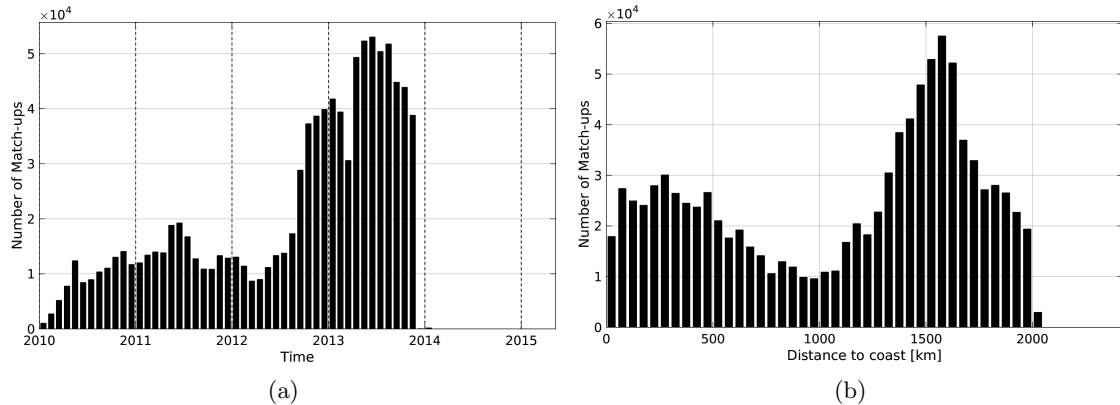
Figure 1: Number of match-ups between Surface drifters and SMOS-L3-CATDS-CECOS-LOCEAN-V2-18DAYS-25KM SSS as a function of time (a) and as function of the distance to coast (b) over the Global Ocean Pi-MEP region and for the full satellite product period.
