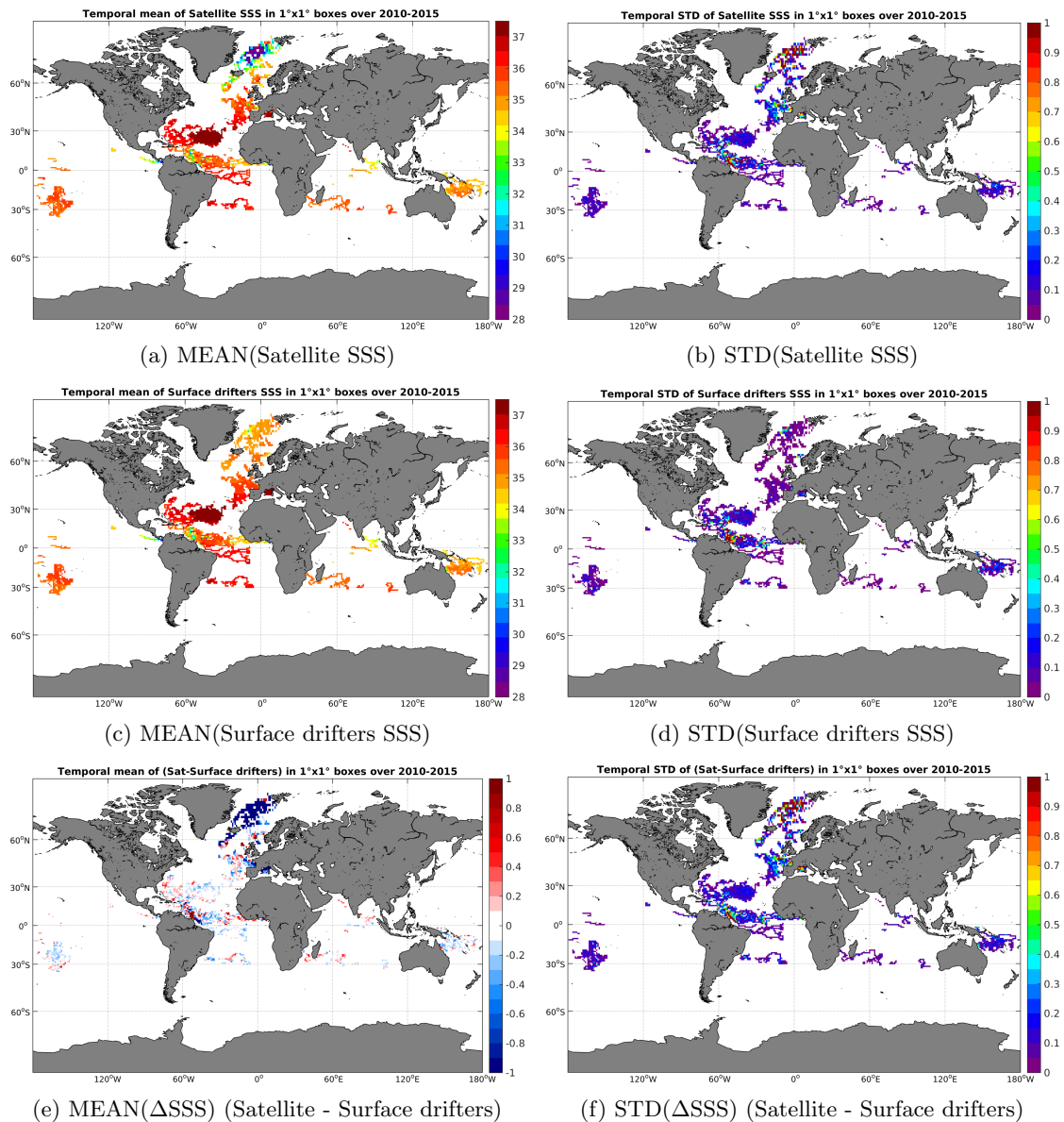
Figure 5: Temporal mean (left) and STD (right) of SSS from SMOS-L3-CATDS-CECOS-LOCEAN-V2-18DAYS-25KM (top), Surface drifters (middle), and of \Delta SSS (Satellite - Surface drifters). Only match-up pairs are used to generate these maps.
