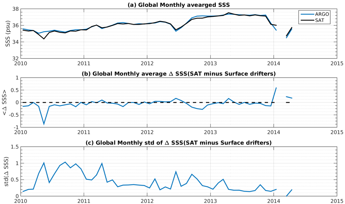
Figure 6: Time series of the monthly averaged mean SSS (top), mean \Delta SSS (Satellite - Surface drifters) and STD of \Delta SSS (Satellite - Surface drifters) over the Global Ocean Pi-MEP region considering all match-ups collected by the Pi-MEP platform.
