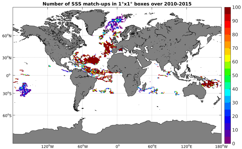
Figure 3: Number of SSS match-ups between Surface drifters SSS and the SMOS-L3-CATDS-CECOS-LOCEAN-V2-18DAYS-25KM SSS product for the Global Ocean Pi-MEP region over 1°x1° boxes and for the full satellite product period.
