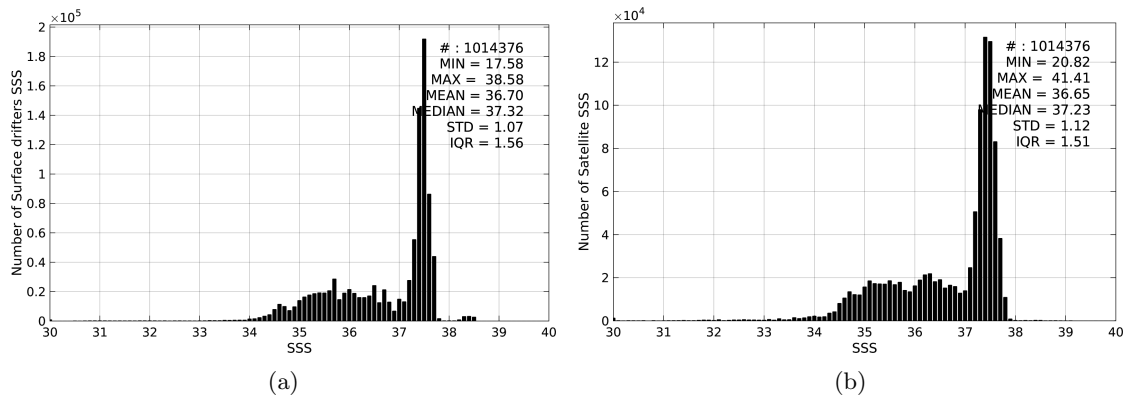
Figure 2: Histograms of SSS from Surface drifters (a) and SMOS-L3-CATDS-CECOS-LOCEAN-V2-18DAYS-25KM (b) considering all match-up pairs per bins of 0.1 over the Global Ocean Pi-MEP region and for the full satellite product period.
