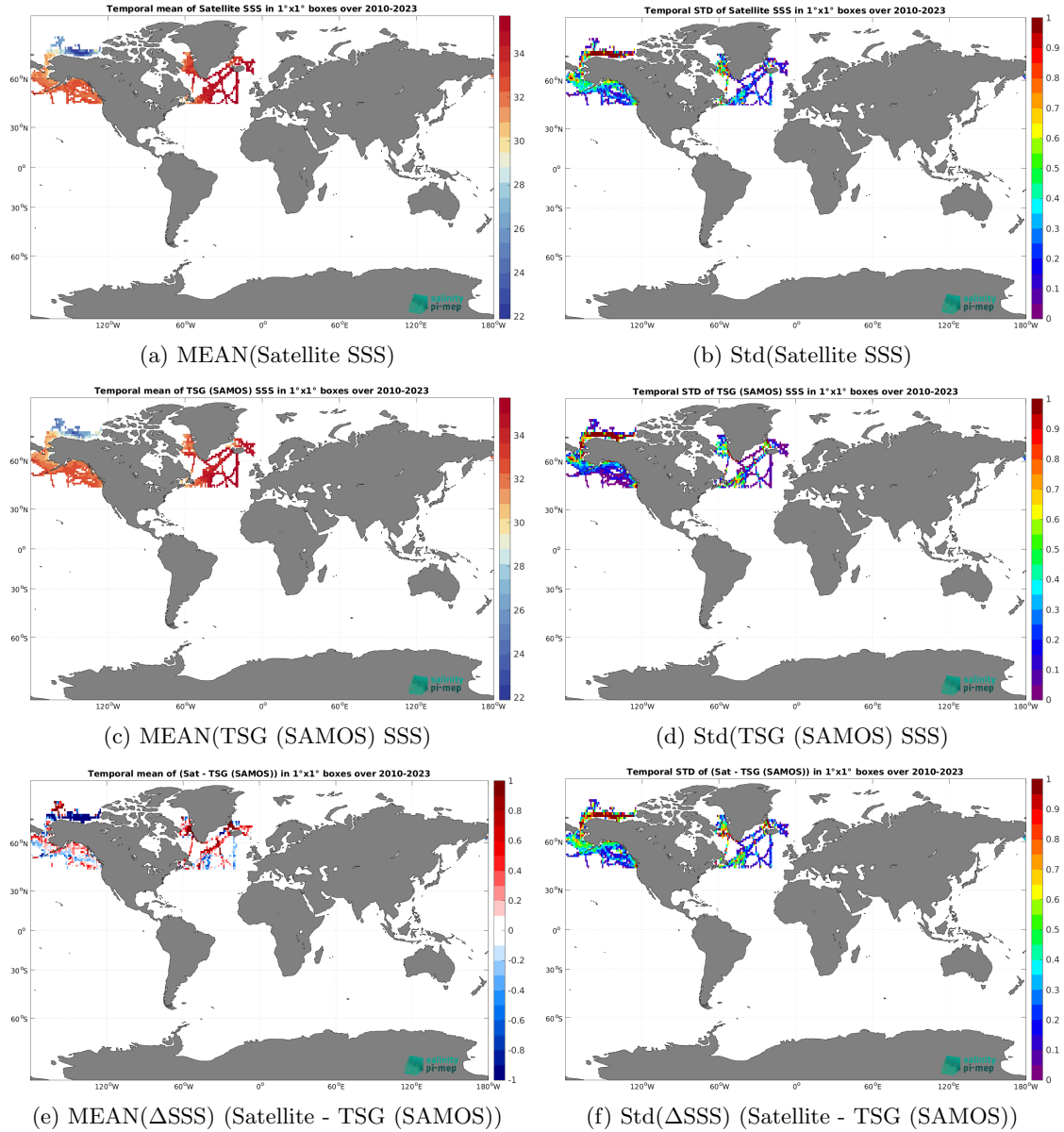
Figure 7: Temporal mean (left) and Std (right) of SSS from SMOS SSS L3 Arctic v2 - 9 Days (CATDS-CEC-LOCEAN) (top), TSG (SAMOS) (middle), and of \Delta SSS (Satellite - TSG (SAMOS)). Only match-up pairs are used to generate these maps.
