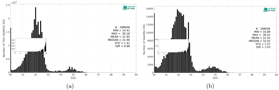
Figure 3: Histograms of SSS from TSG (SAMOS) (a) and SMOS SSS L3 Arctic v2 - 9 Days (CATDS-CEC-LOCEAN) (b) considering all match-up pairs per bins of 0.1 over the Global Ocean Pi-MEP region and for the full satellite product period.
