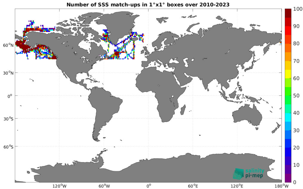
Figure 5: Number of SSS match-ups between TSG (SAMOS) SSS and the SMOS SSS L3 Arctic v2 - 9 Days (CATDS-CEC-LOCEAN) SSS product for the Global Ocean Pi-MEP region over 1^\circ \times 1^\circ boxes and for the full satellite product period.
