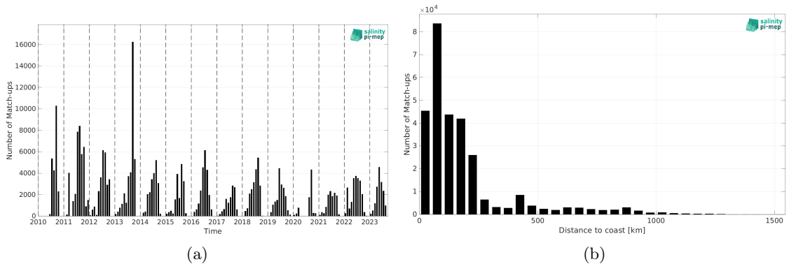
Figure 2: Number of match-ups between TSG (SAMOS) and SMOS SSS L3 Arctic v2 - 9 Days (CATDS-CEC-LOCEAN) SSS as a function of time (a) and as function of the distance to coast (b) over the Global Ocean Pi-MEP region and for the full satellite product period.
