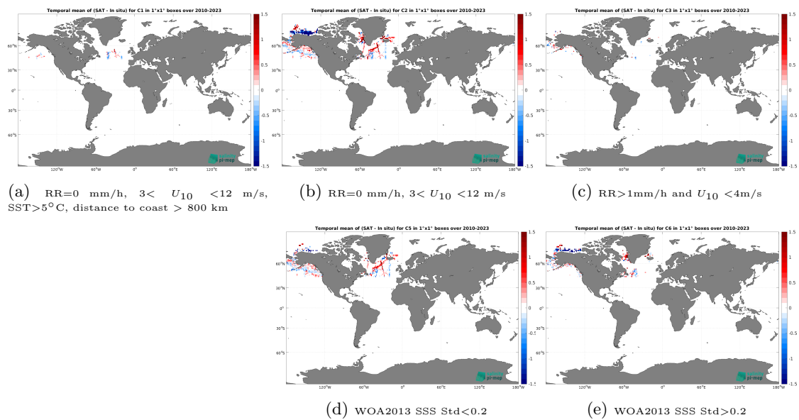
Figure 14: Temporal mean gridded over spatial boxes of size 1^\circ \times 1^\circ of \Delta SSS (SMOS SSS L3 Arctic v2 - 9 Days (CATDS-CEC-LOCEAN) - TSG (SAMOS)) for 5 different subdatasets corresponding to:RR=0 mm/h, 3 < U_{10} < 12 m/s, SST > 5^\circ C, distance to coast > 800 km (a), RR=0 mm/h, 3 < U_{10} < 12 m/s (b), RR > 1 mm/h and U_{10} < 4 m/s (c), WOA2013 SSS Std < 0.2 (d), WOA2013 SSS Std > 0.2 (e).
