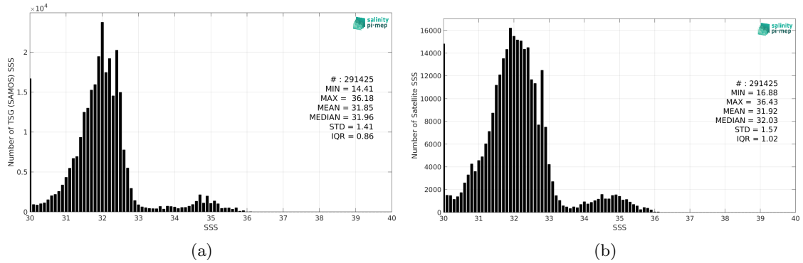
Figure 2: Histograms of SSS from TSG (SAMOS) (a) and SMOS SSS L3 Arctic v2 - 9 Days (CATDS-CEC-LOCEAN) (b) considering all match-up pairs per bins of 0.1 over the Global Ocean Pi-MEP region and for the full satellite product period.
