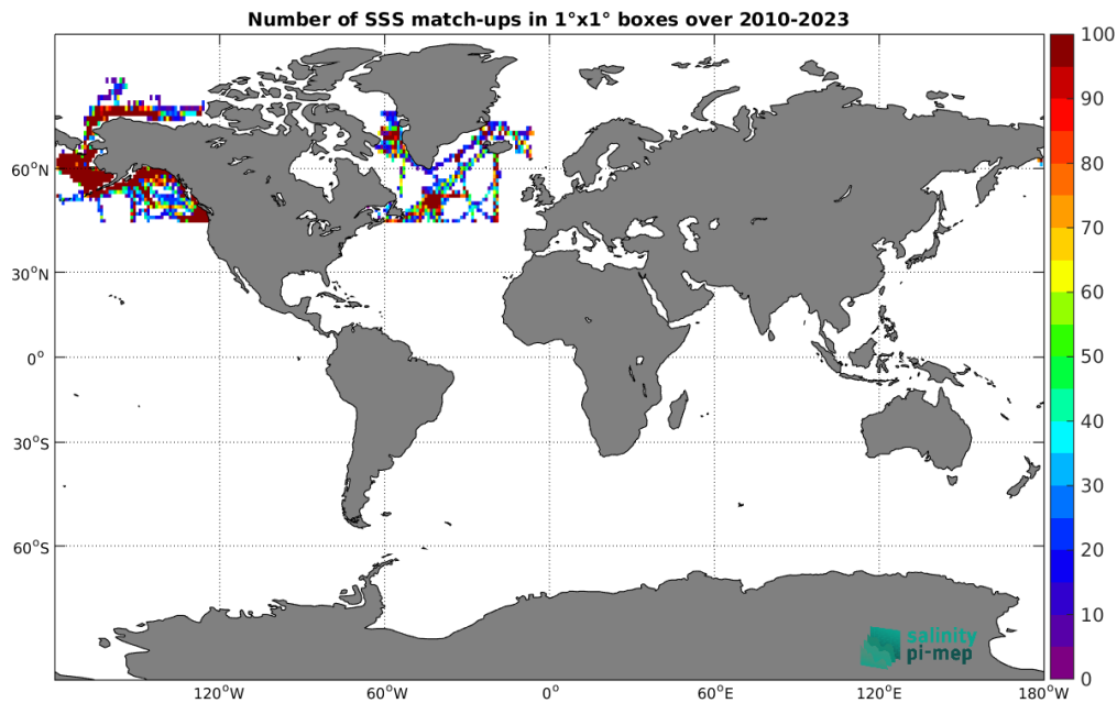
Figure 4: Number of SSS match-ups between TSG (SAMOS) SSS and the SMOS SSS L3 Arctic v2 - 9 Days (CATDS-CEC-LOCEAN) SSS product for the Global Ocean Pi-MEP region over 1^\circ \times 1^\circ boxes and for the full satellite product period.
