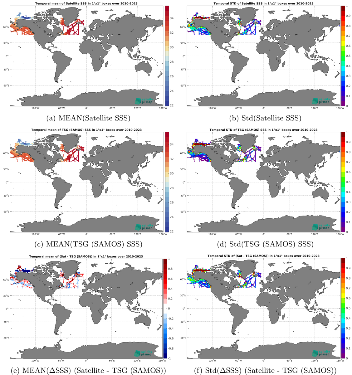
Figure 6: Temporal mean (left) and Std (right) of SSS from SMOS SSS L3 Arctic v2 - 9 Days (CATDS-CEC-LOCEAN) (top), TSG (SAMOS) (middle), and of \Delta SSS (Satellite - TSG (SAMOS)). Only match-up pairs are used to generate these maps.
