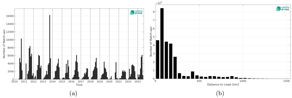
Figure 1: Number of match-ups between TSG (SAMOS) and SMOS SSS L3 Arctic v2 - 9 Days (CATDS-CEC-LOCEAN) SSS as a function of time (a) and as function of the distance to coast (b) over the Global Ocean Pi-MEP region and for the full satellite product period.
