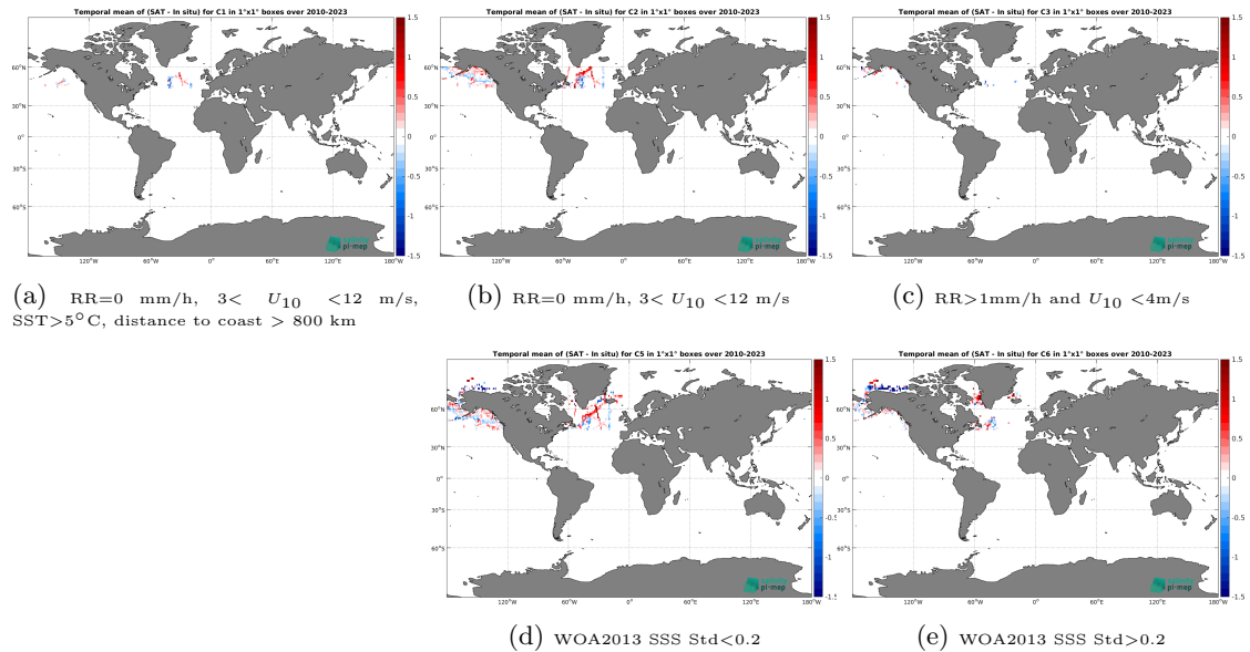
Figure 12: Temporal mean gridded over spatial boxes of size 1^{\circ}\times 1^{\circ} of \Delta\text{SSS} (SMOS SSS L3 Arctic v2 - 9 Days (CATDS-CEC-LOCEAN) - TSG (SAMOS)) for 5 different subdatasets corresponding to:RR=0 mm/h, 3 < U_{10} < 12 m/s, SST >5^{\circ}\text{C} , distance to coast > 800 km (a), RR=0 mm/h, 3 < U_{10} < 12 m/s (b), RR >1 mm/h and U_{10} < 4 m/s (c), WOA2013 SSS Std <0.2 (d), WOA2013 SSS Std >0.2 (e).
