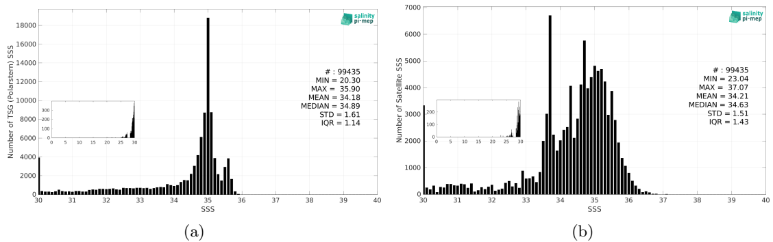
Figure 3: Histograms of SSS from TSG (Polarstern) (a) and SMOS SSS L3 Arctic v2 - 9 Days (CATDS-CEC-LOCEAN) (b) considering all match-up pairs per bins of 0.1 over the Global Ocean Pi-MEP region and for the full satellite product period.
