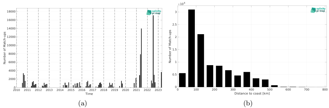
Figure 2: Number of match-ups between TSG (Polarstern) and SMOS SSS L3 Arctic v2 - 9 Days (CATDS-CEC-LOCEAN) SSS as a function of time (a) and as function of the distance to coast (b) over the Global Ocean Pi-MEP region and for the full satellite product period.
