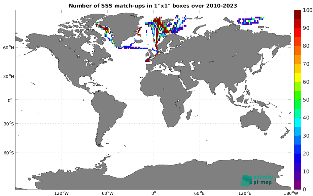
Figure 5: Number of SSS match-ups between TSG (Polarstern) SSS and the SMOS SSS L3 Arctic v2 - 9 Days (CATDS-CEC-LOCEAN) SSS product for the Global Ocean Pi-MEP region over 1^\circ \times 1^\circ boxes and for the full satellite product period.
