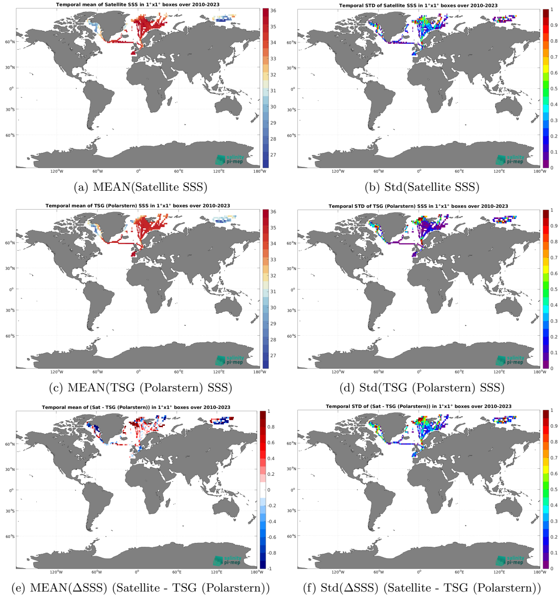
Figure 7: Temporal mean (left) and Std (right) of SSS from SMOS SSS L3 Arctic v2 - 9 Days (CATDS-CEC-LOCEAN) (top), TSG (Polarstern) (middle), and of \Delta SSS (Satellite - TSG (Polarstern)). Only match-up pairs are used to generate these maps.
