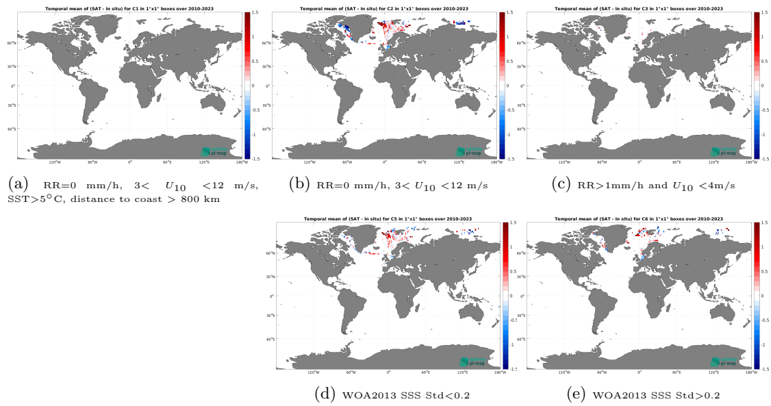
Figure 14: Temporal mean gridded over spatial boxes of size 1^\circ \times 1^\circ of \Delta SSS (SMOS SSS L3 Arctic v2 - 9 Days (CATDS-CEC-LOCEAN) - TSG (Polarstern)) for 5 different subdatasets corresponding to: RR=0 mm/h, 3 < U_{10} < 12 m/s, SST > 5^\circ\text{C} , distance to coast > 800 km (a), RR=0 mm/h, 3 < U_{10} < 12 m/s (b), RR > 1 mm/h and U_{10} < 4 m/s (c), WOA2013 SSS Std < 0.2 (d), WOA2013 SSS Std > 0.2 (e).
