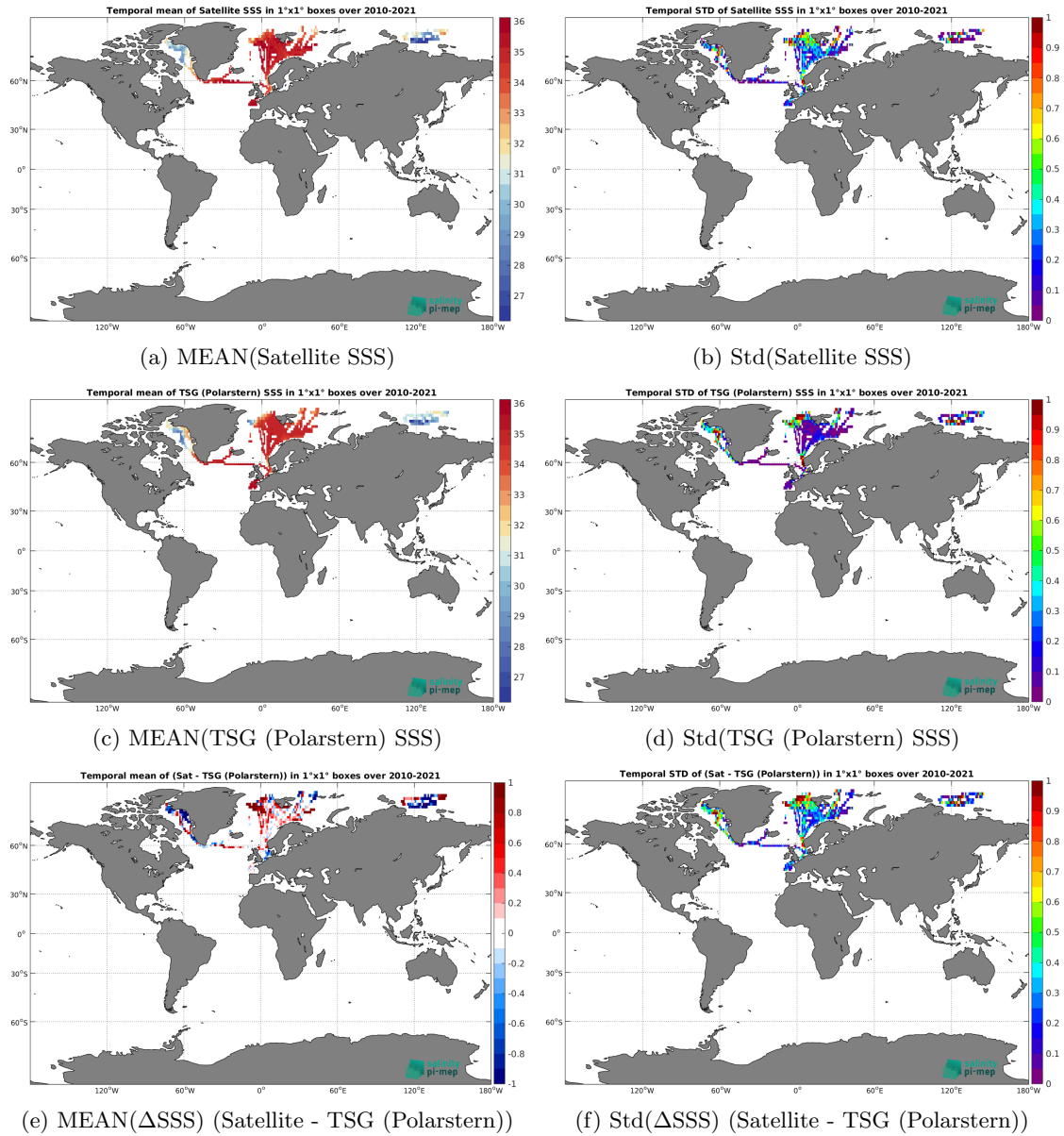
Figure 6: Temporal mean (left) and Std (right) of SSS from SMOS SSS L3 Arctic v2 - 9 Days (CATDS-CEC-LOCEAN) (top), TSG (Polarstern) (middle), and of \Delta SSS (Satellite - TSG (Polarstern)). Only match-up pairs are used to generate these maps.
