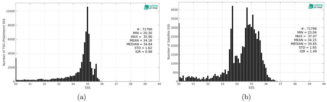
Figure 2: Histograms of SSS from TSG (Polarstern) (a) and SMOS SSS L3 Arctic v2 - 9 Days (CATDS-CEC-LOCEAN) (b) considering all match-up pairs per bins of 0.1 over the Global Ocean Pi-MEP region and for the full satellite product period.
