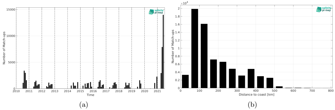
Figure 1: Number of match-ups between TSG (Polarstern) and SMOS SSS L3 Arctic v2 - 9 Days (CATDS-CEC-LOCEAN) SSS as a function of time (a) and as function of the distance to coast (b) over the Global Ocean Pi-MEP region and for the full satellite product period.
