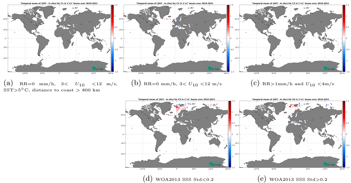
Figure 12: Temporal mean gridded over spatial boxes of size 1^{\circ}\times 1^{\circ} of \Delta\text{SSS} (SMOS SSS L3 Arctic v2 - 9 Days (CATDS-CEC-LOCEAN) - TSG (Polarstern)) for 5 different subdatasets corresponding to:RR=0 mm/h, 3 < U_{10} < 12 m/s, SST >5^{\circ}\text{C} , distance to coast > 800 km (a), RR=0 mm/h, 3 < U_{10} < 12 m/s (b), RR >1 mm/h and U_{10} < 4 m/s (c), WOA2013 SSS Std <0.2 (d), WOA2013 SSS Std >0.2 (e).
