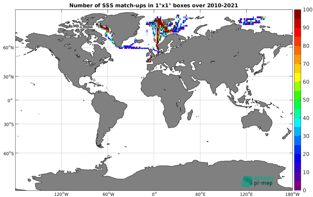
Figure 4: Number of SSS match-ups between TSG (Polarstern) SSS and the SMOS SSS L3 Arctic v2 - 9 Days (CATDS-CEC-LOCEAN) SSS product for the Global Ocean Pi-MEP region over 1^\circ \times 1^\circ boxes and for the full satellite product period.
