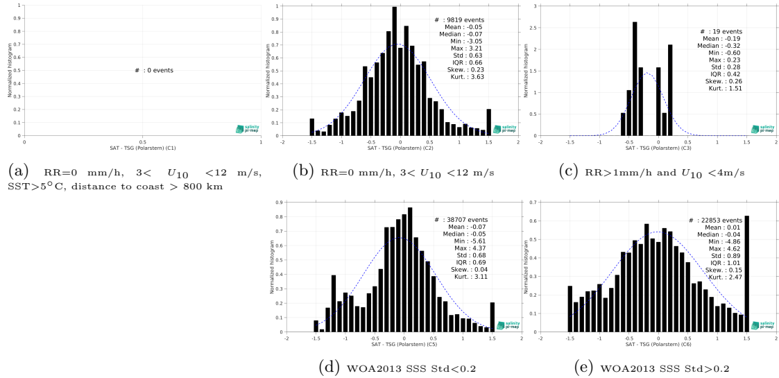
Figure 13: Normalized histogram of \Delta SSS (SMOS SSS L3 Arctic v2 - 9 Days (CATDS-CEC-LOCEAN) - TSG (Polarstern)) for 5 different subdatasets corresponding to: RR=0 mm/h, 3 < U_{10} < 12 m/s, SST > 5^\circ C , distance to coast > 800 km (a), RR=0 mm/h, 3 < U_{10} < 12 m/s (b), RR > 1 mm/h and U_{10} < 4 m/s (c), WOA2013 SSS Std < 0.2 (d), WOA2013 SSS Std > 0.2 (e).
