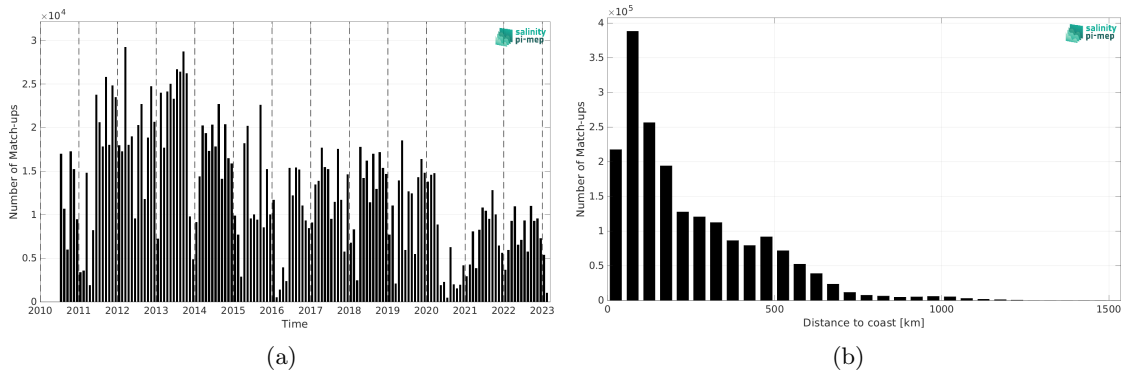
Figure 2: Number of match-ups between TSG (LEGOS-DM) and SMOS SSS L3 Arctic v2 - 9 Days (CATDS-CEC-LOCEAN) SSS as a function of time (a) and as function of the distance to coast (b) over the Global Ocean Pi-MEP region and for the full satellite product period.
