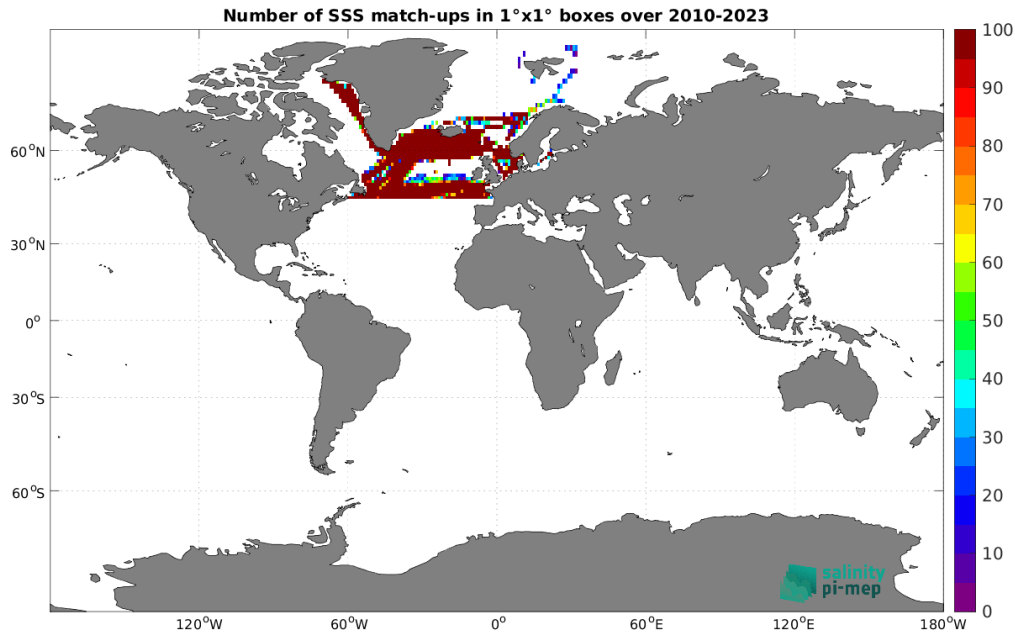
Figure 5: Number of SSS match-ups between TSG (LEGOS-DM) SSS and the SMOS SSS L3 Arctic v2 - 9 Days (CATDS-CEC-LOCEAN) SSS product for the Global Ocean Pi-MEP region over 1^\circ \times 1^\circ boxes and for the full satellite product period.
