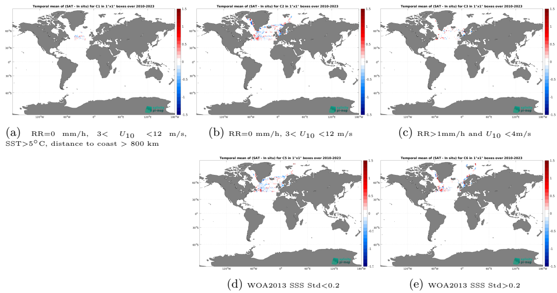
Figure 14: Temporal mean gridded over spatial boxes of size 1^\circ \times 1^\circ of \Delta SSS (SMOS SSS L3 Arctic v2 - 9 Days (CATDS-CEC-LOCEAN) - TSG (LEGOS-DM)) for 5 different subdatasets corresponding to:RR=0 mm/h, 3 < U_{10} < 12 m/s, SST > 5^\circ\text{C} , distance to coast > 800 km (a), RR=0 mm/h, 3 < U_{10} < 12 m/s (b), RR > 1 mm/h and U_{10} < 4 m/s (c), WOA2013 SSS Std < 0.2 (d), WOA2013 SSS Std > 0.2 (e).
