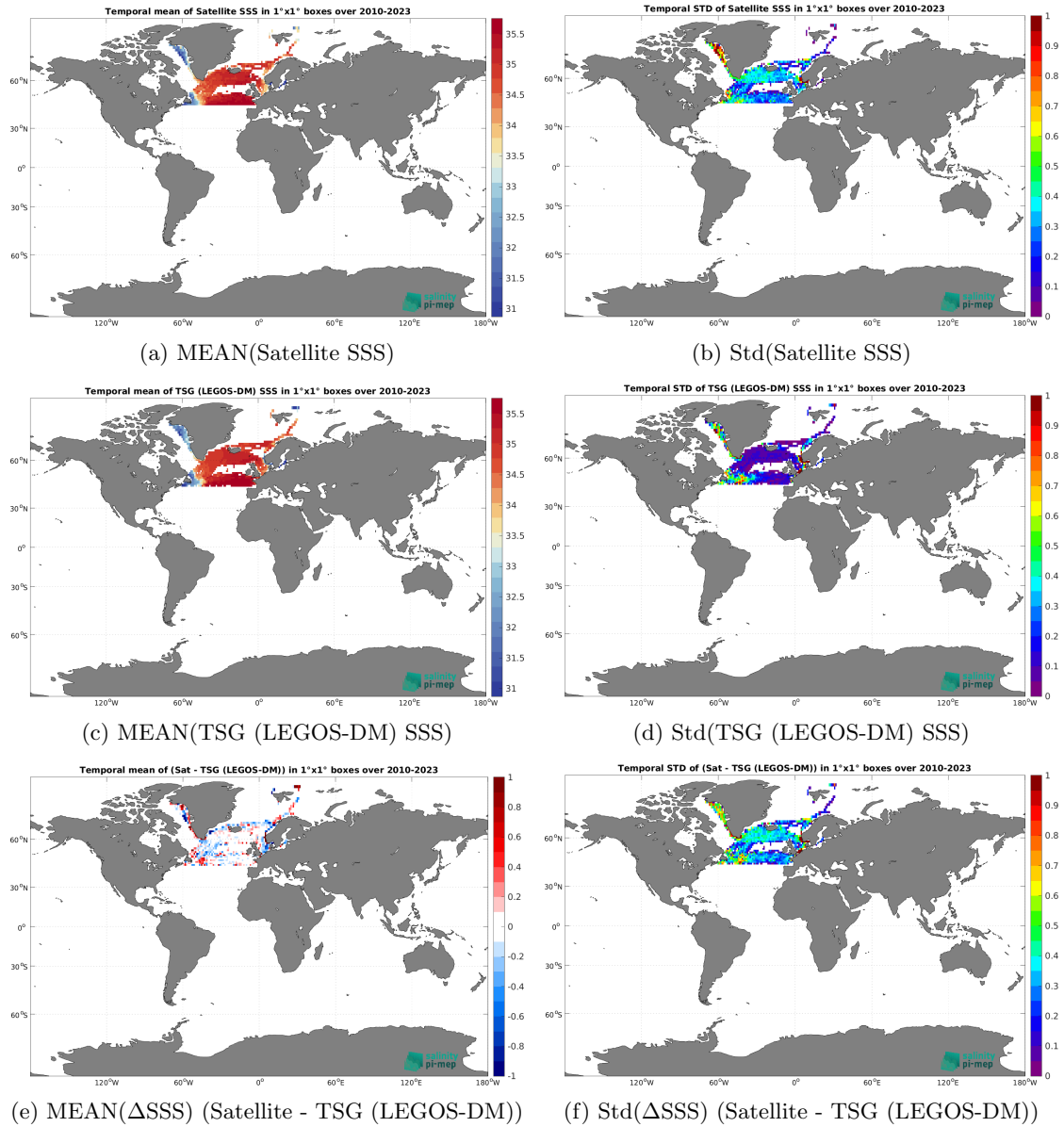
Figure 7: Temporal mean (left) and Std (right) of SSS from SMOS SSS L3 Arctic v2 - 9 Days (CATDS-CEC-LOCEAN) (top), TSG (LEGOS-DM) (middle), and of \Delta SSS (Satellite - TSG (LEGOS-DM)). Only match-up pairs are used to generate these maps.
