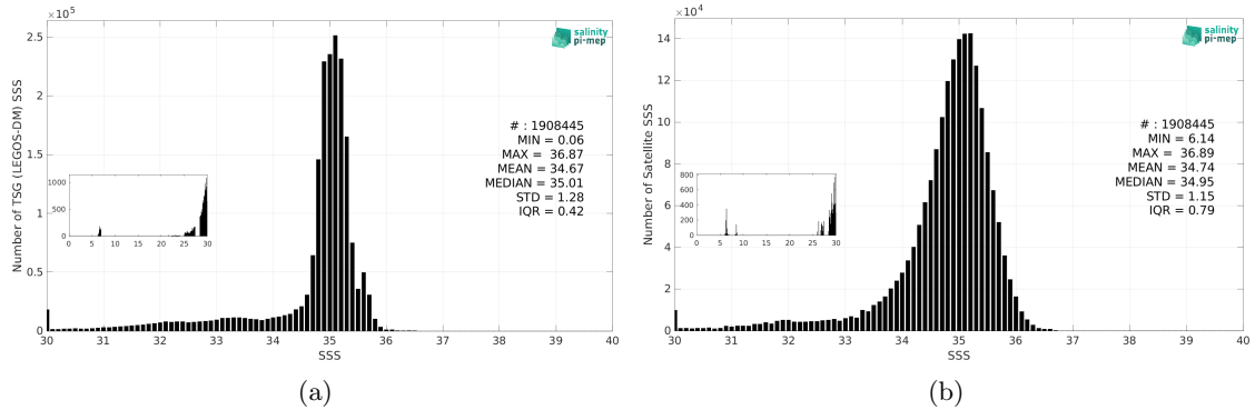
Figure 3: Histograms of SSS from TSG (LEGOS-DM) (a) and SMOS SSS L3 Arctic v2 - 9 Days (CATDS-CEC-LOCEAN) (b) considering all match-up pairs per bins of 0.1 over the Global Ocean Pi-MEP region and for the full satellite product period.
