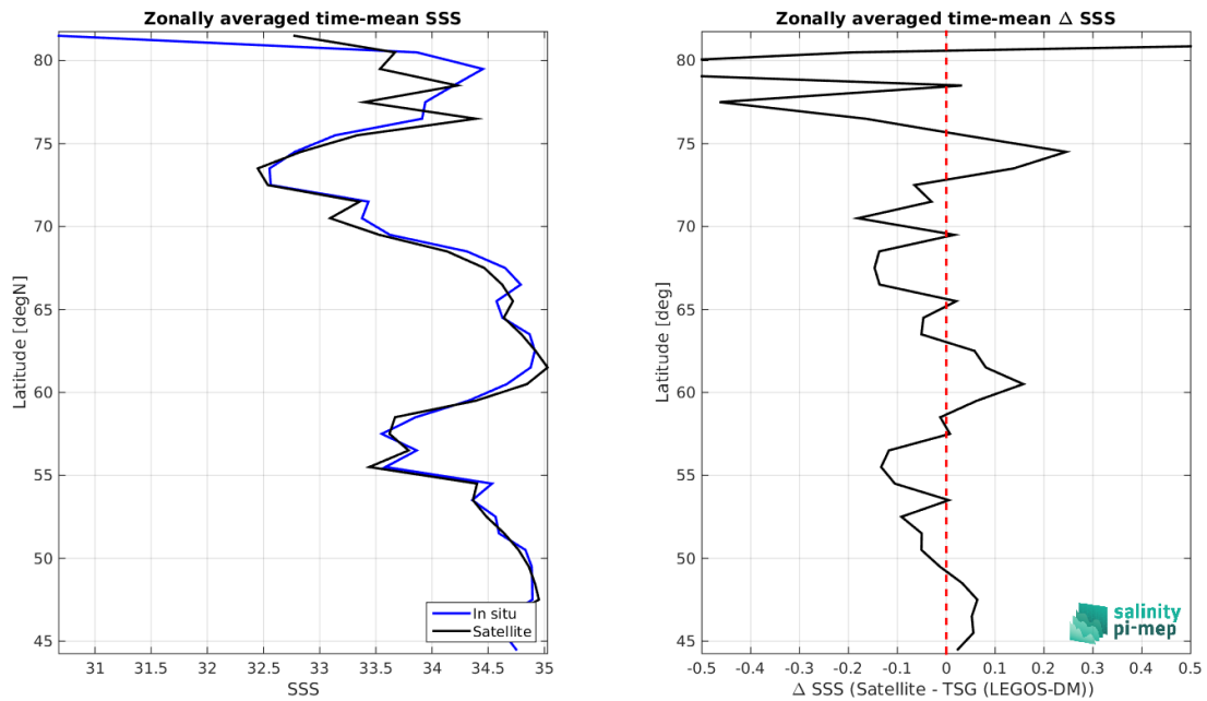
Figure 8: Left panel: Zonal mean SSS from SMOS SSS L3 Arctic v2 - 9 Days (CATDS-CEC-LOCEAN) satellite product (black) and from TSG (LEGOS-DM) (blue). Right panel: Zonal mean of \Delta SSS (Satellite - TSG (LEGOS-DM)) for all the collected Pi-MEP match-up pairs estimated over the full satellite product period.
