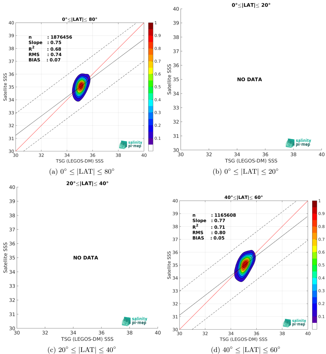
Figure 9: Contour maps of the concentration of SMOS SSS L3 Arctic v2 - 9 Days (CATDS-CEC-LOCEAN) SSS (y-axis) versus TSG (LEGOS-DM) SSS (x-axis) at match-up pairs for different latitude bands. For each plot, the red line shows x=y . The black thin and dashed lines indicate a linear fit through the data cloud and the \pm 95\% confidence levels, respectively. The number match-up pairs n , the slope and R^2 coefficient of the linear fit, the root mean square (RMS) and the mean bias between satellite and in situ data are indicated for each latitude band in each plots.
