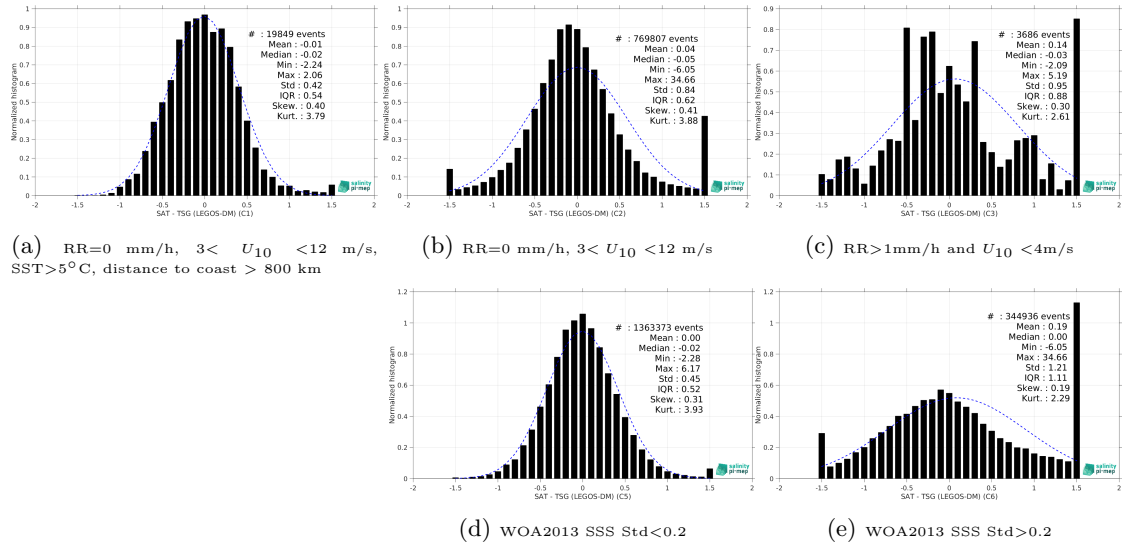
Figure 13: Normalized histogram of \Delta SSS (SMOS SSS L3 Arctic v2 - 9 Days (CATDS-CEC-LOCEAN) - TSG (LEGOS-DM)) for 5 different subdatasets corresponding to: RR=0 mm/h, 3 < U_{10} < 12 m/s, SST>5°C, distance to coast > 800 km (a), RR=0 mm/h, 3 < U_{10} < 12 m/s (b), RR>1mm/h and U_{10} < 4 m/s (c), WOA2013 SSS Std<0.2 (d), WOA2013 SSS Std>0.2 (e).
