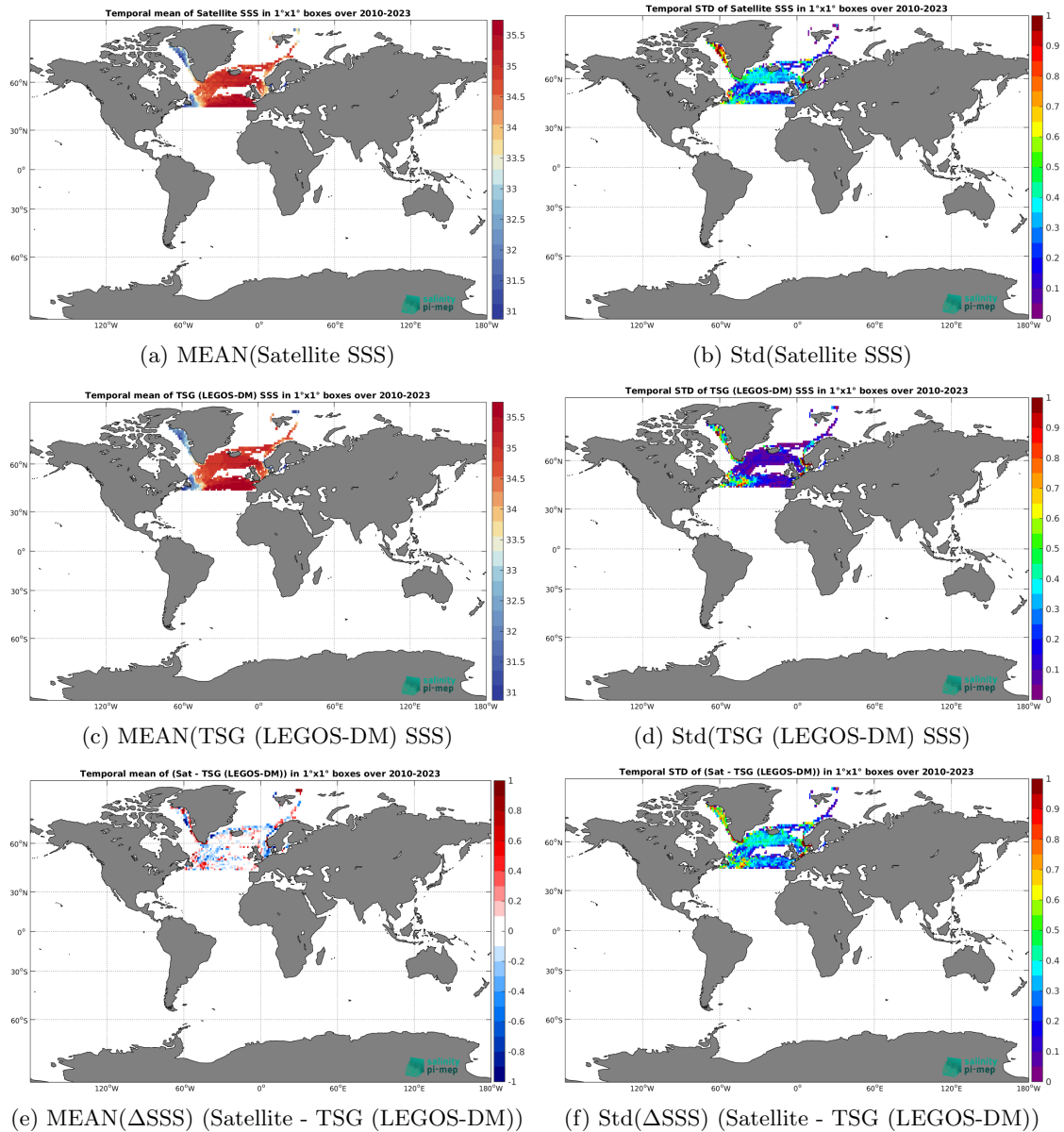
Figure 6: Temporal mean (left) and Std (right) of SSS from SMOS SSS L3 Arctic v2 - 9 Days (CATDS-CEC-LOCEAN) (top), TSG (LEGOS-DM) (middle), and of \Delta SSS (Satellite - TSG (LEGOS-DM)). Only match-up pairs are used to generate these maps.
