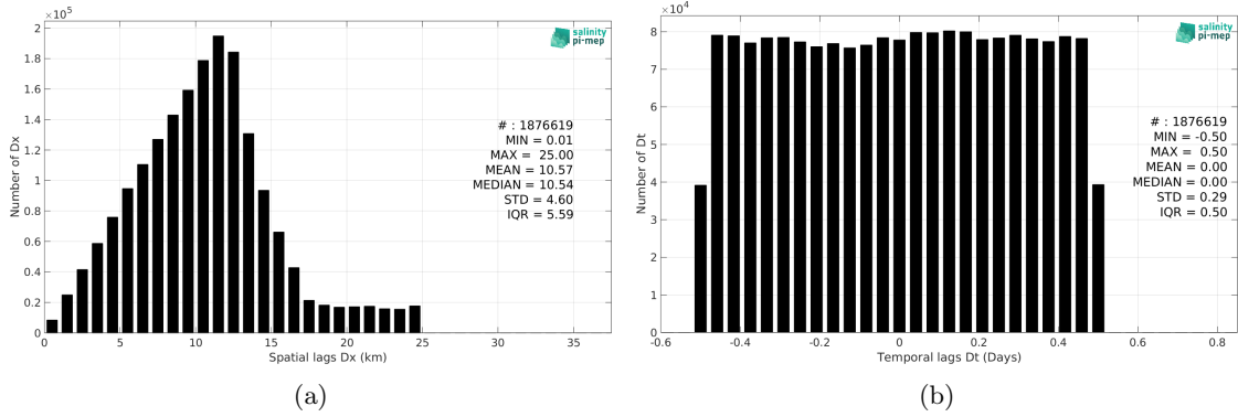
Figure 5: Histograms of the spatial (a) and temporal (b) lags between the location/time of the TSG (LEGOS-DM) measurement and the date of the corresponding SMOS SSS L3 Arctic v2 - 9 Days (CATDS-CEC-LOCEAN) SSS pixel.
