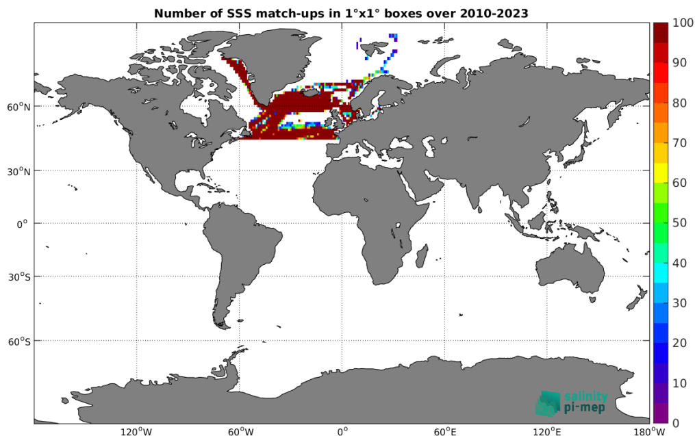
Figure 4: Number of SSS match-ups between TSG (LEGOS-DM) SSS and the SMOS SSS L3 Arctic v2 - 9 Days (CATDS-CEC-LOCEAN) SSS product for the Global Ocean Pi-MEP region over 1^\circ \times 1^\circ boxes and for the full satellite product period.
