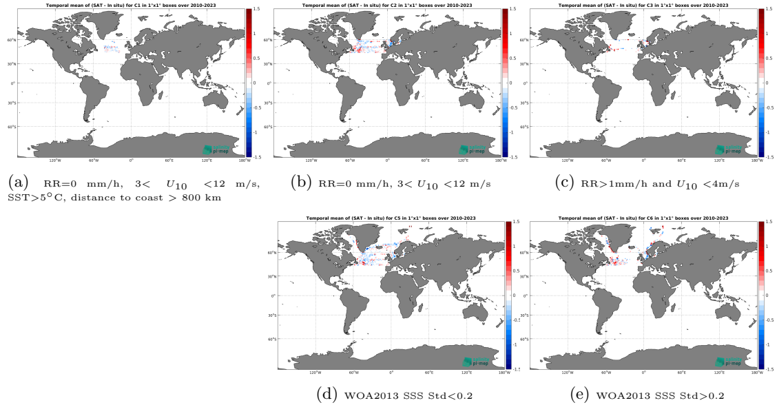
Figure 12: Temporal mean gridded over spatial boxes of size 1^{\circ}\times 1^{\circ} of \Delta\text{SSS} (SMOS SSS L3 Arctic v2 - 9 Days (CATDS-CEC-LOCEAN) - TSG (LEGOS-DM)) for 5 different subdatasets corresponding to:RR=0 mm/h, 3 < U_{10} < 12 m/s, SST >5^{\circ}\text{C} , distance to coast > 800 km (a), RR=0 mm/h, 3 < U_{10} < 12 m/s (b), RR >1 mm/h and U_{10} < 4 m/s (c), WOA2013 SSS Std <0.2 (d), WOA2013 SSS Std >0.2 (e).
