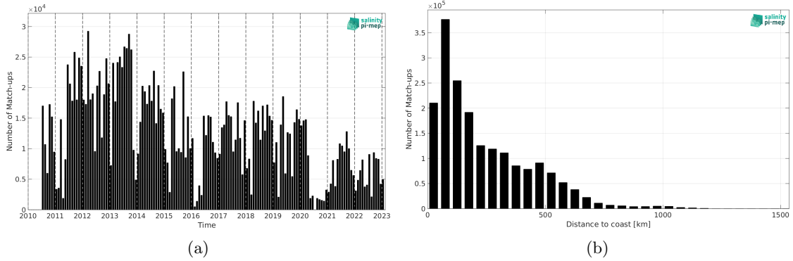
Figure 1: Number of match-ups between TSG (LEGOS-DM) and SMOS SSS L3 Arctic v2 - 9 Days (CATDS-CEC-LOCEAN) SSS as a function of time (a) and as function of the distance to coast (b) over the Global Ocean Pi-MEP region and for the full satellite product period.
