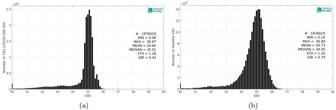
Figure 2: Histograms of SSS from TSG (LEGOS-DM) (a) and SMOS SSS L3 Arctic v2 - 9 Days (CATDS-CEC-LOCEAN) (b) considering all match-up pairs per bins of 0.1 over the Global Ocean Pi-MEP region and for the full satellite product period.
