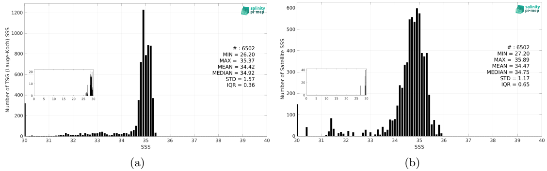
Figure 3: Histograms of SSS from TSG (Lauge-Koch) (a) and SMOS SSS L3 Arctic v2 - 9 Days (CATDS-CEC-LOCEAN) (b) considering all match-up pairs per bins of 0.1 over the Global Ocean Pi-MEP region and for the full satellite product period.
