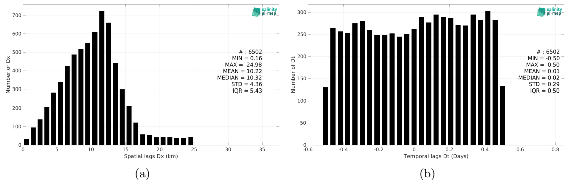
Figure 6: Histograms of the spatial (a) and temporal (b) lags between the location/time of the TSG (Lauge-Koch) measurement and the date of the corresponding SMOS SSS L3 Arctic v2 - 9 Days (CATDS-CEC-LOCEAN) SSS pixel.
