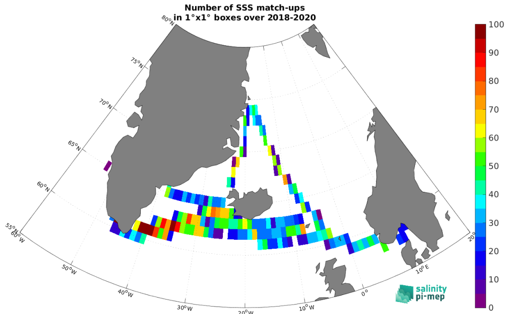
Figure 5: Number of SSS match-ups between TSG (Lauge-Koch) SSS and the SMOS SSS L3 Arctic v2 - 9 Days (CATDS-CEC-LOCEAN) SSS product for the Global Ocean Pi-MEP region over 1^\circ \times 1^\circ boxes and for the full satellite product period.
