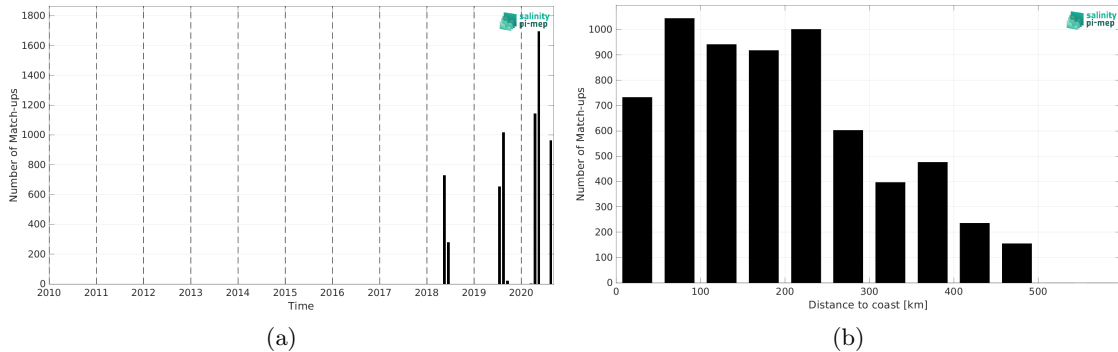
Figure 2: Number of match-ups between TSG (Lauge-Koch) and SMOS SSS L3 Arctic v2 - 9 Days (CATDS-CEC-LOCEAN) SSS as a function of time (a) and as function of the distance to coast (b) over the Global Ocean Pi-MEP region and for the full satellite product period.
